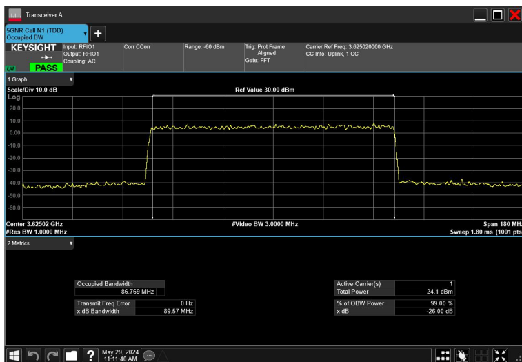
90MHz_30kHz_3625MHz_DFT-s-OFDM 16QAM_RB243@0
