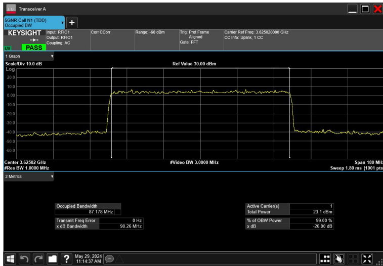
90MHz_30kHz_3625MHz_CP-OFDM 16QAM_RB245@0
