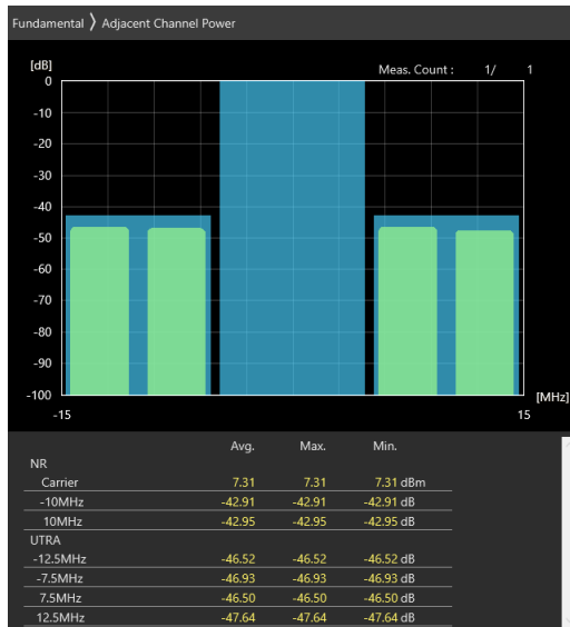
10MHz_30kHz_3695MHz_CP-OFDM 64 QAM_RB1@23 -42.91 dB,-42.95 dB
