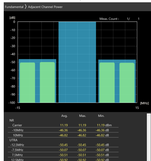
10MHz_15kHz_3695MHz_DFT-s-OFDM QPSK_RB25@12 -46.36 dB,-46.82 dB
