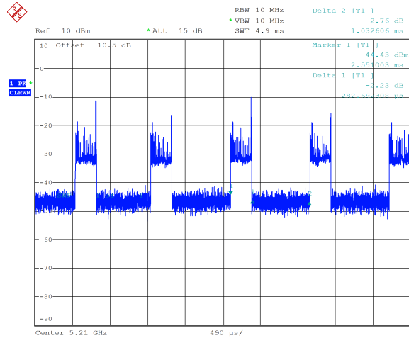
ax80_5210MHz_RU_52/37_Chain 0 0.283 ms,1.033ms
