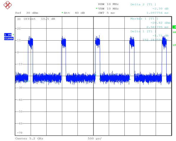
ax20_5200MHz_RU_242/61_Chain 0 0.152 ms,1.098ms
