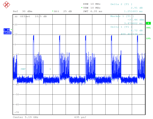
ax40_5190MHz_RU_52/37_Chain 0 0.488 ms,1.252ms
