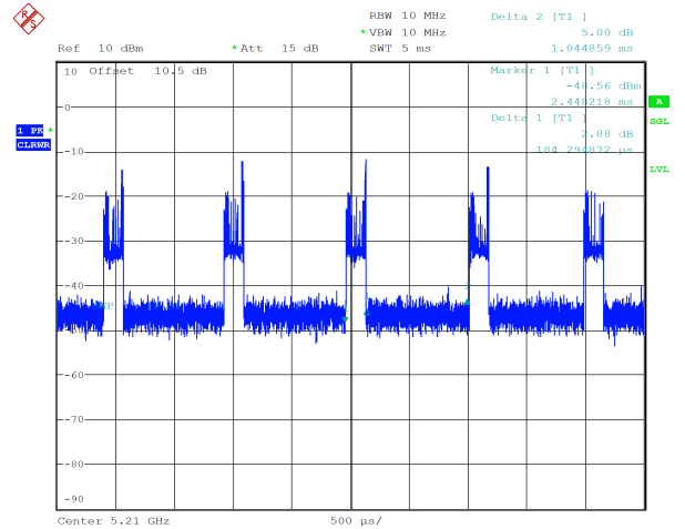
ax80_5210MHz_RU_106/53_Chain 0 0.184 ms,1.045ms
