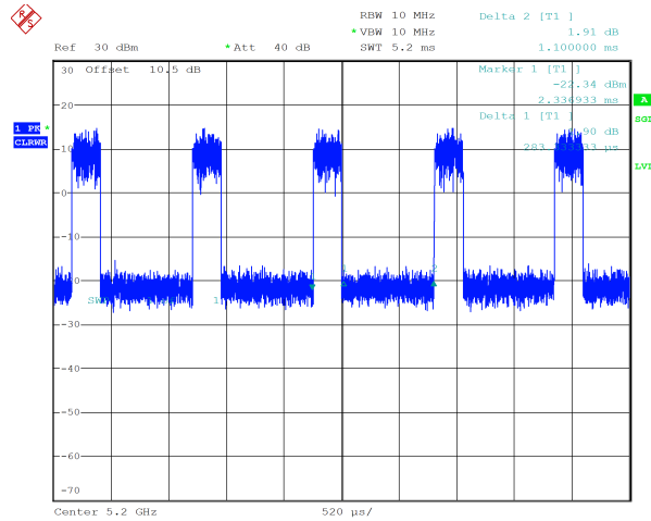
ax20_5200MHz_RU_106/53_Chain 0 0.283 ms,1.1ms
