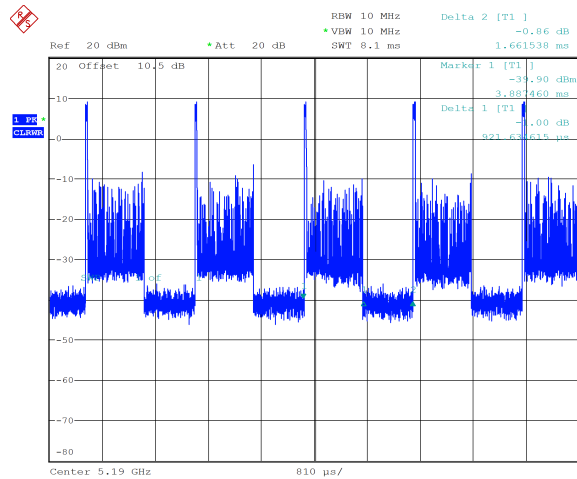
ax40_5190MHz_RU_26/0_Chain 0 0.922 ms,1.662ms
