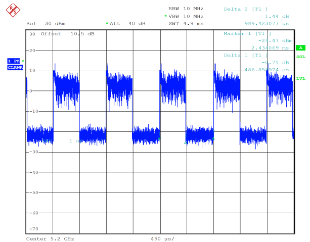
ax20_5200MHz_RU_52/37_Chain 0 0.487 ms,0.989ms
