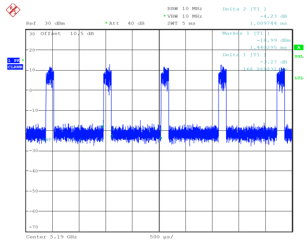
ax40_5190MHz_RU_242/61_Chain 0 0.168 ms,1.09ms
