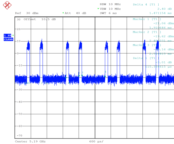
ax40_5190MHz_RU_484/65_Chain 0
