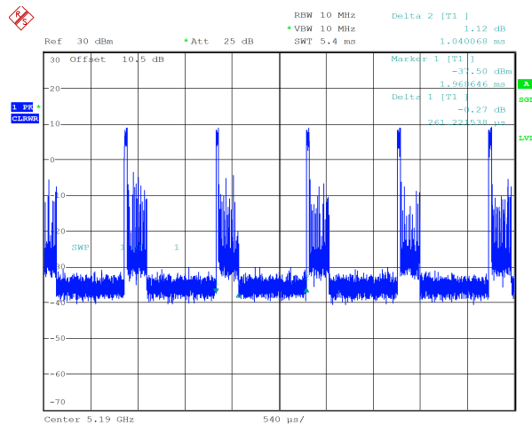
ax40_5190MHz_RU_106/53_Chain 0 0.261 ms,1.04ms
