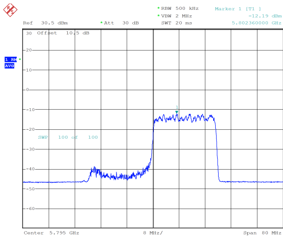
ax40_5795MHz_RU_242/62_Chain 0 -12.19 dBm
