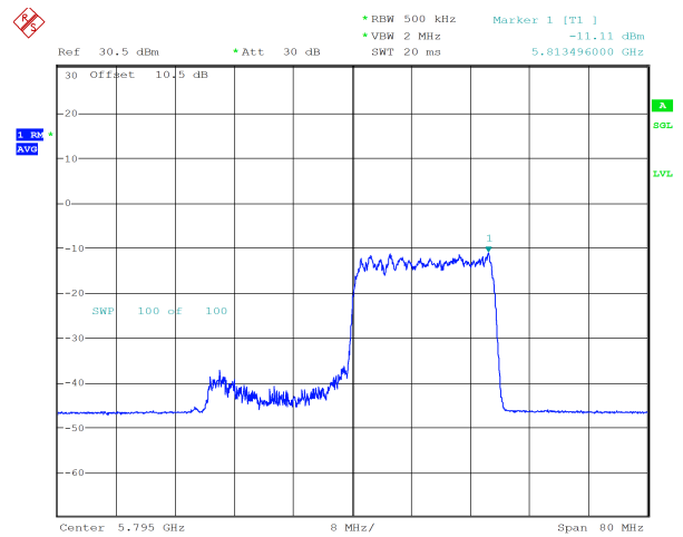
ax40_5795MHz_RU_242/62_Chain 1 -11.11 dBm
