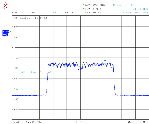
ax40_5795MHz_RU_484/65_Chain 0 -14.07 dBm
