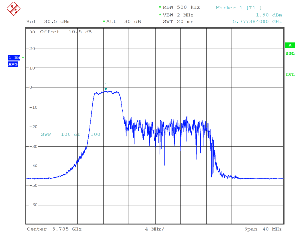
ax20_5785MHz_RU_52/37_Chain 1 -1.90 dBm
