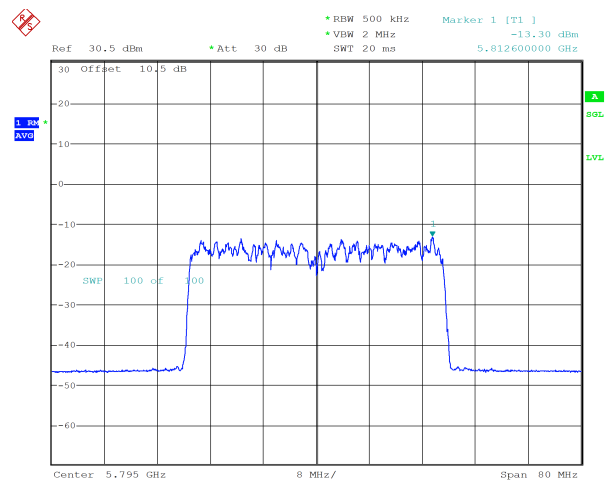
ax40_5795MHz_RU_484/65_Chain 1 -13.30 dBm
