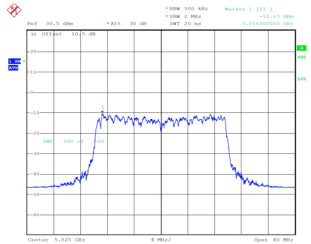
ax20_5825MHz_RU_242/61_Chain 1 -10.63 dBm
