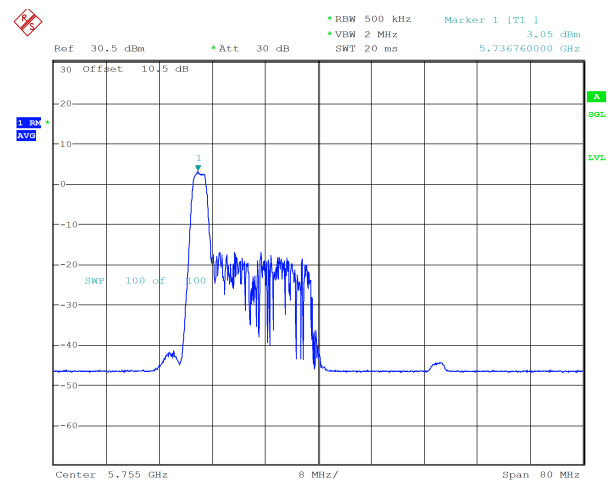
ax40_5755MHz_RU_26/0_Chain 1 3.05 dBm
