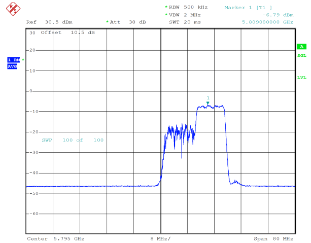
ax40_5795MHz_RU_106/56_Chain 1 -6.79 dBm
