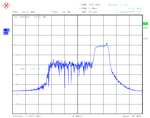
ax20_5825MHz_RU_52/40_Chain 1 0.56 dBm
