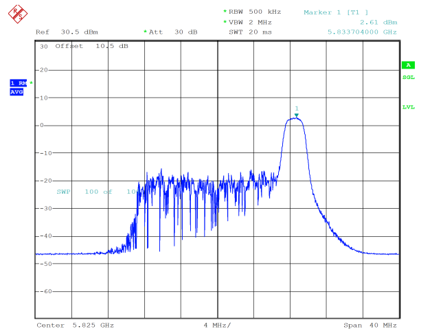
ax20_5825MHz_RU_26/8_Chain 1 2.61 dBm
