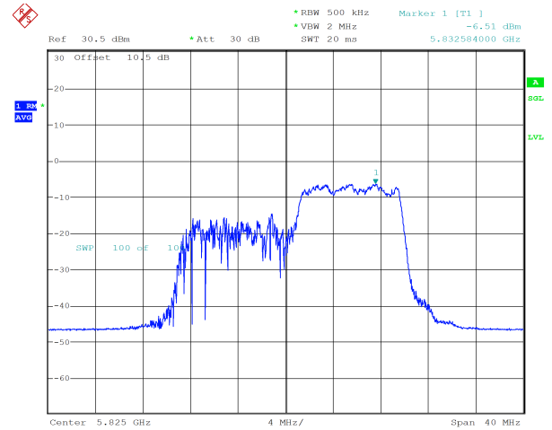
ax20_5825MHz_RU_106/54_Chain 1 -6.51 dBm
