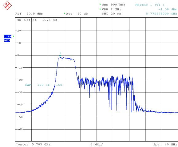
ax20_5785MHz_RU_52/37_Chain 0 -1.58 dBm
