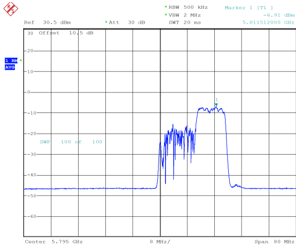
ax40_5795MHz_RU_106/56_Chain 0 -6.91 dBm
