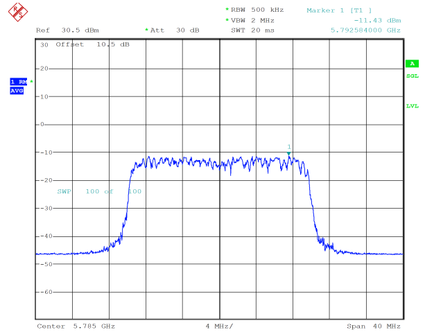
ax20_5785MHz_RU_242/61_Chain 1 -11.43 dBm
