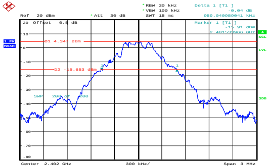
GFSK_Low 0.959MHz
