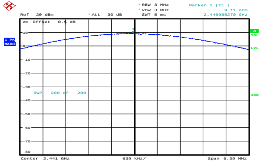
8DPSK_Middle 9.11dBm
