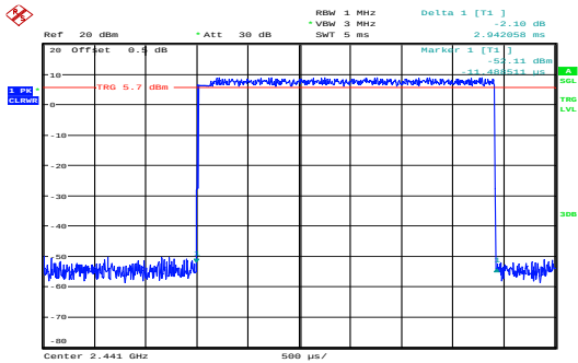
8DPSK_Hopping_3DH5 2.942ms
