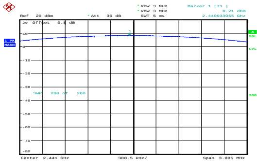
GFSK_Middle 8.21dBm
