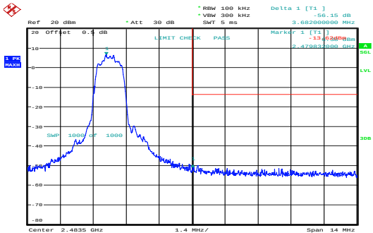
8DPSK_High
