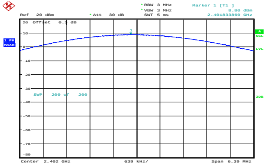
8DPSK_Low 8.80dBm
