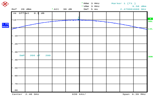
8DPSK_High 9.58dBm
