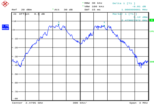
GFSK_High 1.001MHz
