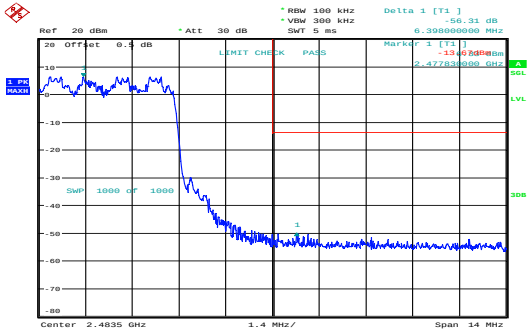
8DPSK_Hopping_Upper
