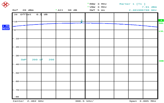
GFSK_Low 7.91dBm
