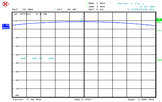
GFSK_High 8.64dBm
