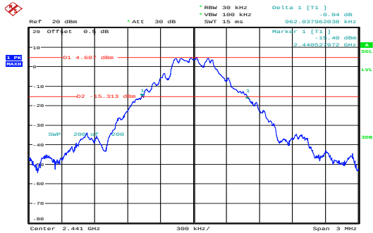
GFSK_Middle 0.962MHz
