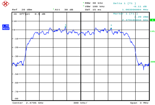
\pi/4 -DQPSK_High 1.004MHz
