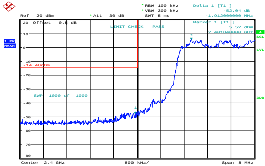
8DPSK_Hopping_Lower
