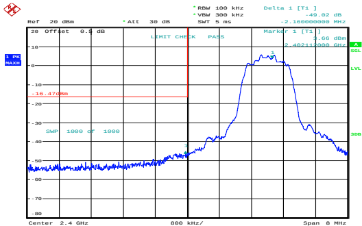
8DPSK_Low
