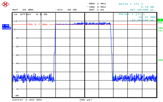
8DPSK_Hopping_3DH1 0.408ms
