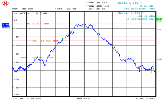
GFSK_High 0.941MHz
