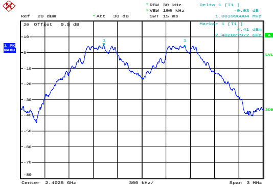
GFSK_Low 1.004MHz
