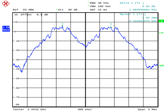
GFSK_Middle 1.004MHz
