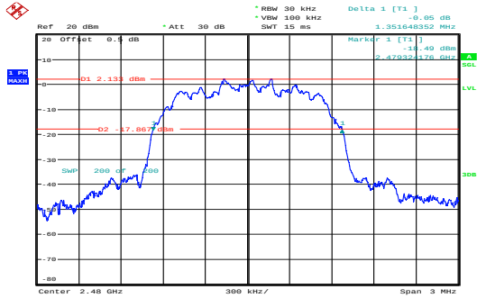
\pi/4 -DQPSK_High 1.352MHz
