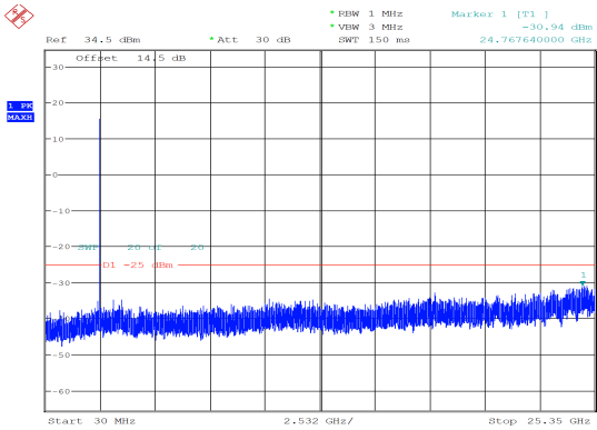
10MHz_Middle_QPSK_1@0 -30.94 dBm
