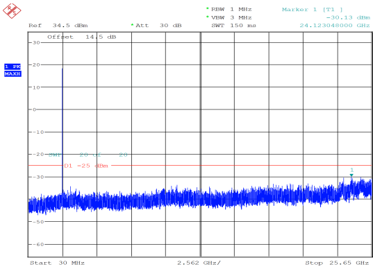
10MHz_High_QPSK_1@0 -30.13 dBm
