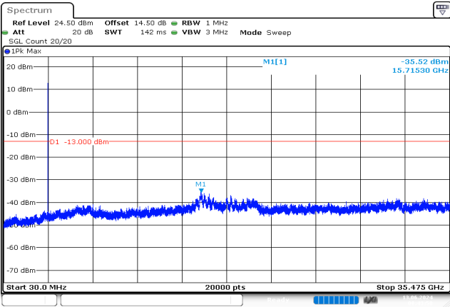
5MHz_High_QPSK_25@0 -35.52 dBm
