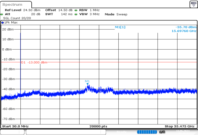
5MHz_High_QPSK_1@0 -35.70 dBm
