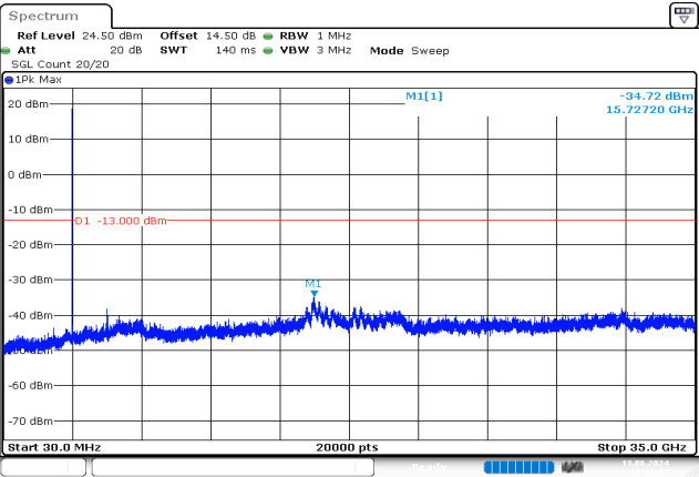
5MHz_Middle_QPSK_1@0 -34.72 dBm
