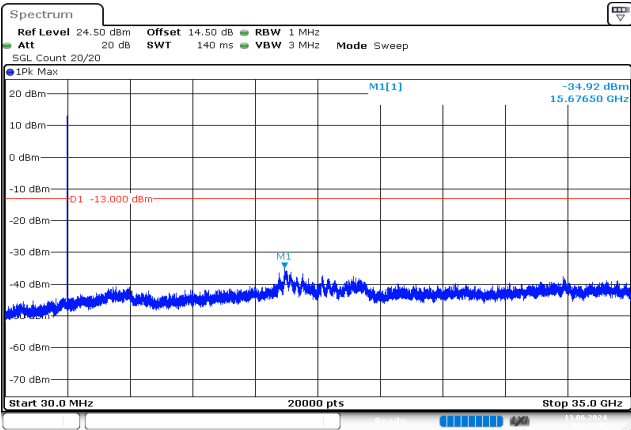
5MHz_Middle_QPSK_25@0 -34.92 dBm
