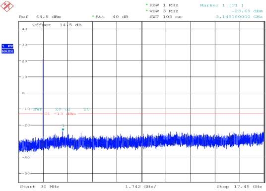
20MHz_High_QPSK_1@0 -23.69 dBm
