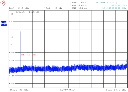
10MHz_High_QPSK_1@0 -22.98 dBm
