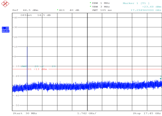
20MHz_High_QPSK_100@0 -23.68 dBm
