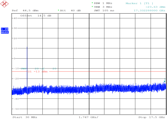
10MHz_High_QPSK_50@0 -23.63 dBm
