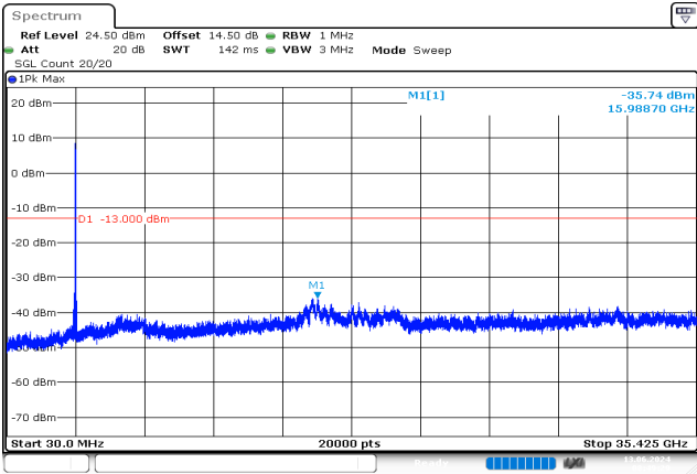
15MHz_High_QPSK_75@0 -35.74 dBm
