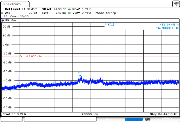
15MHz_High_QPSK_1@0 -35.54 dBm
