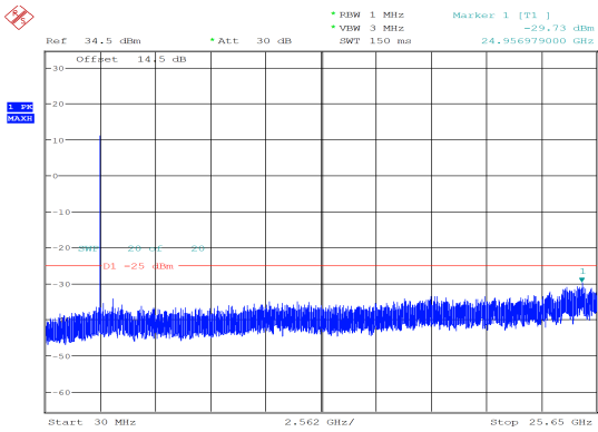
10MHz_High_QPSK_50@0 -29.73 dBm
