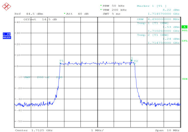
99% Occupied Bandwidth 4.49 MHz
