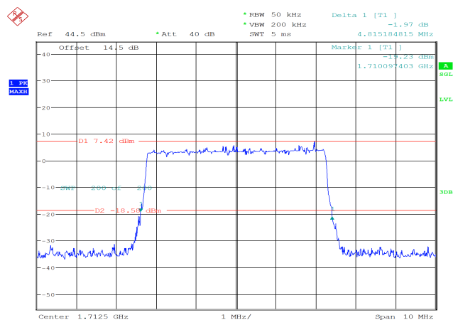
26dB Bandwidth 4.815MHz
