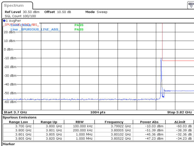
15MHz_30kHz_3792.5MHz_DFT-s-OFDM QPSK_RB1@37 -45.36 dBm
