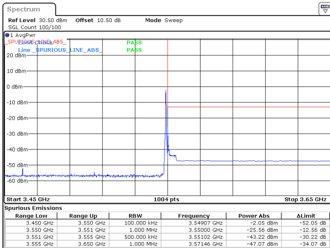
90MHz_30kHz_3505MHz_DFT-s-OFDM QPSK_RB1@244 -25.56 dBm
