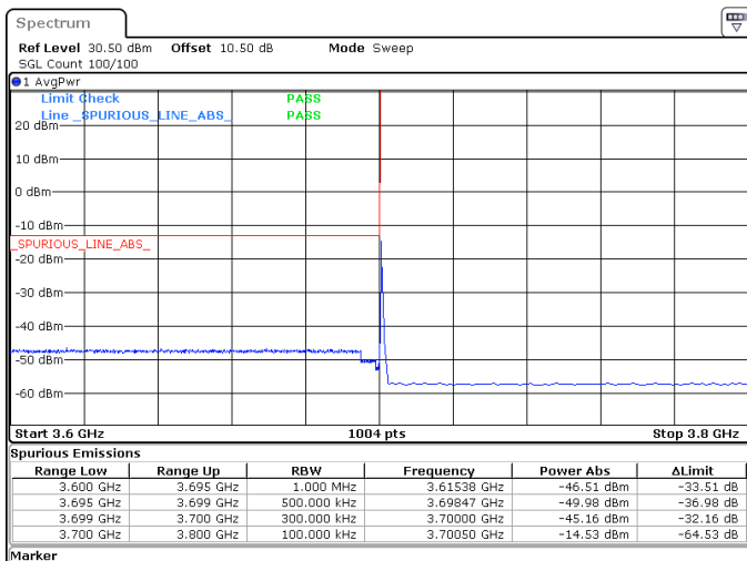
25MHz_15kHz_3712.5MHz_DFT-s-OFDM QPSK_RB1@0 -45.16 dBm
