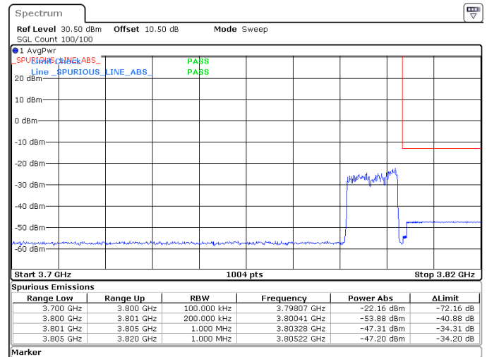
15MHz_30kHz_3792.5MHz_DFT-s-OFDM QPSK_RB36@0 -47.20 dBm
