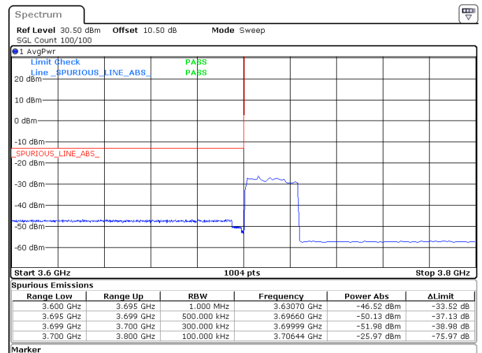
25MHz_15kHz_3712.5MHz_DFT-s-OFDM QPSK_RB128@0 -46.52 dBm
