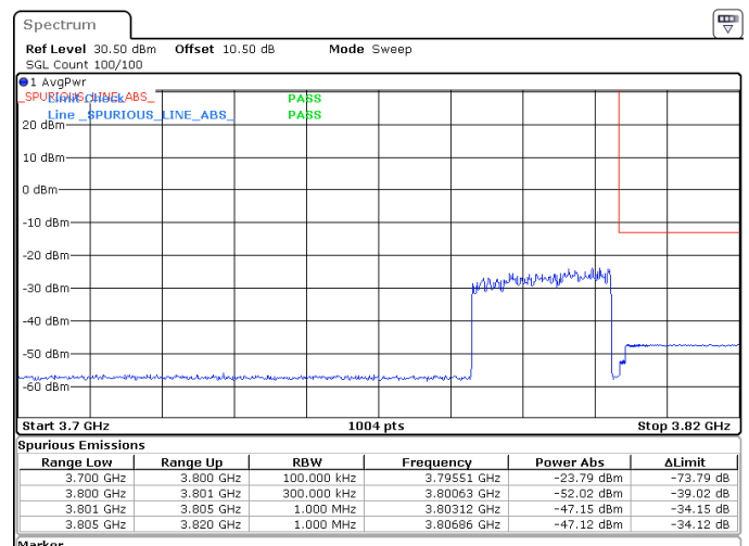
25MHz_15kHz_3787.5MHz_DFT-s-OFDM QPSK_RB128@0 -47.12 dBm
