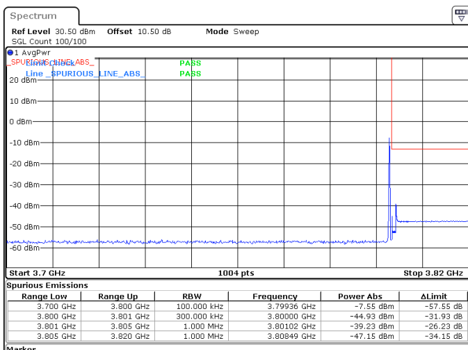
25MHz_15kHz_3787.5MHz_DFT-s-OFDM QPSK_RB1@132 -39.23 dBm
