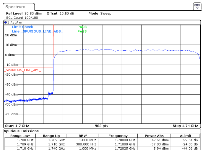
30MHz_15kHz_1725MHz_DFT-s-OFDM QPSK_RB160@0 -37.00 dBm
