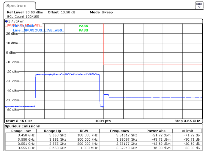
70MHz_30kHz_3515MHz_DFT-s-OFDM QPSK_RB180@0 -43.69 dBm
