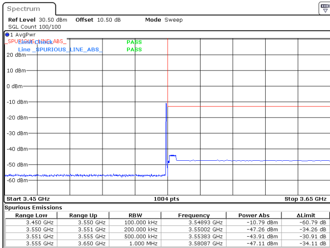
20MHz_30kHz_3540MHz_DFT-s-OFDM QPSK_RB1@50 -43.91 dBm
