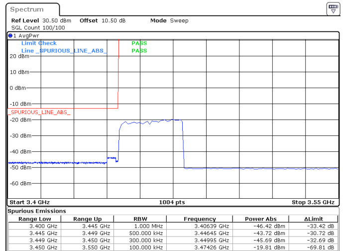
30MHz_15kHz_3465MHz_DFT-s-OFDM QPSK_RB160@0 -43.72 dBm
