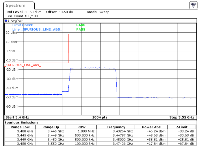
40MHz_30kHz_3470MHz_DFT-s-OFDM QPSK_RB100@0 -38.81 dBm
