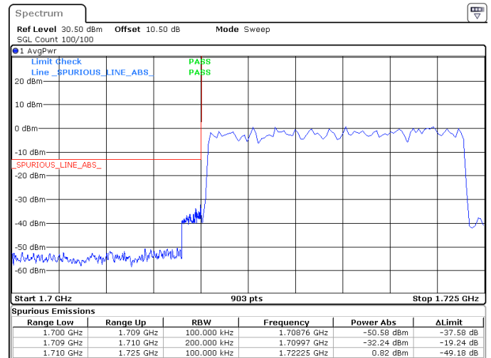
15MHz_15kHz_1717.5MHz_DFT-s-OFDM QPSK_RB75@0 -32.24 dBm
