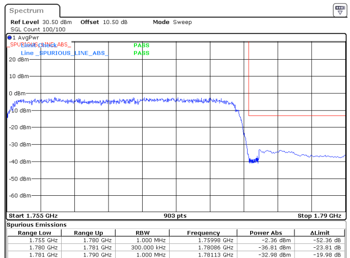
25MHz_15kHz_1767.5MHz_DFT-s-OFDM QPSK_RB128@0 -32.98 dBm
