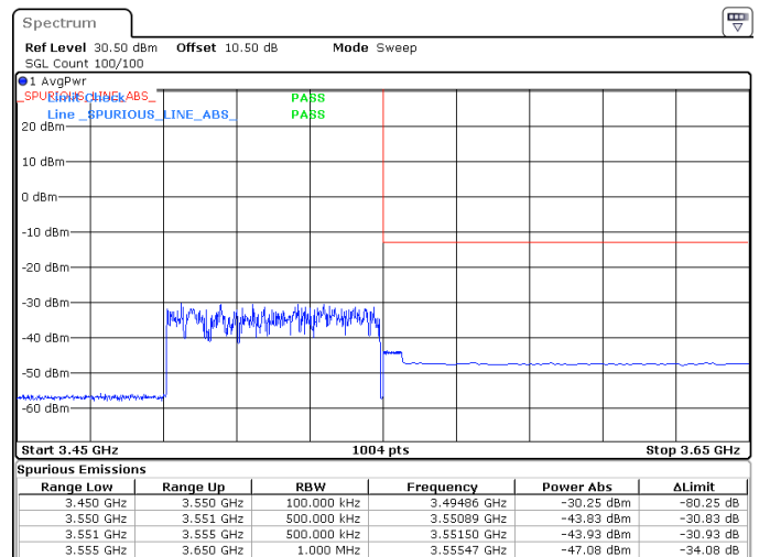
60MHz_30kHz_3520MHz_DFT-s-OFDM QPSK_RB162@0 -43.83 dBm
