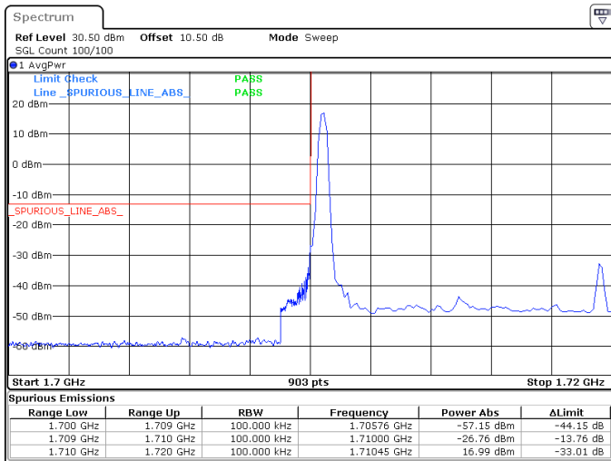
10MHz_15kHz_1715MHz_DFT-s-OFDM QPSK_RB1@0 -26.76 dBm
