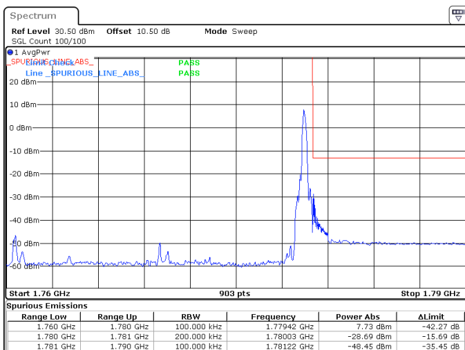
20MHz_15kHz_1770MHz_DFT-s-OFDM QPSK_RB1@105 -28.69 dBm
