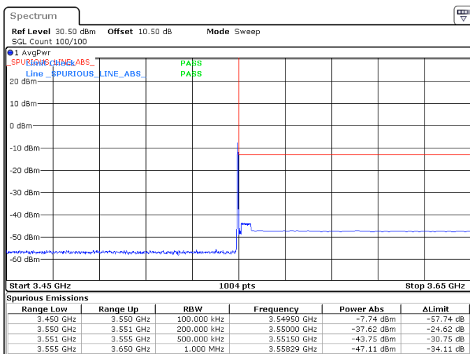
20MHz_15kHz_3540MHz_DFT-s-OFDM QPSK_RB1@105 -37.62 dBm
