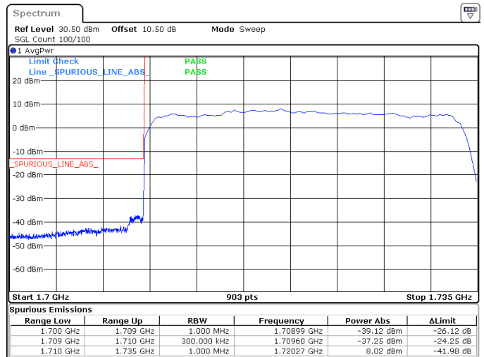
25MHz_15kHz_1722.5MHz_DFT-s-OFDM QPSK_RB128@0 -37.25 dBm
