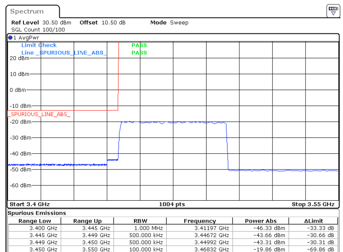
50MHz_15kHz_3475MHz_DFT-s-OFDM QPSK_RB270@0 -43.31 dBm
