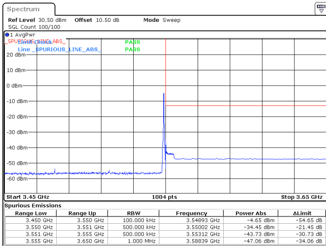
70MHz_30kHz_3515MHz_DFT-s-OFDM QPSK_RB1@188 -34.45 dBm
