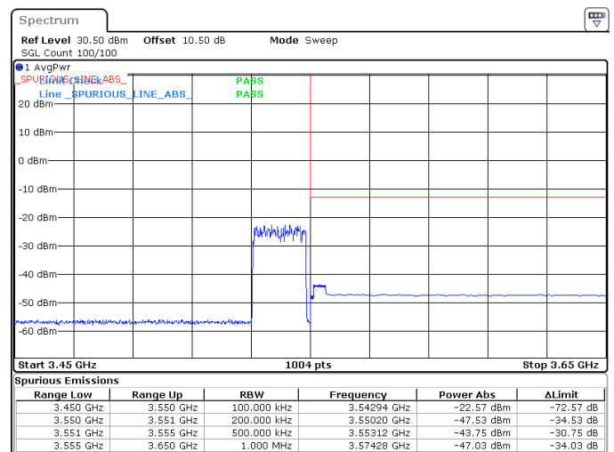
20MHz_15kHz_3540MHz_DFT-s-OFDM QPSK_RB100@0 -43.75 dBm
