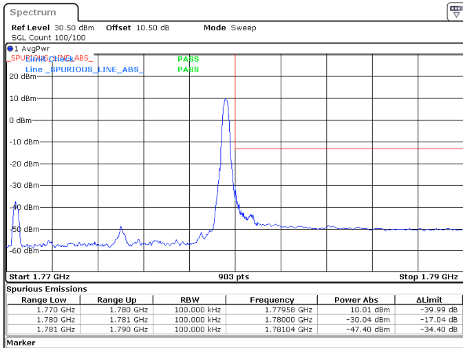
10MHz_15kHz_1775MHz_DFT-s-OFDM QPSK_RB1@51 -30.04 dBm
