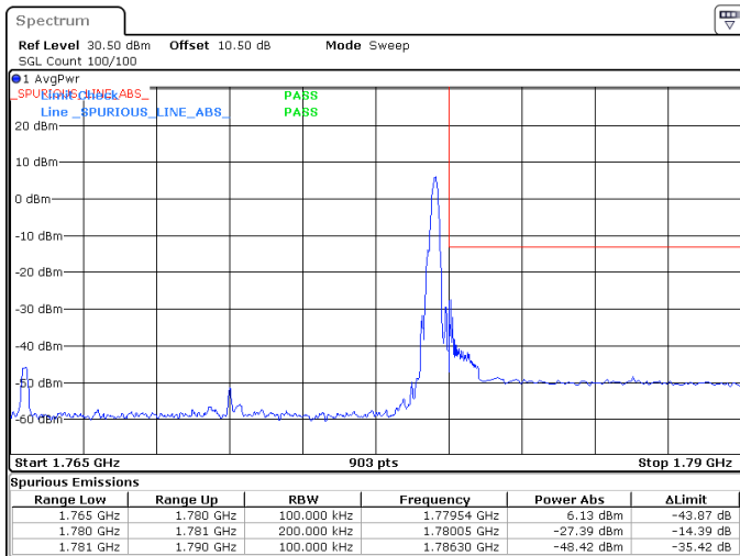
15MHz_15kHz_1772.5MHz_DFT-s-OFDM QPSK_RB1@78 -27.39 dBm
