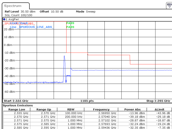
15MHz_15kHz_2562.5MHz_DFT-s-OFDM QPSK_RB1@78 -32.35 dBm
