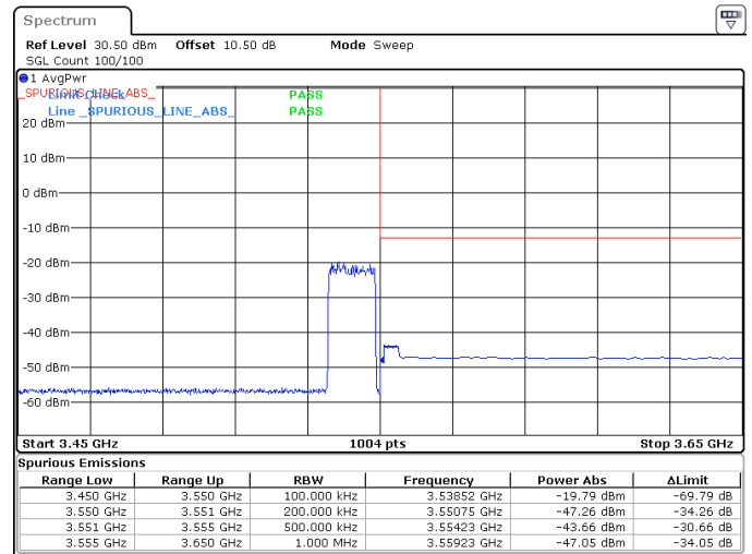
15MHz_30kHz_3542.5MHz_DFT-s-OFDM QPSK_RB36@0 -43.66 dBm
