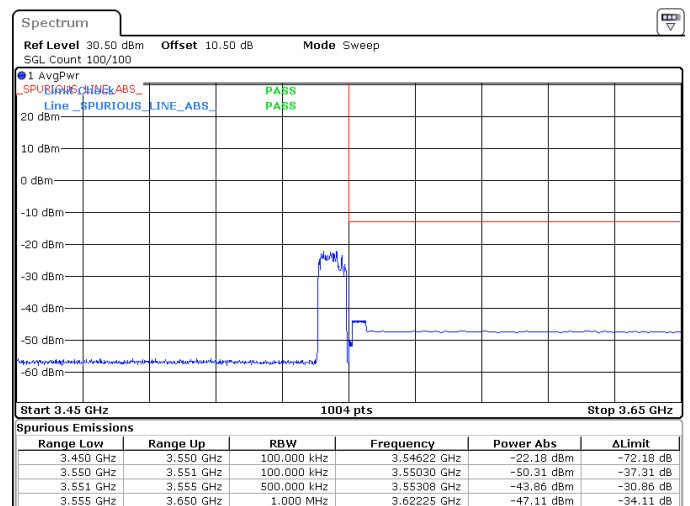
10MHz_30kHz_3545MHz_DFT-s-OFDM QPSK_RB24@0 -43.86 dBm
