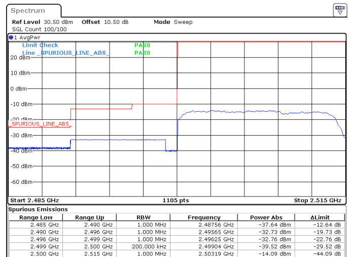
15MHz_15kHz_2507.5MHz_DFT-s-OFDM QPSK_RB75@0 -37.64 dBm
