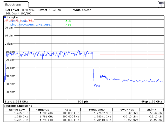
15MHz_15kHz_1772.5MHz_DFT-s-OFDM QPSK_RB75@0 -39.10 dBm
