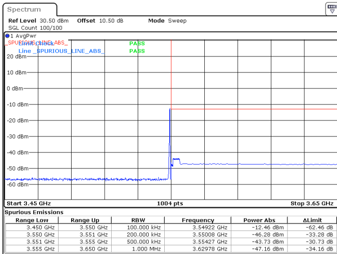
15MHz_30kHz_3542.5MHz_DFT-s-OFDM QPSK_RB1@37 -43.73 dBm
