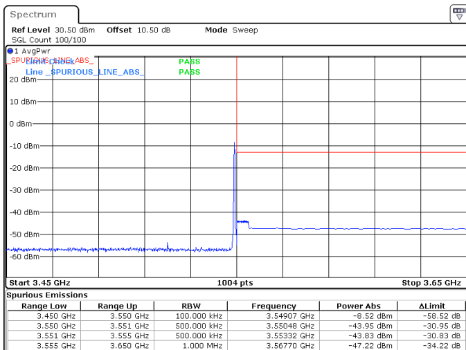
60MHz_30kHz_3520MHz_DFT-s-OFDM QPSK_RB1@161 -43.83 dBm
