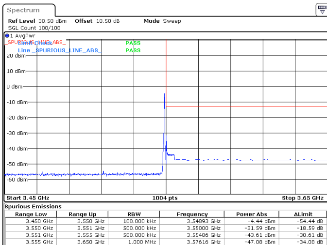
40MHz_30kHz_3530MHz_DFT-s-OFDM QPSK_RB1@105 -31.59 dBm
