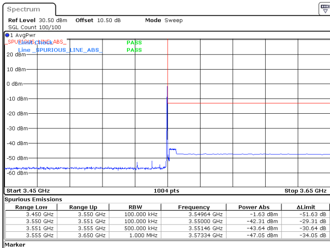
10MHz_15kHz_3545MHz_DFT-s-OFDM QPSK_RB1@51 -42.31 dBm
