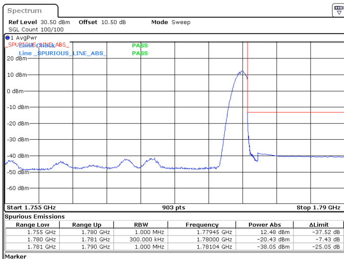
25MHz_15kHz_1767.5MHz_DFT-s-OFDM QPSK_RB1@132 -20.43 dBm
