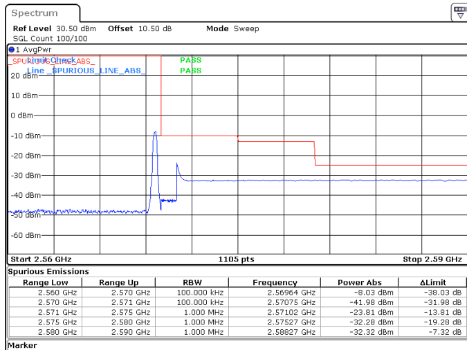
10MHz_15kHz_2565MHz_DFT-s-OFDM QPSK_RB1@51 -32.32 dBm
