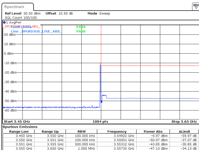
10MHz_30kHz_3545MHz_DFT-s-OFDM QPSK_RB1@23 -43.85 dBm
