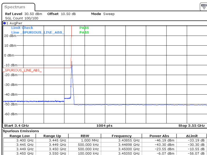
50MHz_15kHz_3475MHz_DFT-s-OFDM QPSK_RB1@0 -23.55 dBm
