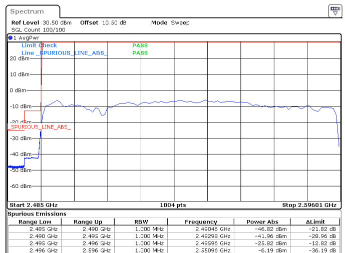
100MHz_30kHz_2546.01MHz_DFT-s-OFDM QPSK_RB270@0 -25.82 dBm
