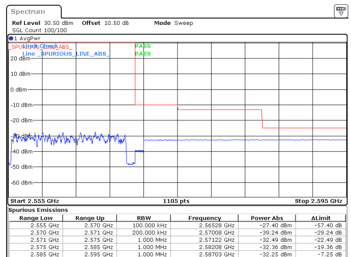
15MHz_15kHz_2562.5MHz_DFT-s-OFDM QPSK_RB75@0 -32.25 dBm
