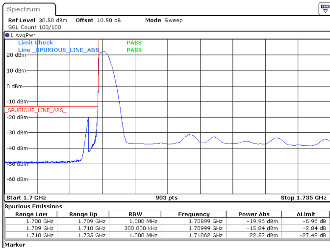
25MHz_15kHz_1722.5MHz_DFT-s-OFDM QPSK_RB1@0 -15.84 dBm
