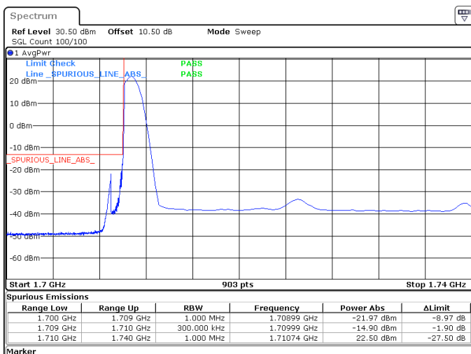
30MHz_15kHz_1725MHz_DFT-s-OFDM QPSK_RB1@0 -14.90 dBm
