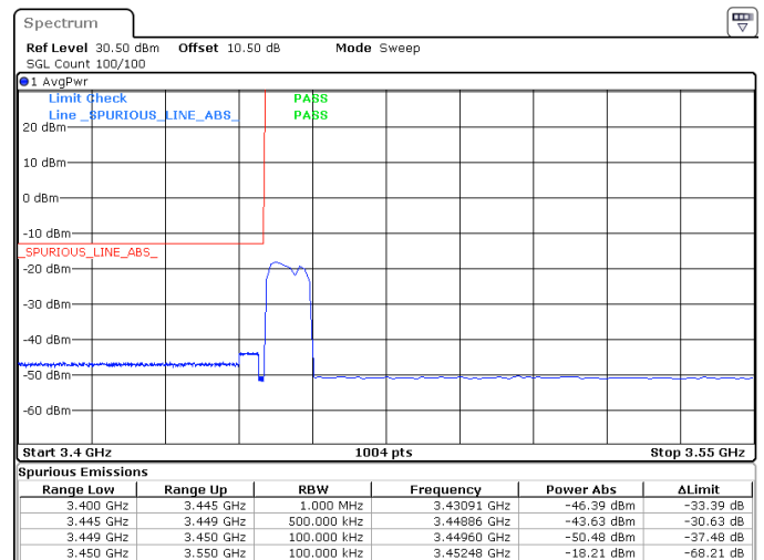
10MHz_30kHz_3545MHz_DFT-s-OFDM QPSK_RB24@0 -43.63 dBm
