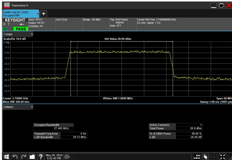
30MHz_30kHz_3750MHz_DFT-s-OFDM 64 QAM_RB75@0
