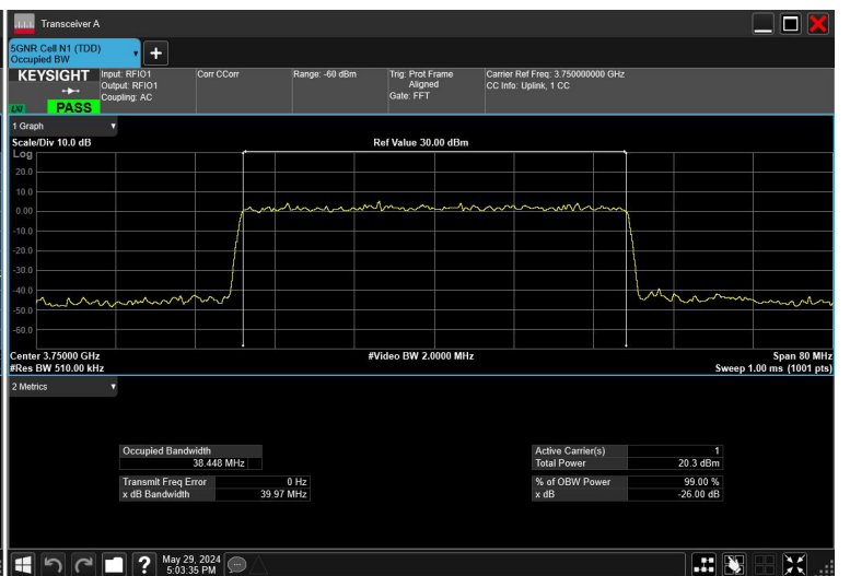
40MHz_15kHz_3750MHz_CP-OFDM 64 QAM_RB216@0
