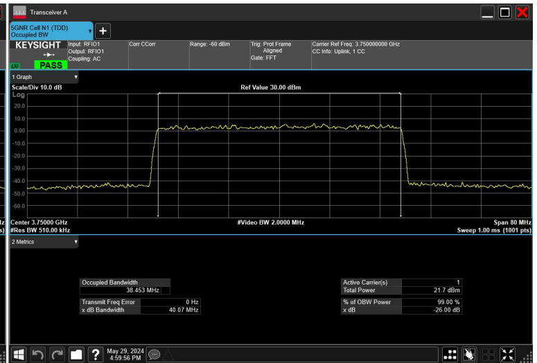
40MHz_15kHz_3750MHz_DFT-s-OFDM 16 QAM_RB216@0
