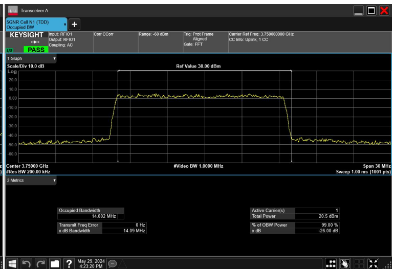
15MHz_15kHz_3750MHz_DFT-s-OFDM 64 QAM_RB75@0
