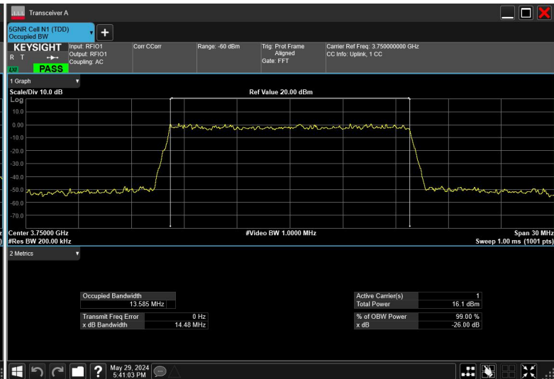
15MHz_30kHz_3750MHz_CP-OFDM 256 QAM_RB38@0
