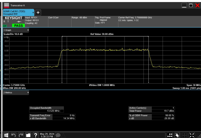
15MHz_30kHz_3750MHz_CP-OFDM QPSK_RB38@0
