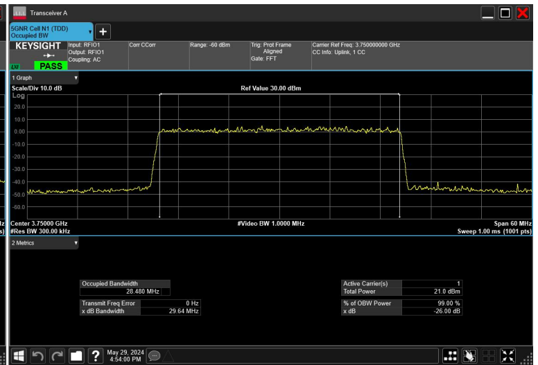
30MHz_15kHz_3750MHz_DFT-s-OFDM 64 QAM_RB160@0
