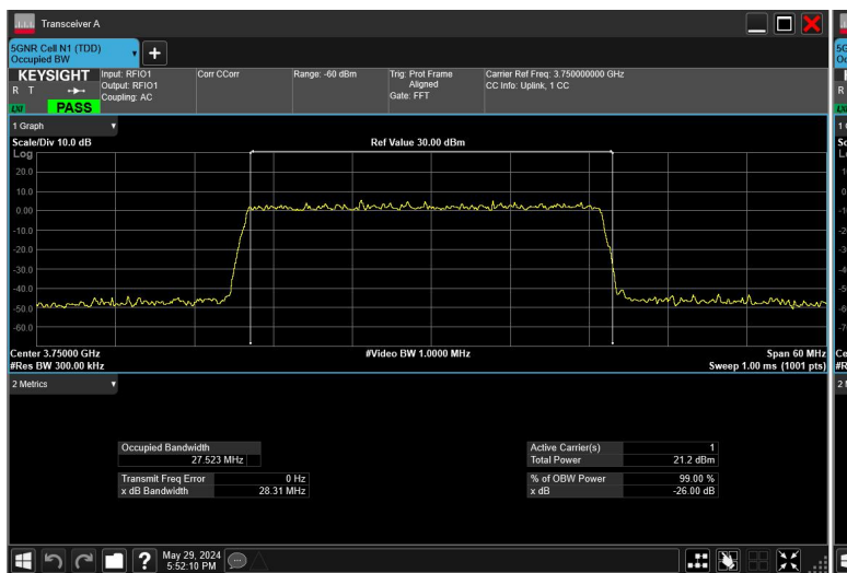
30MHz_30kHz_3750MHz_DFT-s-OFDM 16 QAM_RB75@0
