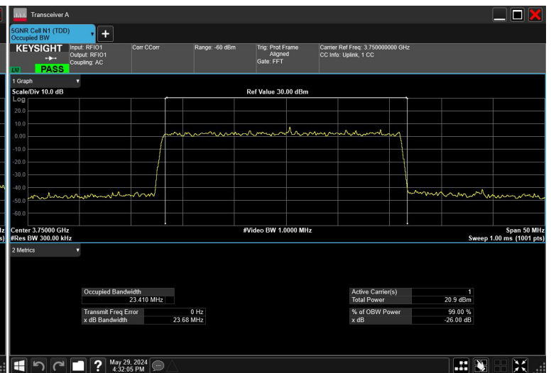
25MHz_15kHz_3750MHz_DFT-s-OFDM 64 QAM_RB128@0
