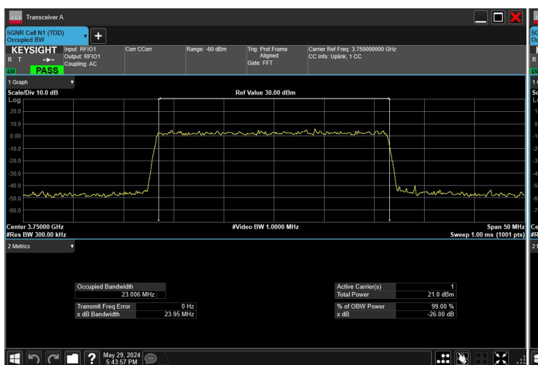
25MHz_30kHz_3750MHz_DFT-s-OFDM 16 QAM_RB64@0
