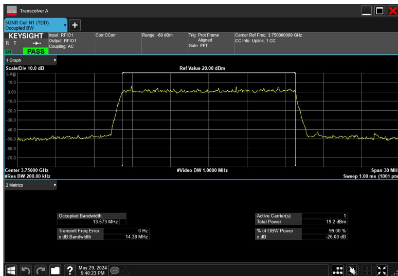
15MHz_30kHz_3750MHz_CP-OFDM 64 QAM_RB38@0
