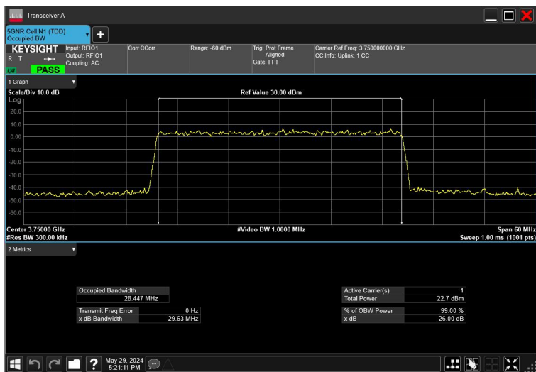
30MHz_15kHz_3750MHz_DFT-s-OFDM QPSK_RB160@0
