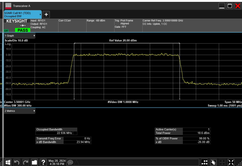
25MHz_30kHz_3500MHz_DFT-s-OFDM 16QAM_RB64@0
