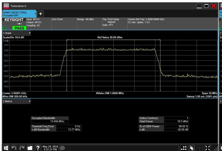
15MHz_30kHz_3500MHz_DFT-s-OFDM QPSK_RB36@0
