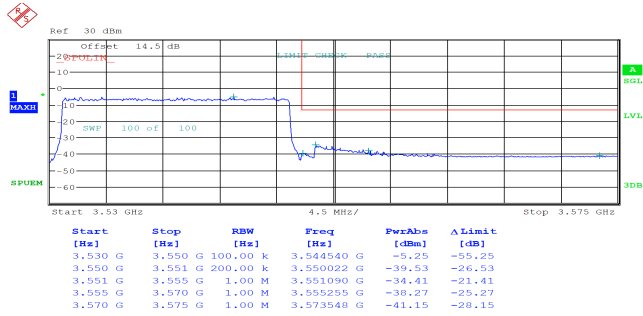
20MHz_High_QPSK_100@0
