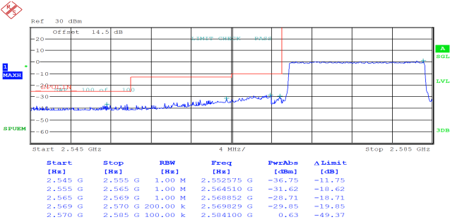
15MHz_Low_QPSK_75@0
