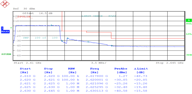
10MHz_High_QPSK_50@0
