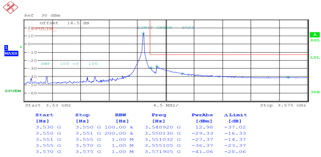
20MHz_High_QPSK_1@99
