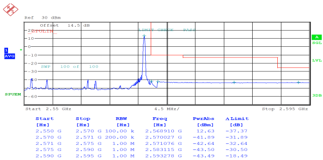
20MHz_High_QPSK_1@99
