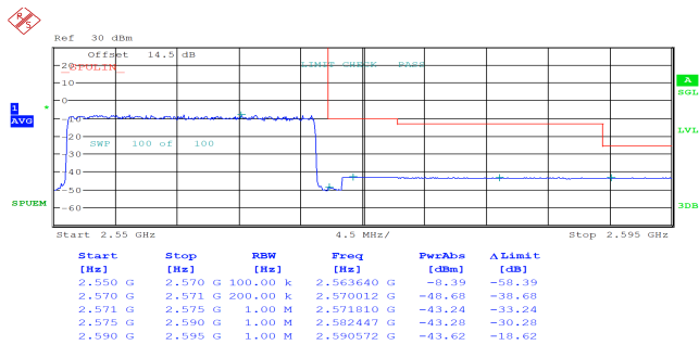
20MHz_High_QPSK_100@0
