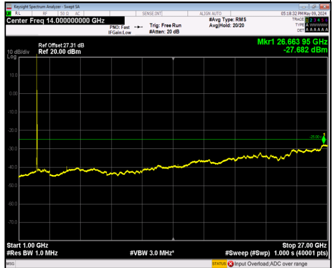
Band7_20MHz_QPSK_21100_1RB#0_1000~27000_1000~27000
