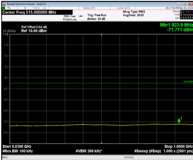
Band7_20MHz_QPSK_21100_1RB#0_30~1000_30~1000
