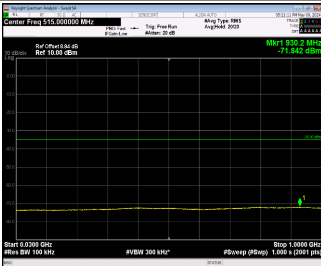
Band7_20MHz_QPSK_21350_1RB#0_30~1000_30~1000
