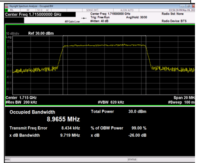
Band4-10MHz-64QAM-20000-50RB#0-PASS
