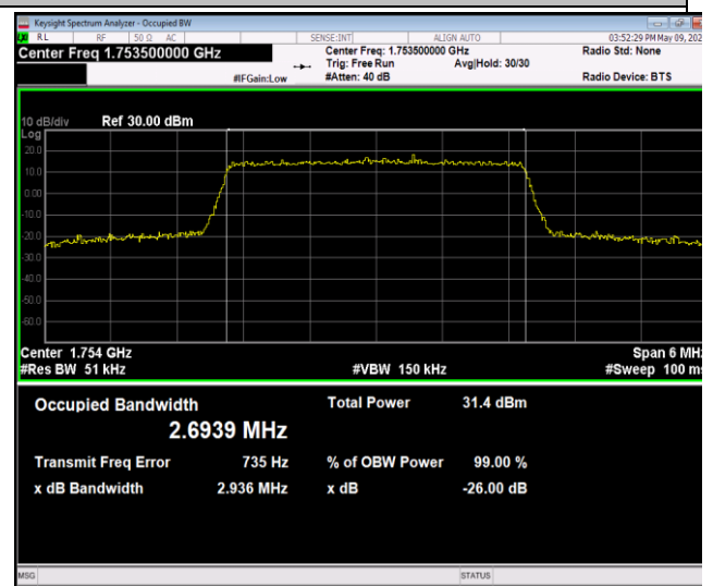
Band4-3MHz-QPSK-20385-15RB#0-PASS
