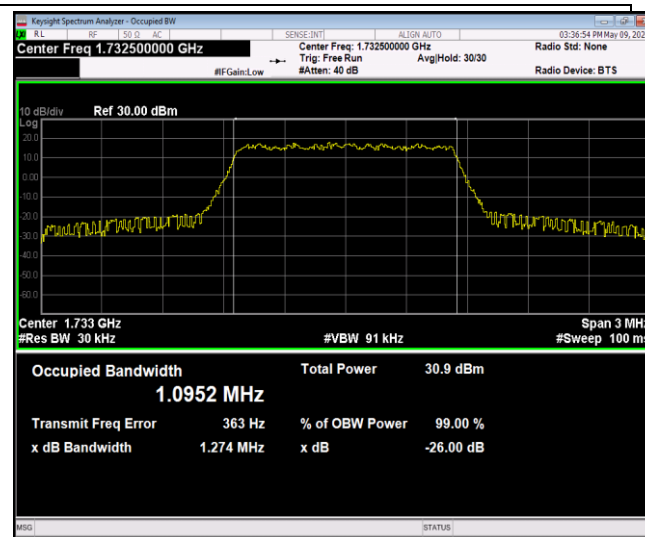
Band4-1.4MHz-QPSK-20175-6RB#0-PASS
