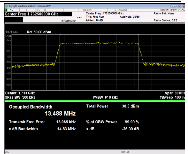
Band4-15MHz-64QAM-20175-75RB#0-PASS
