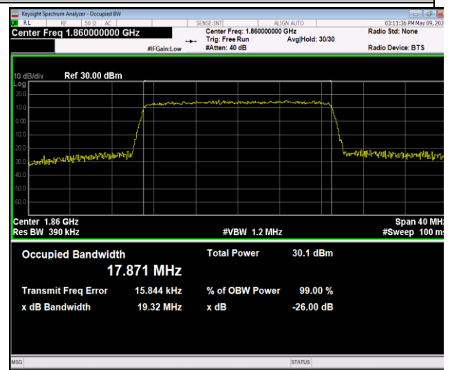
Band2-20MHz-64QAM-18700-100RB#0-PASS
