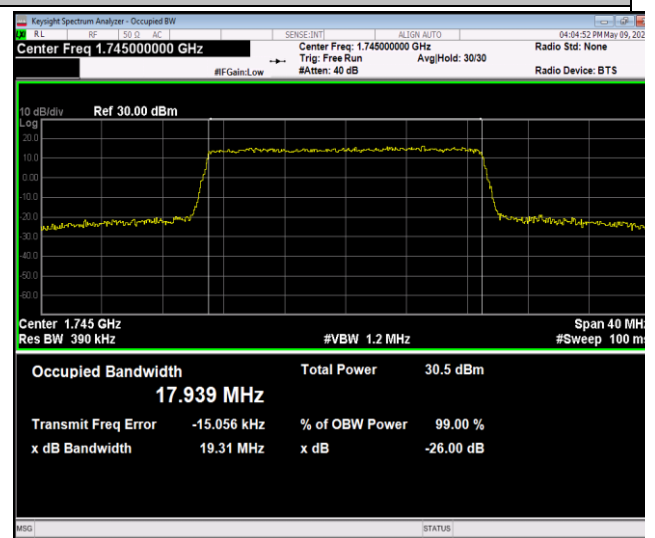
Band4-20MHz-64QAM-20300-100RB#0-PASS
