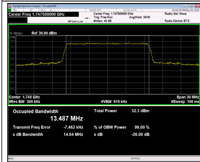
Band4-15MHz-QPSK-20325-75RB#0-PASS
