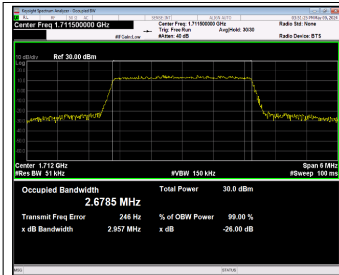
Band4-3MHz-16QAM-19965-15RB#0-PASS
