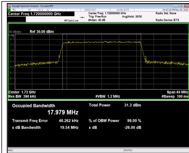
Band4-20MHz-16QAM-20050-100RB#0-PASS
