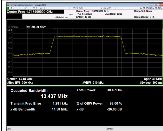
Band4-15MHz-64QAM-20325-75RB#0-PASS
