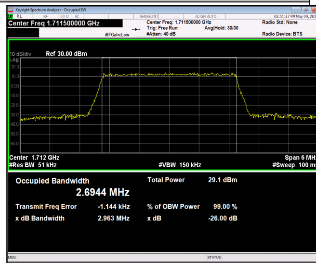
Band4-3MHz-64QAM-19965-15RB#0-PASS
