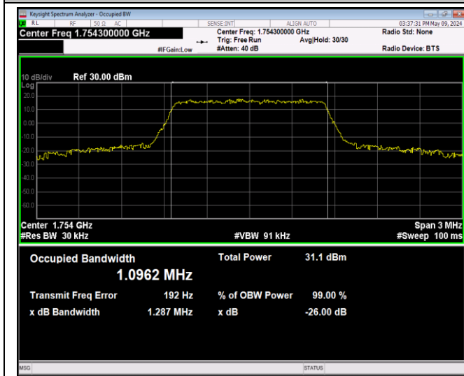
Band4-1.4MHz-QPSK-20393-6RB#0-PASS
