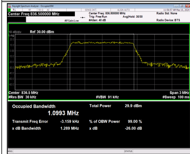
Band5-1.4MHz-16QAM-20525-6RB#0-PASS
