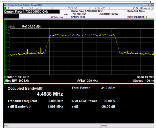
Band4-5MHz-QPSK-20175-25RB#0-PASS
