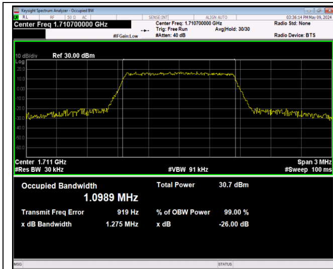
Band4-1.4MHz-QPSK-19957-6RB#0-PASS
