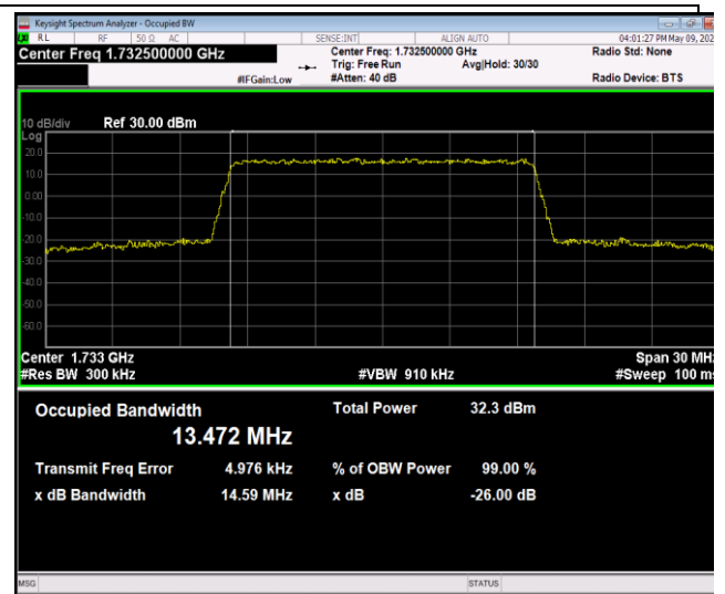
Band4-15MHz-QPSK-20175-75RB#0-PASS
