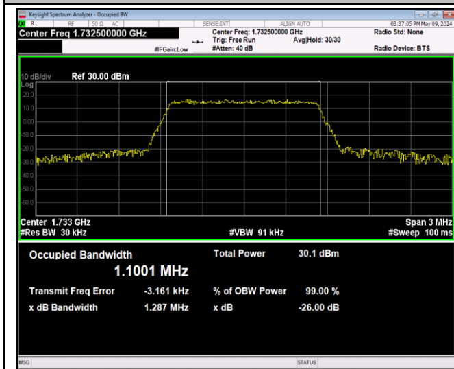
Band4-1.4MHz-16QAM-20175-6RB#0-PASS
