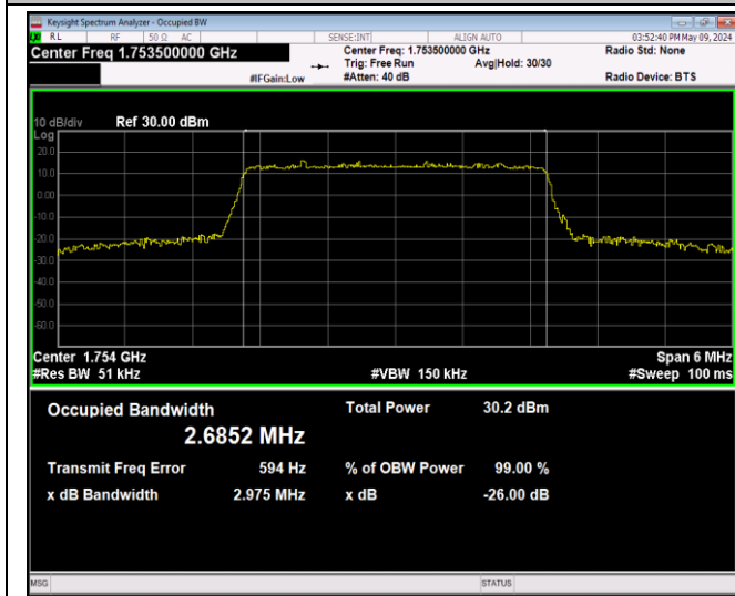
Band4-3MHz-16QAM-20385-15RB#0-PASS
