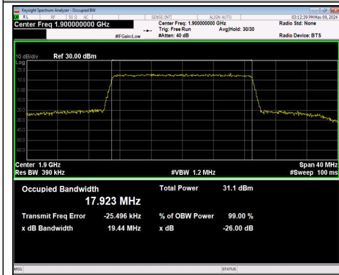
Band2-20MHz-16QAM-19100-100RB#0-PASS
