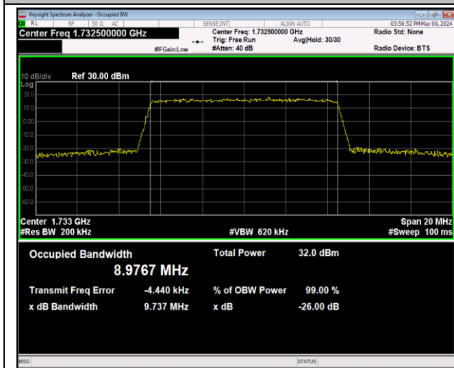
Band4-10MHz-QPSK-20175-50RB#0-PASS
