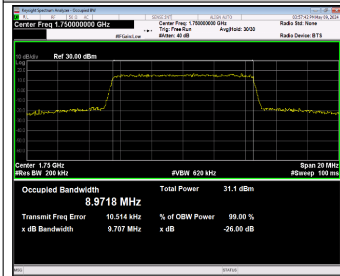
Band4-10MHz-16QAM-20350-50RB#0-PASS
