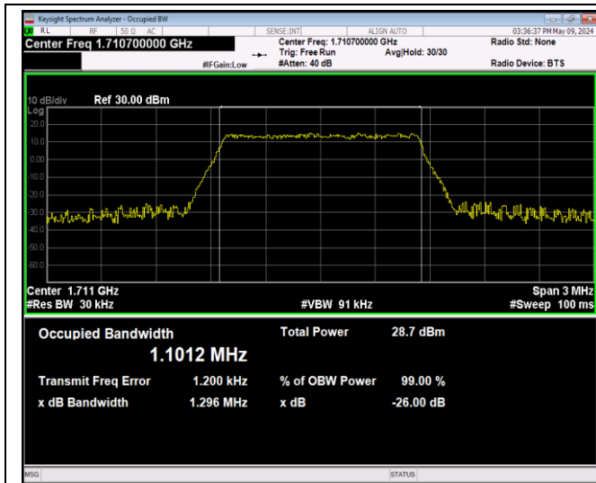
Band4-1.4MHz-64QAM-19957-6RB#0-PASS
