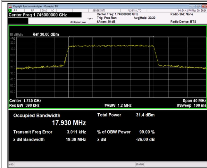
Band4-20MHz-16QAM-20300-100RB#0-PASS
