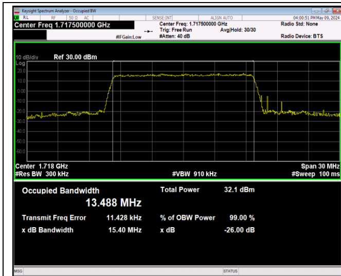
Band4-15MHz-QPSK-20025-75RB#0-PASS
