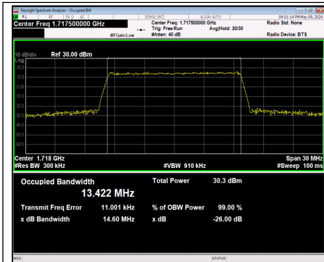
Band4-15MHz-64QAM-20025-75RB#0-PASS
