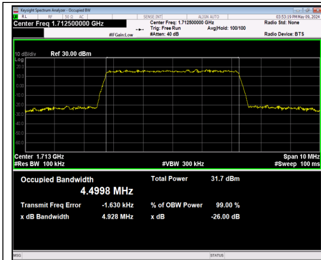
Band4-5MHz-QPSK-19975-25RB#0-PASS
