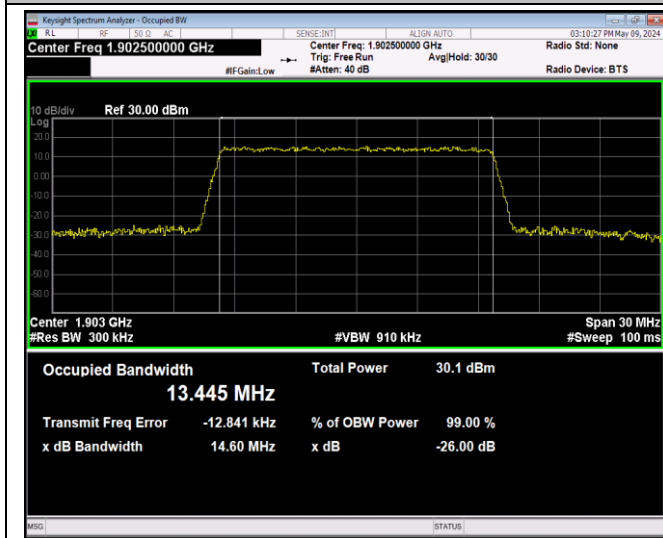
Band2-15MHz-64QAM-19125-75RB#0-PASS
