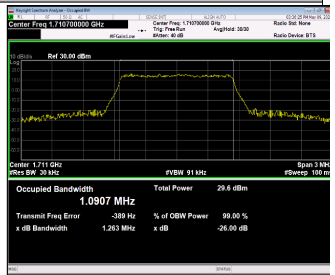
Band4-1.4MHz-16QAM-19957-6RB#0-PASS
