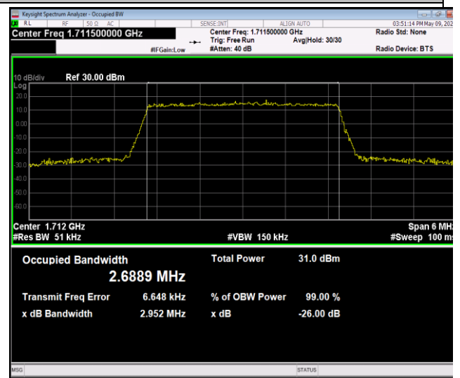
Band4-3MHz-QPSK-19965-15RB#0-PASS
