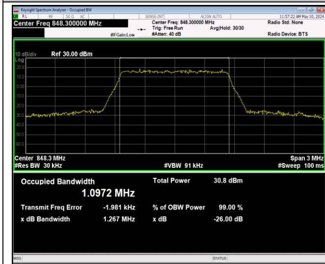
Band5-1.4MHz-QPSK-20643-6RB#0-PASS
