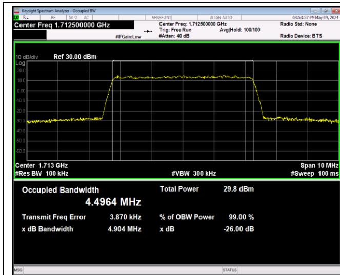
Band4-5MHz-64QAM-19975-25RB#0-PASS
