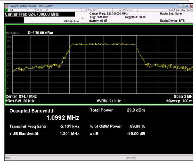
Band5-1.4MHz-16QAM-20407-6RB#0-PASS
