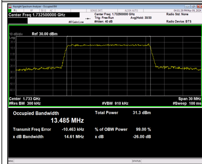
Band4-15MHz-16QAM-20175-75RB#0-PASS
