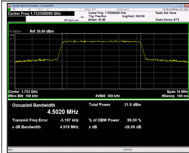
Band4-5MHz-QPSK-20375-25RB#0-PASS
