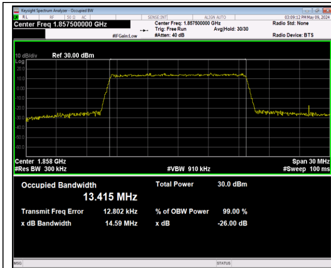
Band2-15MHz-64QAM-18675-75RB#0-PASS
