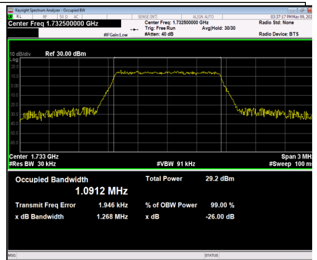
Band4-1.4MHz-64QAM-20175-6RB#0-PASS
