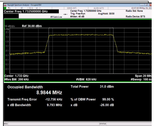
Band4-10MHz-16QAM-20175-50RB#0-PASS
