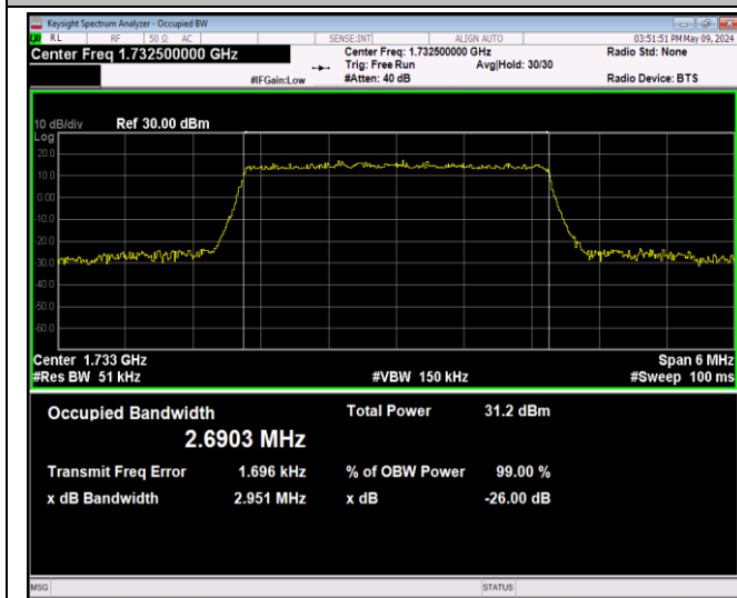
Band4-3MHz-QPSK-20175-15RB#0-PASS
