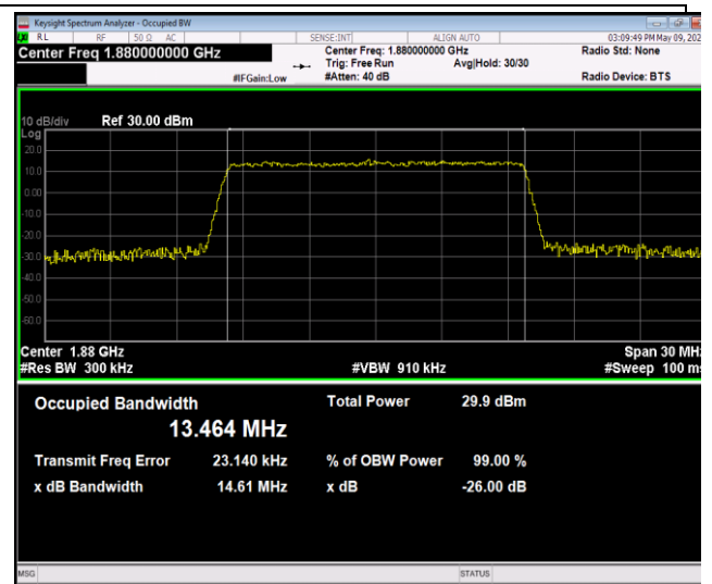
Band2-15MHz-64QAM-18900-75RB#0-PASS
