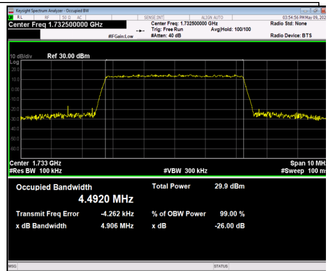
Band4-5MHz-64QAM-20175-25RB#0-PASS
