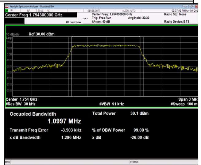
Band4-1.4MHz-16QAM-20393-6RB#0-PASS
