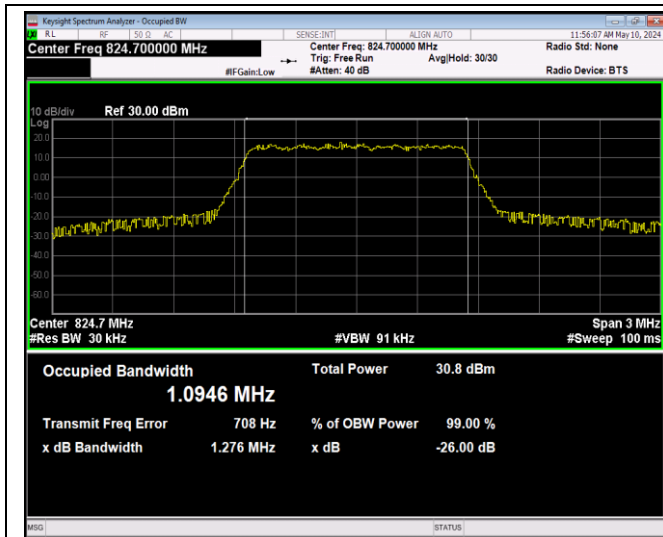
Band5-1.4MHz-QPSK-20407-6RB#0-PASS
