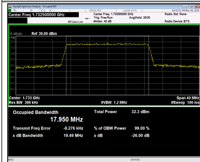
Band4-20MHz-QPSK-20175-100RB#0-PASS
