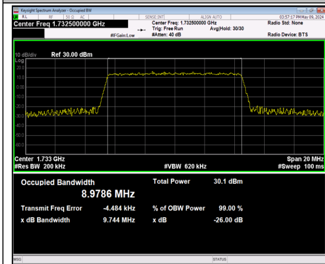
Band4-10MHz-64QAM-20175-50RB#0-PASS
