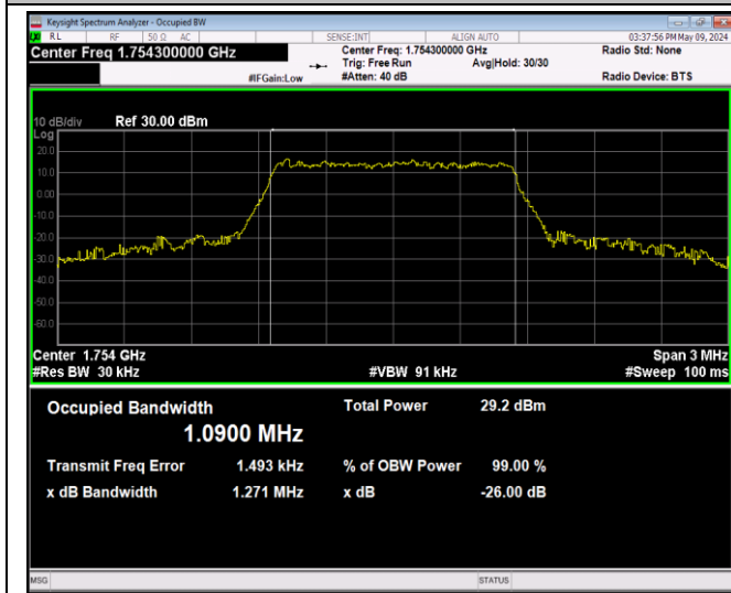
Band4-1.4MHz-64QAM-20393-6RB#0-PASS
