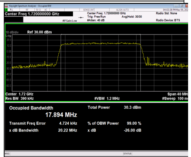
Band4-20MHz-64QAM-20050-100RB#0-PASS
