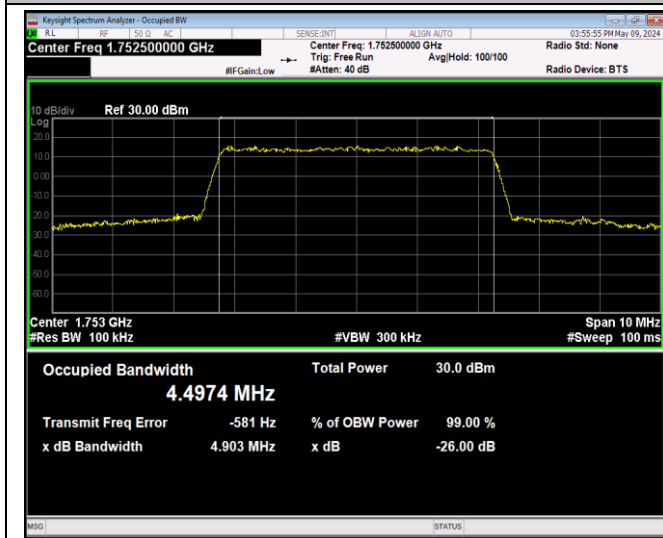
Band4-5MHz-64QAM-20375-25RB#0-PASS
