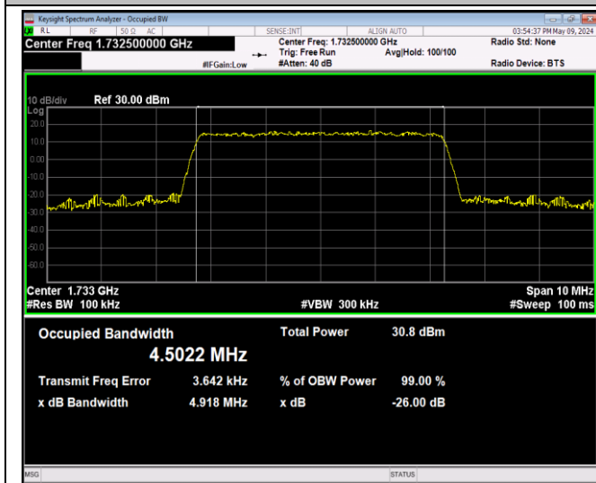
Band4-5MHz-16QAM-20175-25RB#0-PASS
