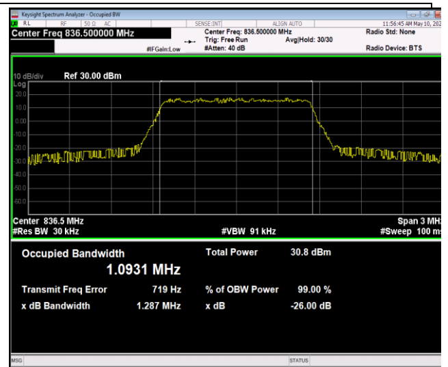
Band5-1.4MHz-QPSK-20525-6RB#0-PASS
