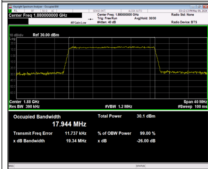
Band2-20MHz-64QAM-18900-100RB#0-PASS
