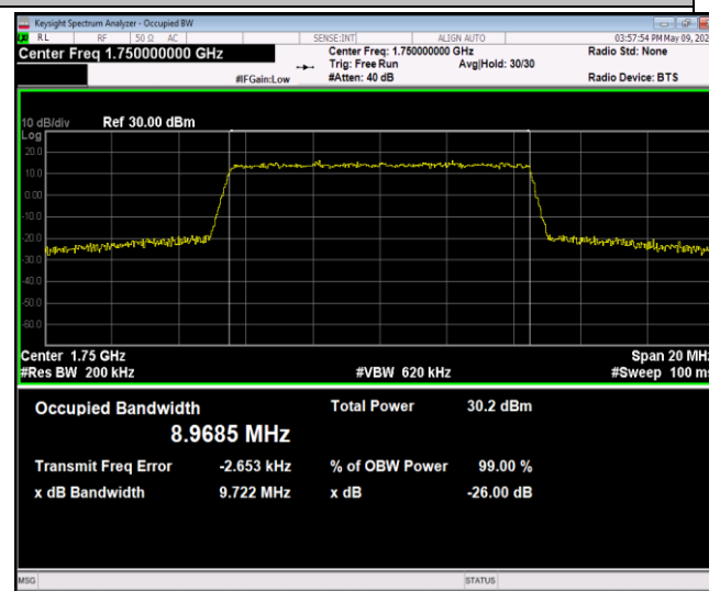
Band4-10MHz-64QAM-20350-50RB#0-PASS
