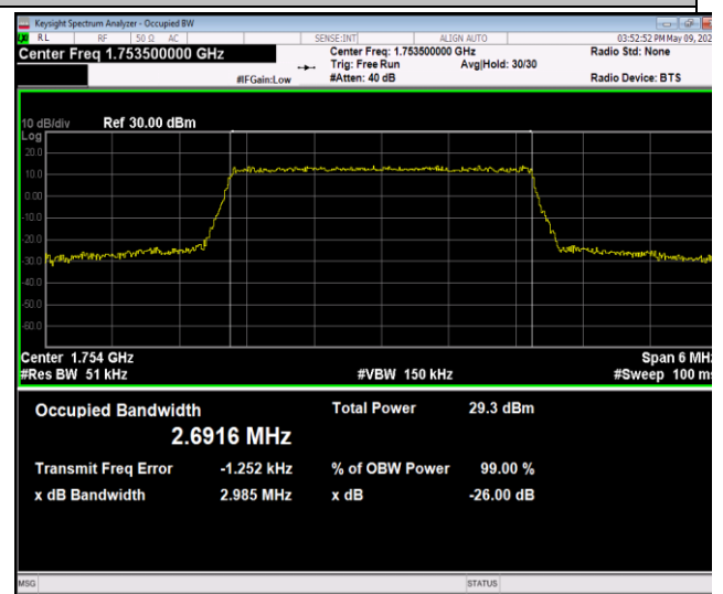
Band4-3MHz-64QAM-20385-15RB#0-PASS
