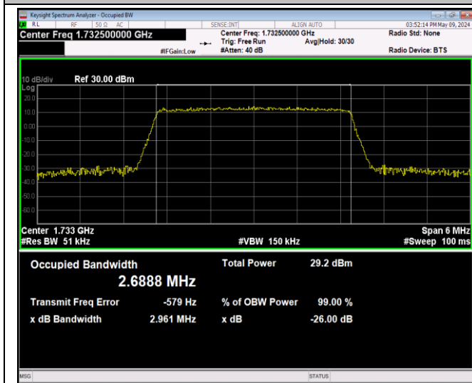
Band4-3MHz-64QAM-20175-15RB#0-PASS
