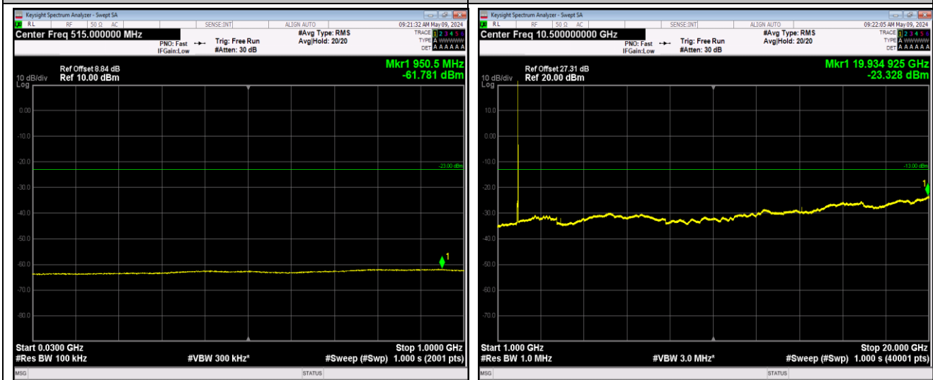
Band2_20MHz_64QAM_18900_1RB#0_1000~20000
