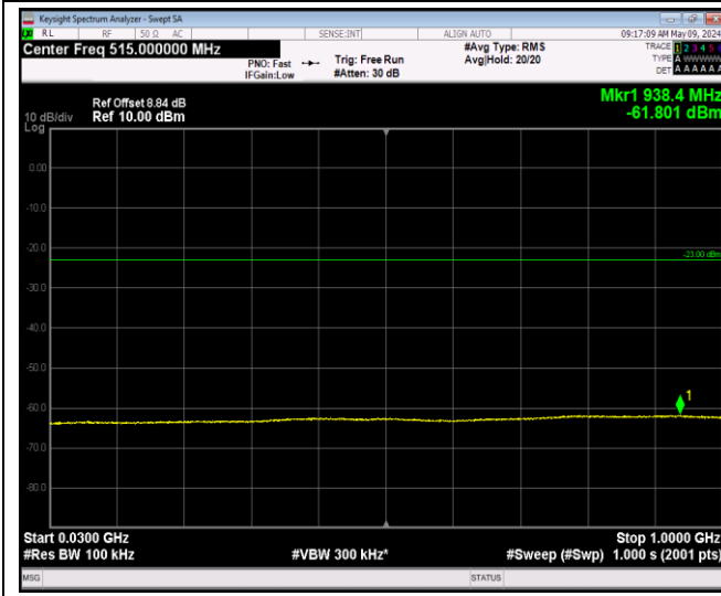
Band2_20MHz_16QAM_18900_1RB#0_30~1000_30~100 0
