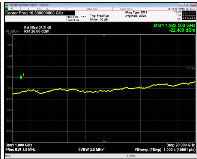
Band2_1.4MHz_QPSK_18900_1RB#01000~20000
