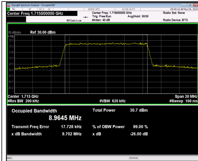
Band4-10MHz-16QAM-20000-50RB#0-PASS
