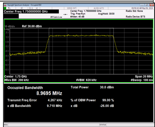
Band4-10MHz-64QAM-20350-50RB#0-PASS
