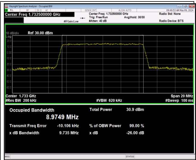
Band4-10MHz-16QAM-20175-50RB#0-PASS
