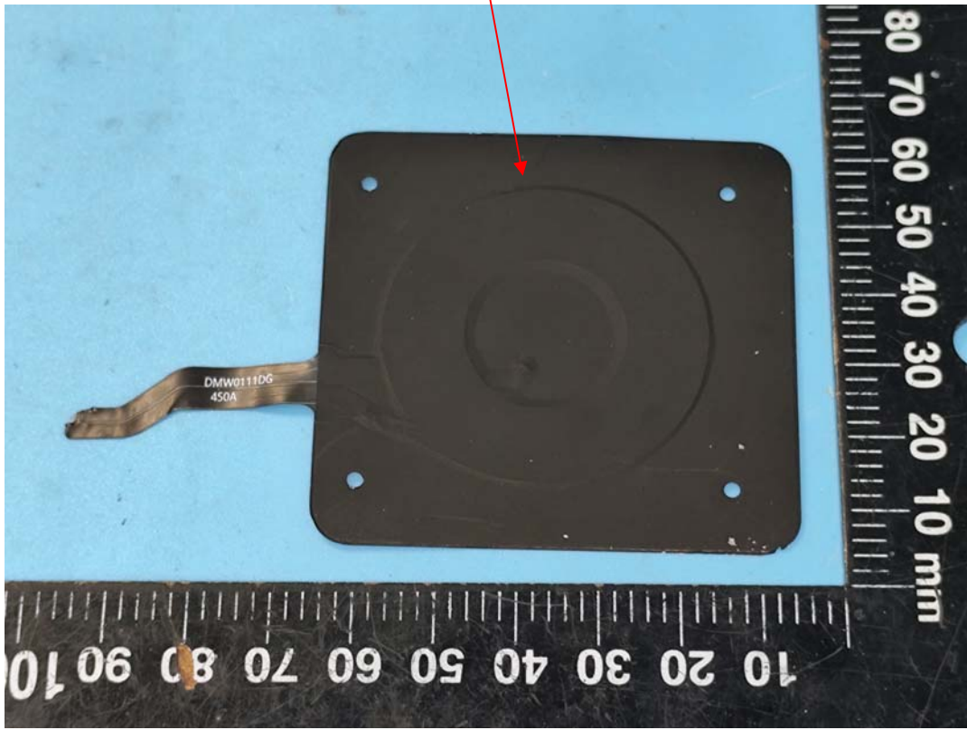
WPT Antenna
