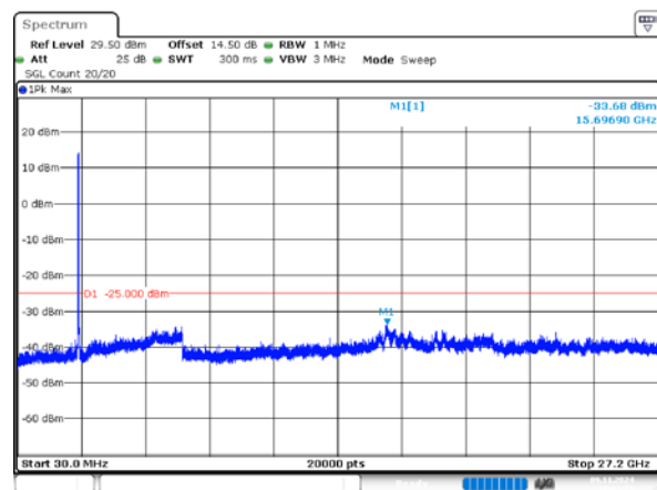
15MHz_Middle_QPSK_75@0(30MHz~27.2GHz)
