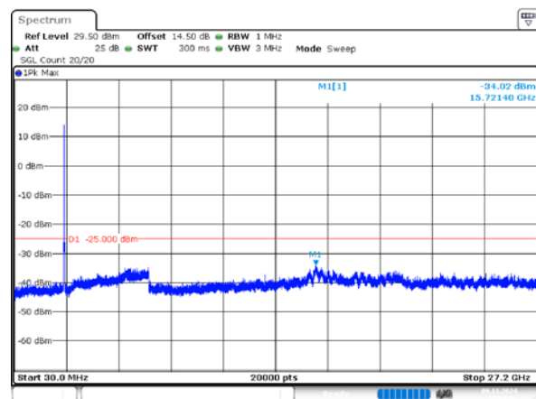
15MHz_High_QPSK_75@0(30MHz~27.2GHz)
