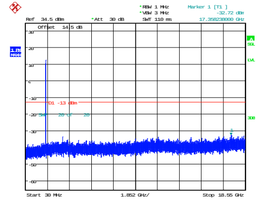
15MHz_Low_QPSK_75@0(30MHz~18.55GHz)
