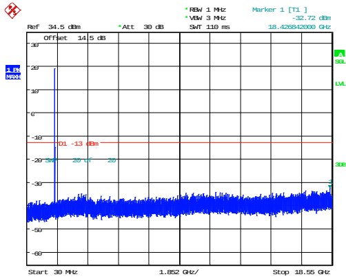
15MHz_Low_QPSK_1@0(30MHz~18.55GHz)
