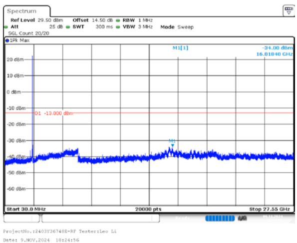
2_20MHz_High_QPSK_1@0(30MHz~27.55GHz)
