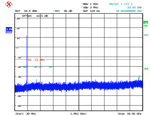
15MHz_Middle_QPSK_75@0(30MHz~18.55GHz)
