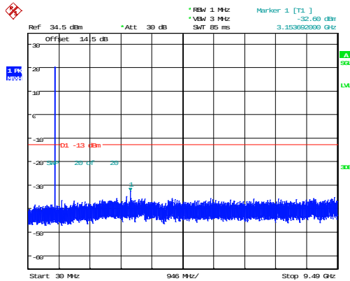
3MHz_High_QPSK_15@0(30MHz~9.49GHz)
