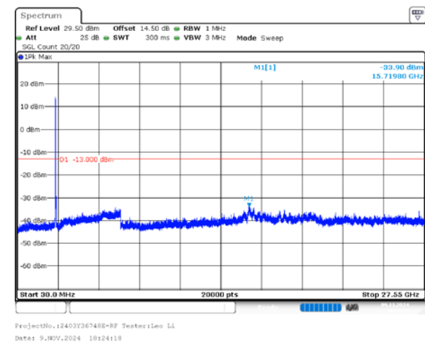
2_20MHz_High_QPSK_100@0(30MHz~27.55GHz)
