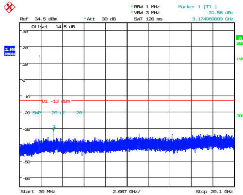
3MHz_Low_QPSK_15@0(30MHz~20.1GHz)
