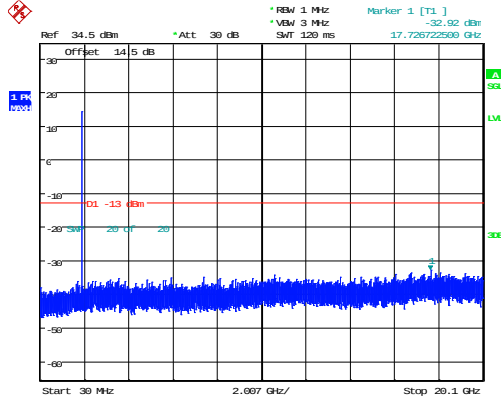
3MHz_High_QPSK_15@0(30MHz~20.1GHz)
