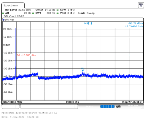
2_20MHz_Middle_QPSK_1@0(30MHz~27.55GHz)
