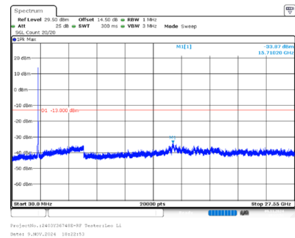
2_20MHz_Middle_QPSK_100@0(30MHz~27.55GHz)
