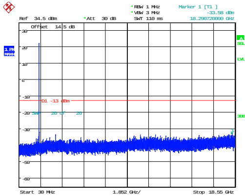
15MHz_Middle_QPSK_1@0(30MHz~18.55GHz)
