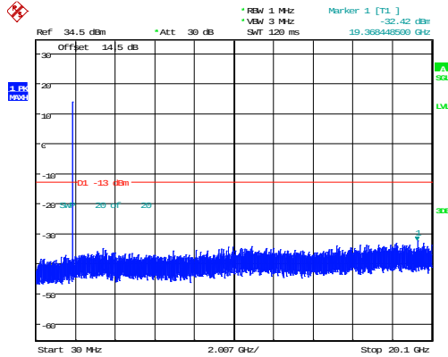
3MHz_Middle_QPSK_15@0(30MHz~20.1GHz)
