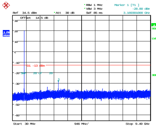
3MHz_Low_QPSK_15@0(30MHz~9.49GHz)
