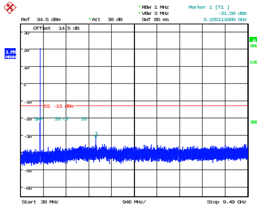
3MHz_Middle_QPSK_15@0(30MHz~9.49GHz)
