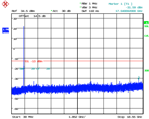
15MHz_High_QPSK_1@0(30MHz~18.55GHz)
