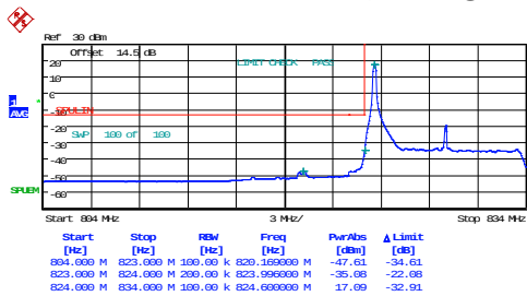
10MHz_Low_16QAM_1@0
