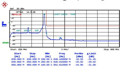
10MHz_High_QPSK_1@49
