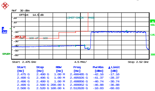
20MHz_Low_16QAM_100@0
