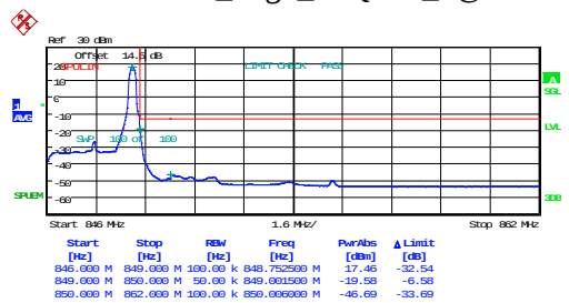
3MHz_High_16QAM_1@14
