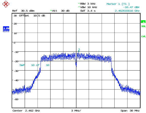
802.11g_2462MHz_Chain 0 -10.47dBm/3kHz
