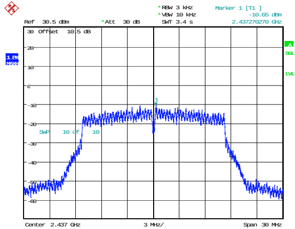
802.11g_2437MHz_Chain 0 -10.65dBm/3kHz
