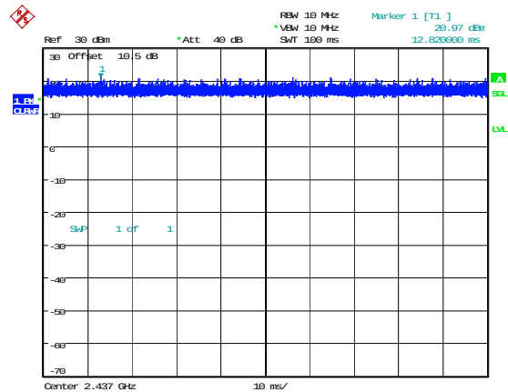
802.11g_2437MHz_Chain 0 100ms,100ms
