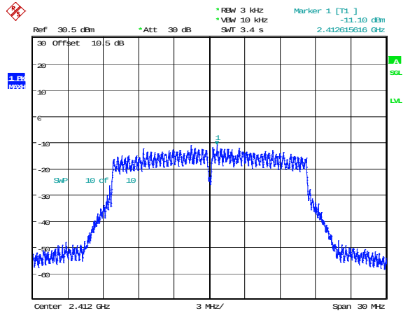
802.11g_2412MHz_Chain 1 -11.10dBm/3kHz
