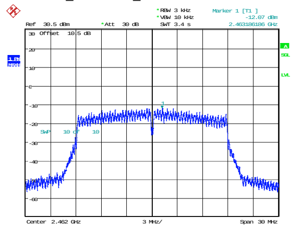
802.11n20_2462MHz_Chain 1 -12.07dBm/3kHz
