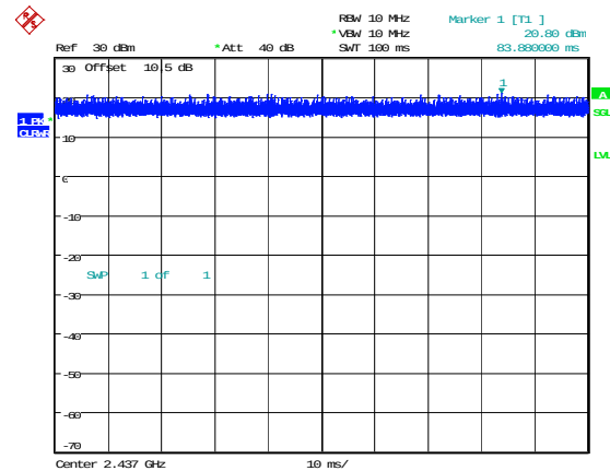
802.11g_2437MHz_Chain 1 100ms,100ms
