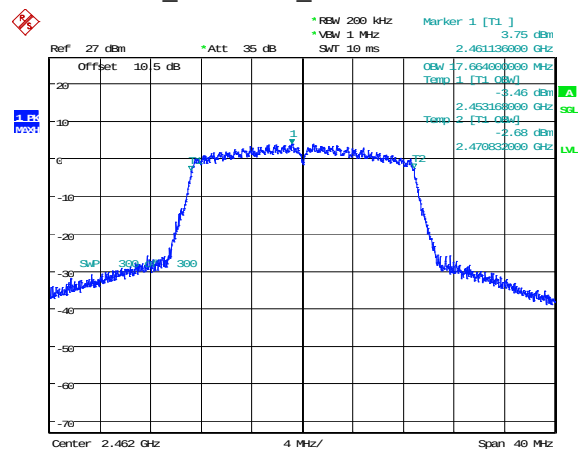
802.11n20_2462MHz_Chain 1 17.664MHz
