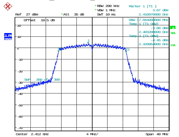
802.11n20_2412MHz_Chain 1 17.664MHz
