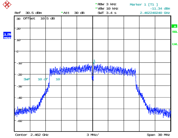
802.11g_2462MHz_Chain 1 -11.34dBm/3kHz
