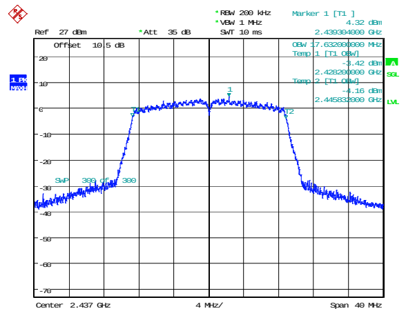
802.11n20_2437MHz_Chain 0 17.632MHz
