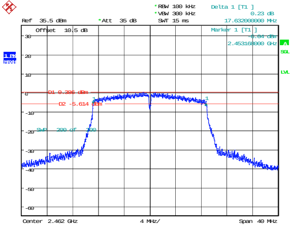
802.11n20_2462MHz_Chain 0 17.632MHz
