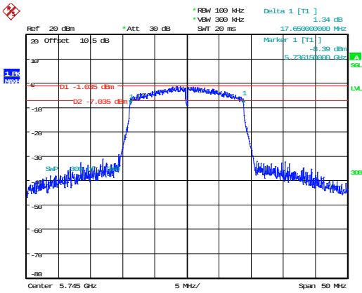
802.11n20_5745MHz 17.650MHz
