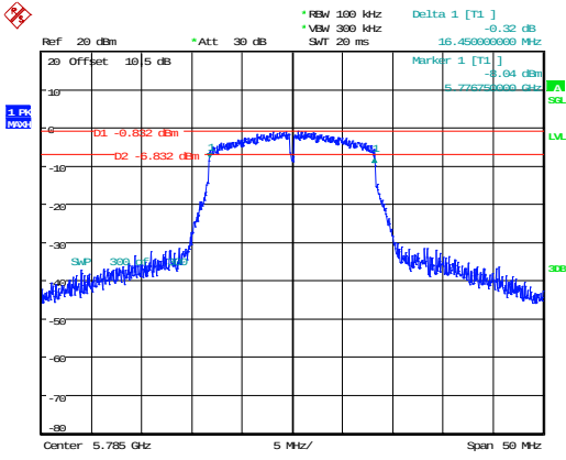
802.11a_5785MHz 16.450MHz
