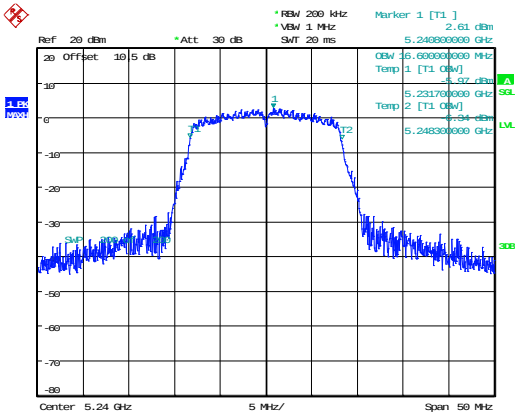
802.11a_5240MHz 16.600MHz
