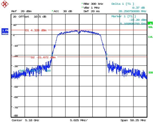
802.11a_5180MHz 20.251MHz
