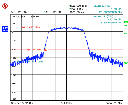
802.11a_5320MHz 20.502MHz
