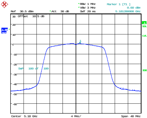
802.11n20_5180MHz
