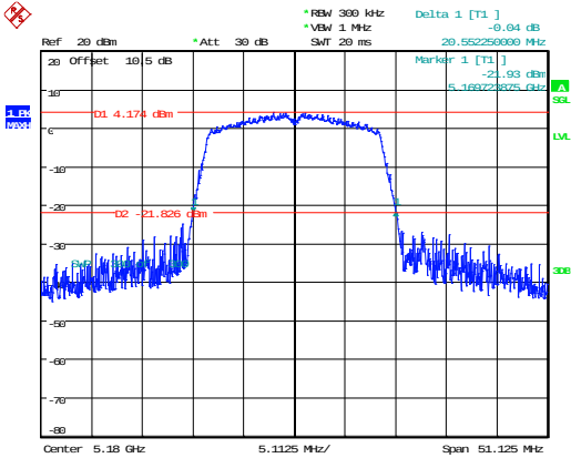
802.11n20_5180MHz 20.552MHz
