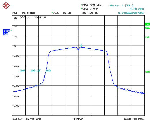
802.11n20_5745MHz
