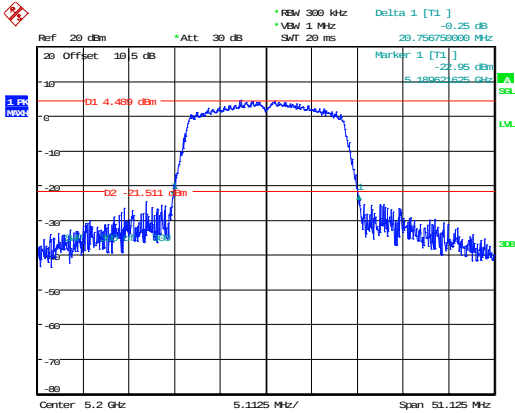
802.11n20_5200MHz 20.757MHz
