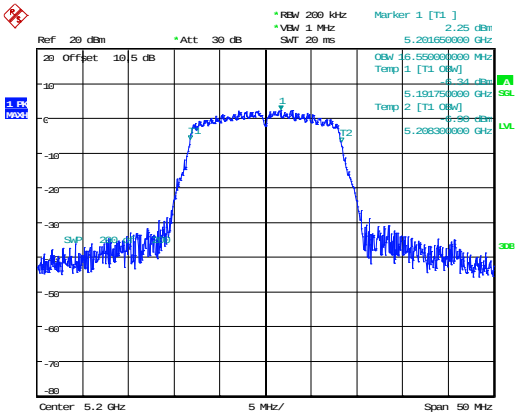
802.11a_5200MHz 16.550MHz
