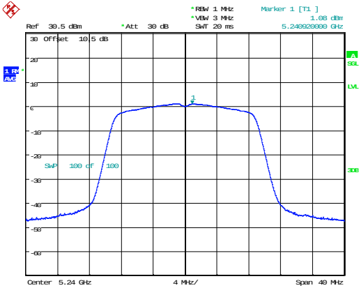
802.11n20_5240MHz
