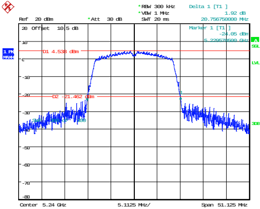
802.11n20_5240MHz 20.757MHz
