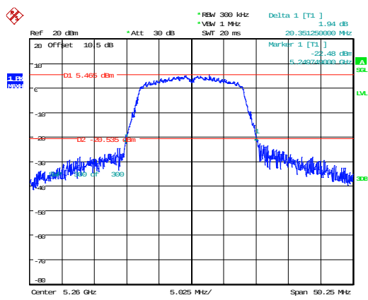
802.11a_5260MHz 20.351MHz
