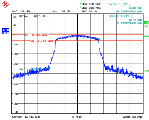
802.11a_5745MHz 16.450MHz
