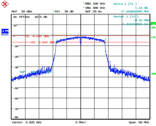
802.11n20_5825MHz 17.650MHz
