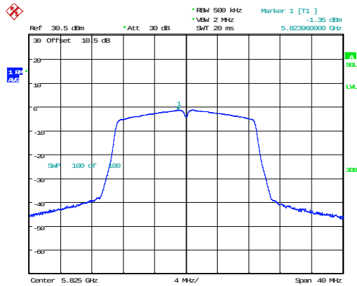
802.11n20_5825MHz
