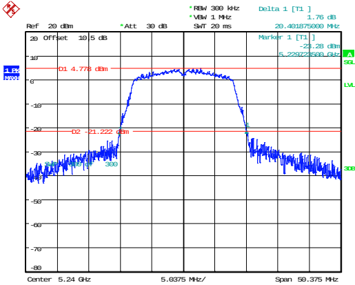
802.11a_5240MHz 20.402MHz
