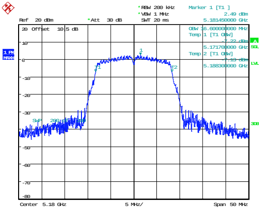
802.11a_5180MHz 16.600MHz
