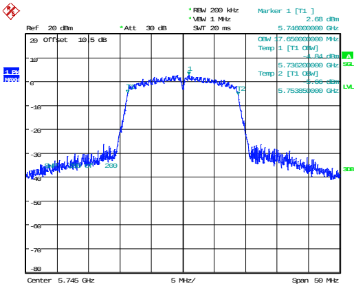
802.11n20_5745MHz 17.650MHz
