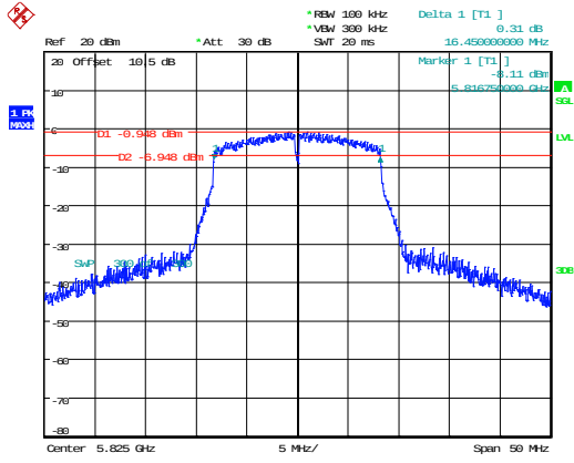
802.11a_5825MHz 16.450MHz
