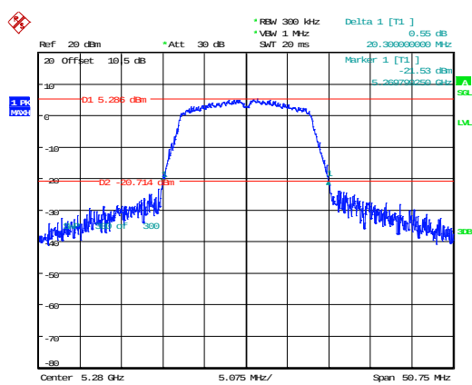
802.11a_5280MHz 20.300MHz
