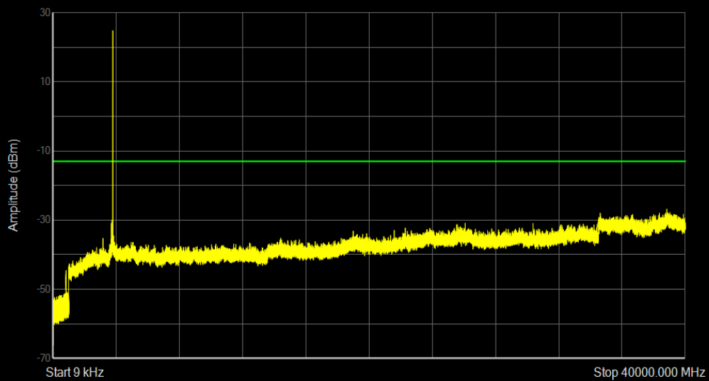
n78 SCS=30kHz CP_QPSK BW=100MHz Channel=650000 RB=1@272
