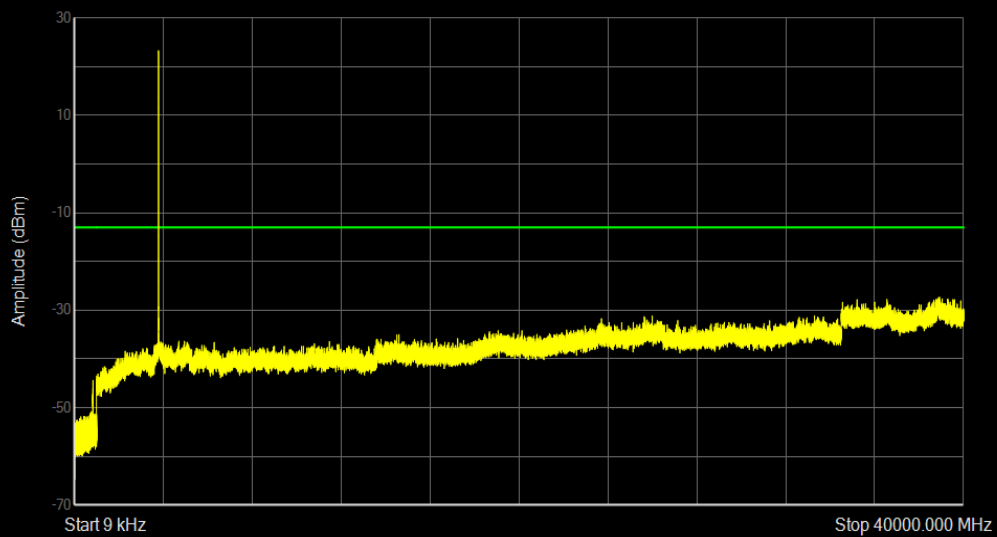
n78 SCS=30kHz CP_QPSK BW=10MHz Channel=653000 RB=1@0
