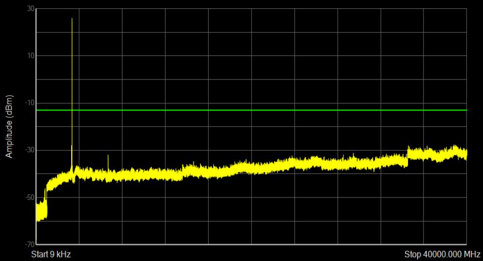
n78 SCS=30kHz CP_QPSK BW=50MHz Channel=621668 RB=1@132
