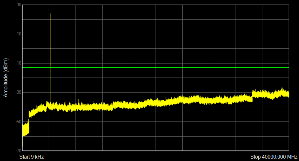
n77 SCS=30kHz CP_QPSK BW=10MHz Channel=679666 RB=1@23
