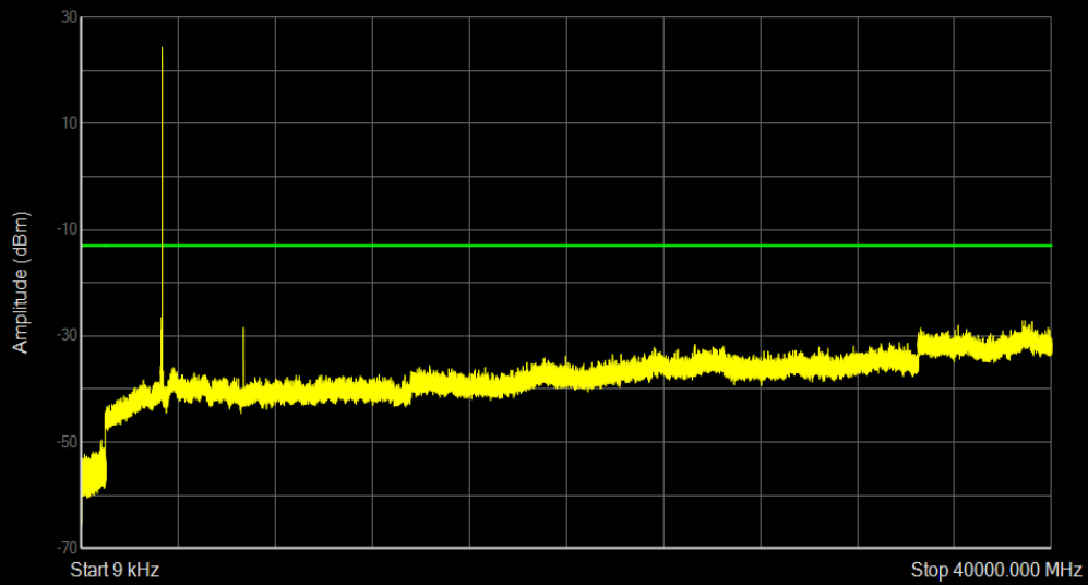
n77 SCS=30kHz CP_QPSK BW=50MHz Channel=621668 RB=1@132
