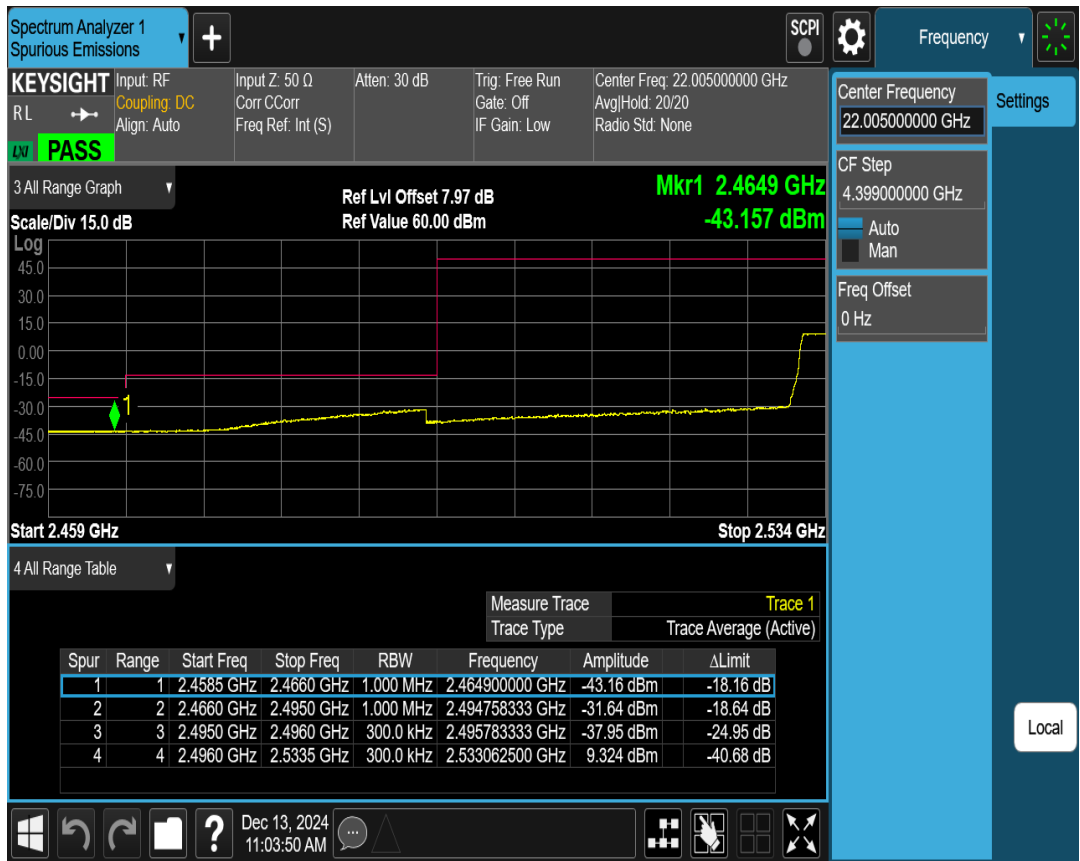
41C 16QAM PCC BW=15MHz Ch=39728 RB=1@0,SCC BW=20MHz Ch=39899 RB=1@99
