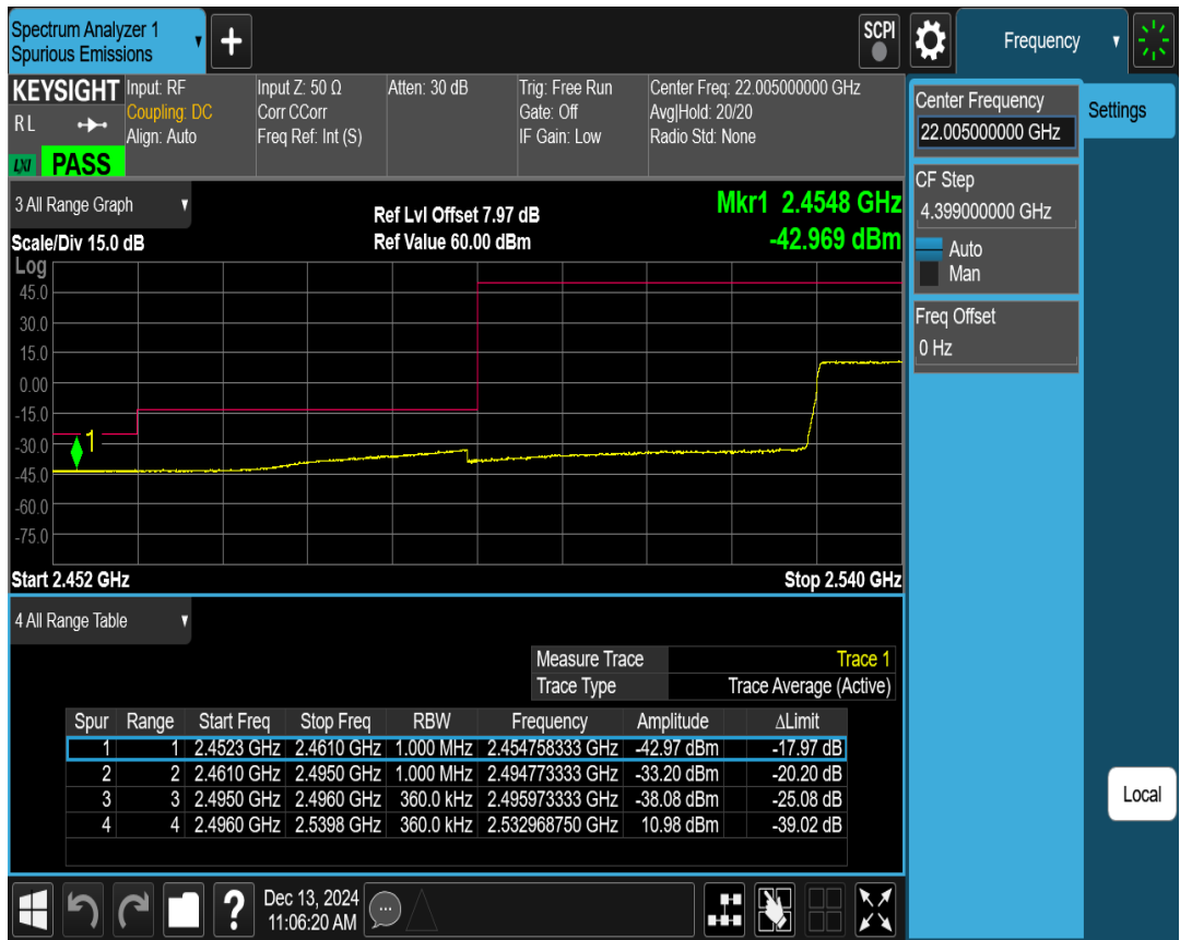
41C QPSK PCC BW=15MHz Ch=41319 RB=1@0,SCC BW=20MHz Ch=41490 RB=1@99
