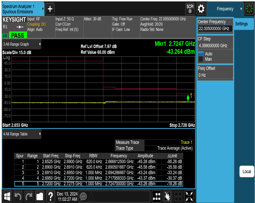
41C 16QAM PCC BW=20MHz Ch=41391 RB=1@0,SCC BW=10MHz Ch=41535 RB=1@49
