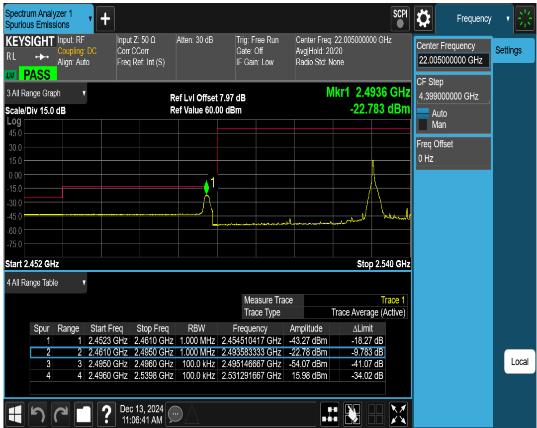
41C 16QAM PCC BW=15MHz Ch=41319 RB=1@0,SCC BW=20MHz Ch=41490 RB=1@99
