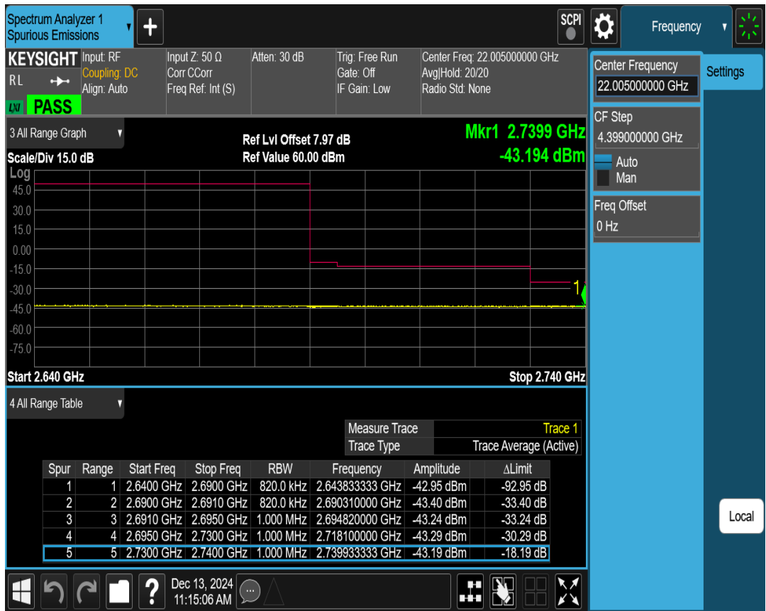
41C 16QAM PCC BW=20MHz Ch=39750 RB=1@0,SCC BW=20MHz Ch=39948 RB=1@99
