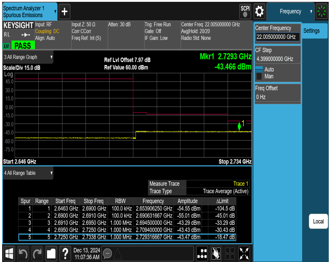
41C QPSK PCC BW=15MHz Ch=41319 RB=75@0,SCC BW=20MHz Ch=41490 RB=100@0
