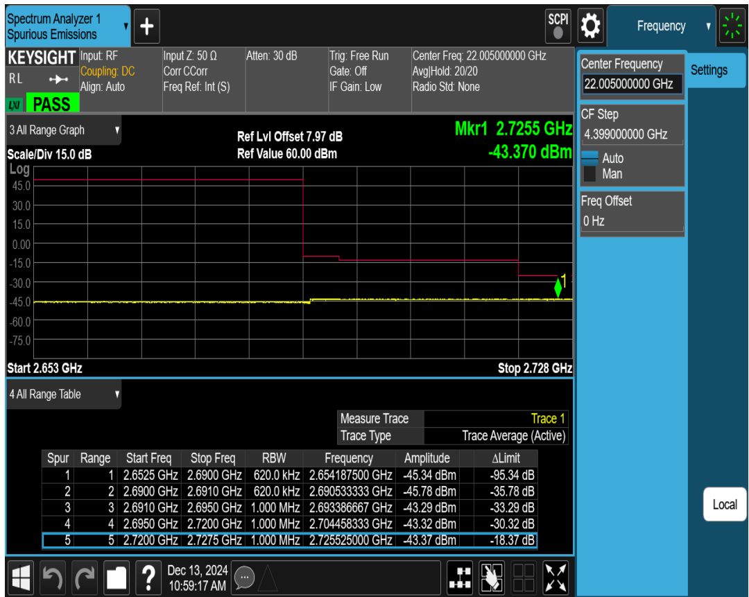
41C 16QAM PCC BW=15MHz Ch=39725 RB=1@0,SCC BW=15MHz Ch=39875 RB=1@74
