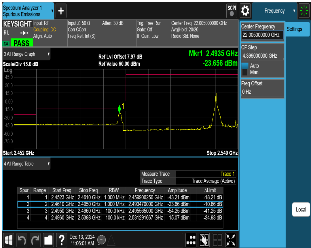
41C QPSK PCC BW=15MHz Ch=39728 RB=75@0,SCC BW=20MHz Ch=39899 RB=100@0
