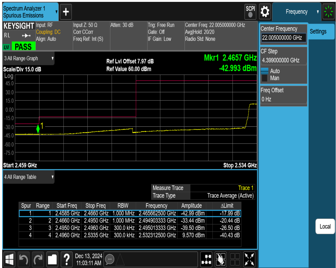
41C QPSK PCC BW=15MHz Ch=39728 RB=1@0,SCC BW=20MHz Ch=39899 RB=1@99
