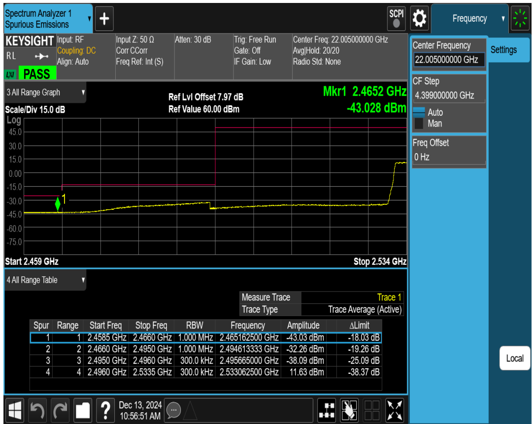
41C QPSK PCC BW=10MHz Ch=41346 RB=1@0,SCC BW=20MHz Ch=41490 RB=1@99
