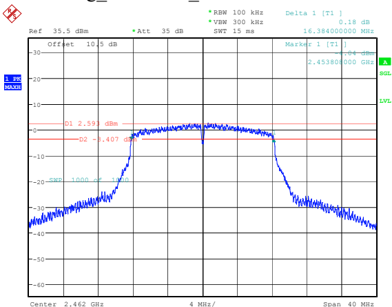
802.11g_2462MHz_Chain 1 16.384MHz
