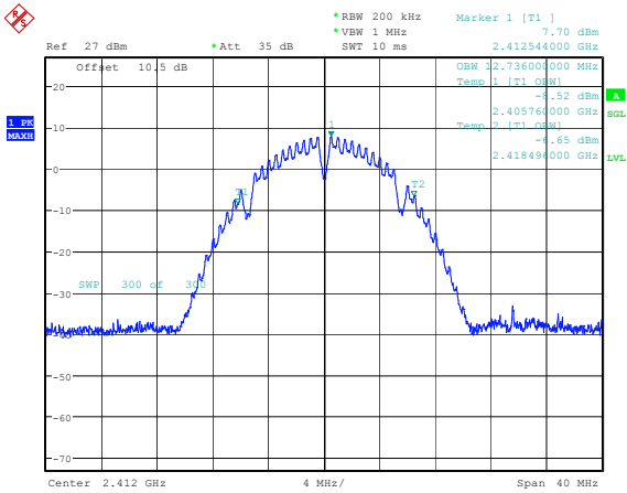
802.11b_2412MHz_Chain 1 12.736MHz
