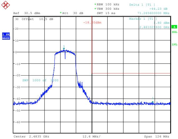
802.11g_2462MHz_Chain 0 44.23dB
