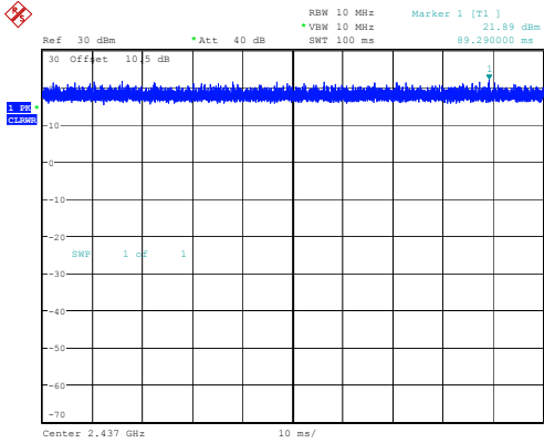
802.11n20_2437MHz_Chain 0 100ms,100ms
