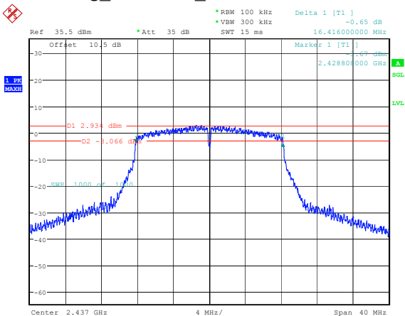
802.11g_2437MHz_Chain 1 16.416MHz
