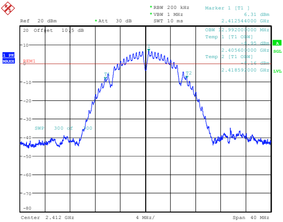
802.11b_2412MHz_Chain 0 12.992MHz
