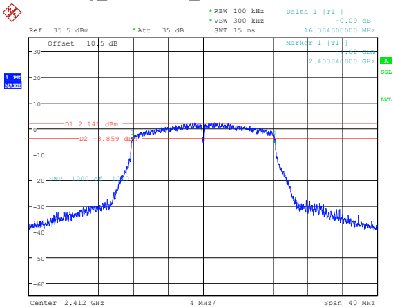
802.11g_2412MHz_Chain 1 16.384MHz
