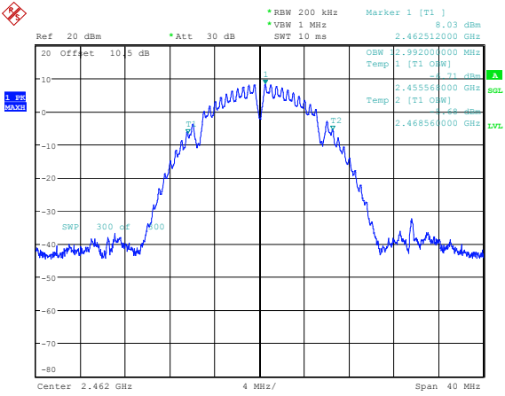
802.11b_2462MHz_Chain 0 12.992MHz
