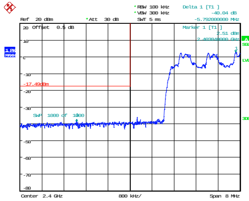
2DH1_Hopping_Lower 40.04dB
