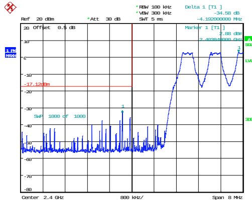
DH1_Hopping_Lower 34.58dB
