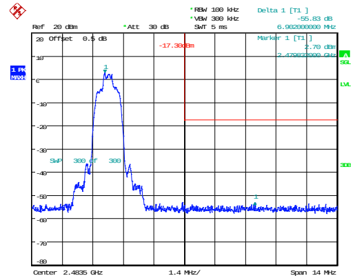
2DH1_High 55.83dB
