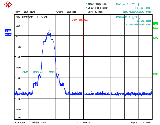
3DH1_High 55.43dB
