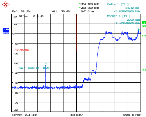
3DH1_Hopping_Lower 34.42dB
