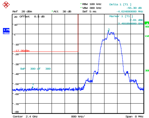
2DH1_Low 55.30dB
