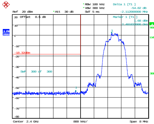
3DH1_Low 54.82dB
