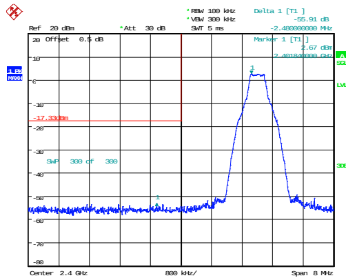
DH1_Low 55.91dB
