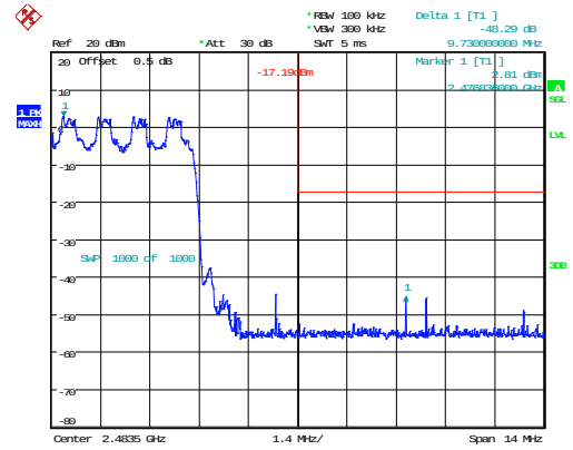
2DH1_Hopping_Upper 48.29dB
