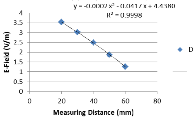
Position D E-Field
