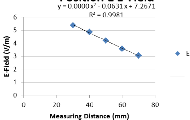
Position E E-Field
