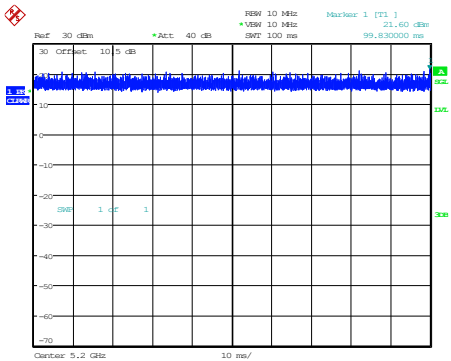
802.11n20_5200MHz 100ms,100ms
