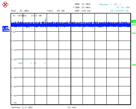
802.11a_5200MHz 100ms,100ms
