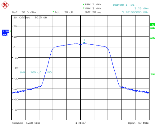
802.11a_5280MHz
