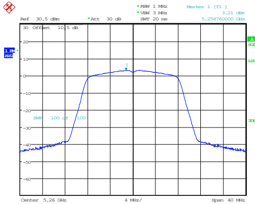
802.11a_5260MHz
