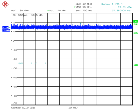
802.11n40_5190MHz 100ms,100ms
