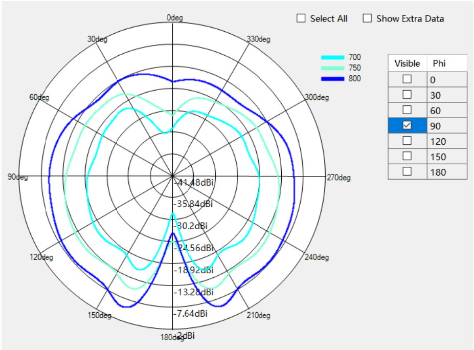
LTE B12/17/28 Phi=90deg
