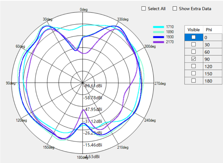
DCS1800/PCS1900/WCDMA B1/B2/B4/LTE B1/2/3/4Phi=90deg
