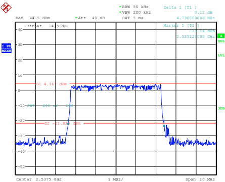
26dB Bandwidth
