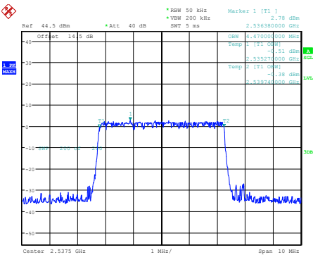
Occupied Bandwidth
