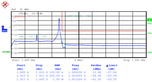
15MHz_High_16QAM_1@74
