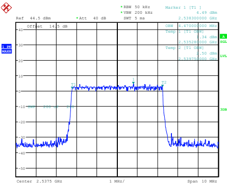
Occupied Bandwidth
