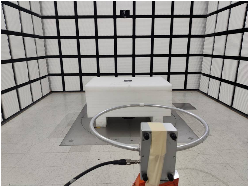
Radiated Emission Below 30MHz View Ground-parallel-2CII-6
