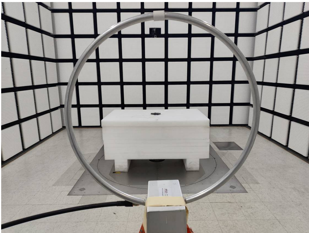
Radiated Emission Below 30MHz View Parallel-2CII-5
