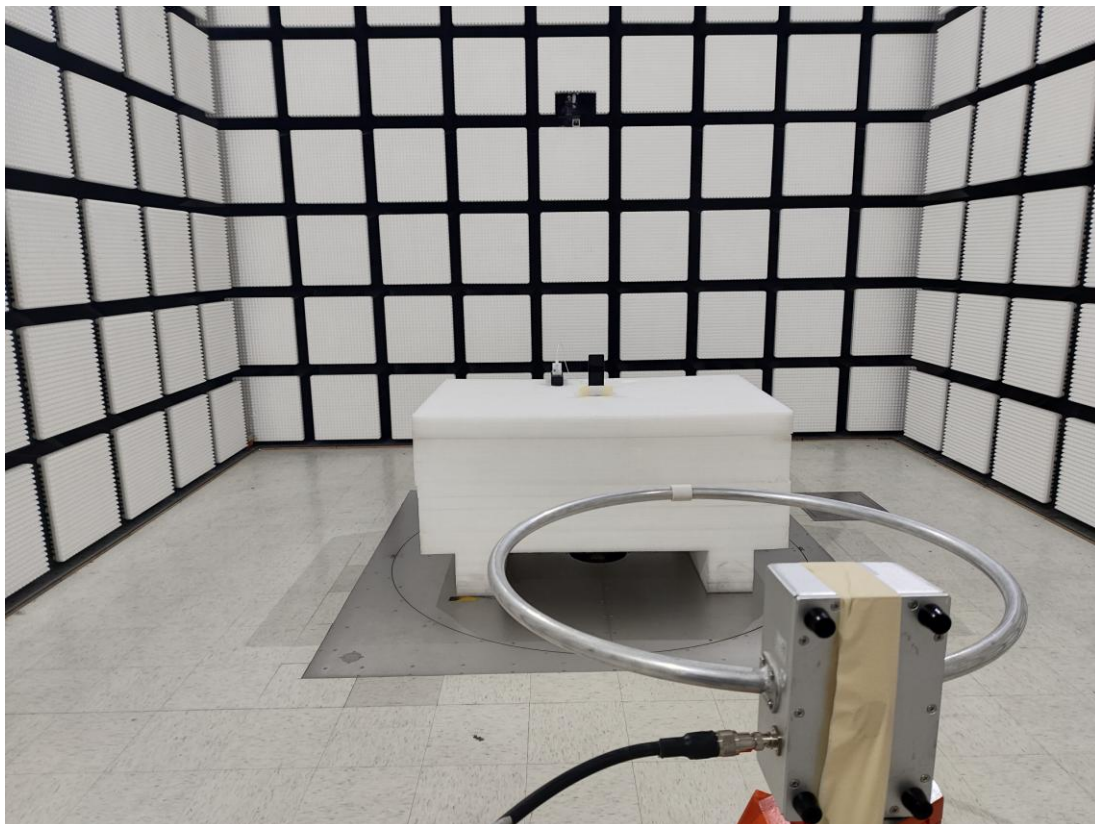
Radiated Emission Below 30MHz View Ground-parallel-2CIH-5
