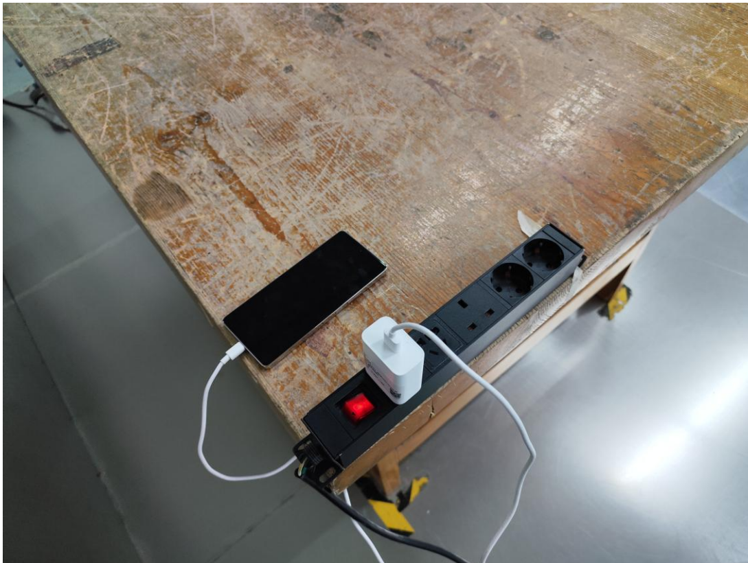
Conducted Emissions Side View-2CIH-5
