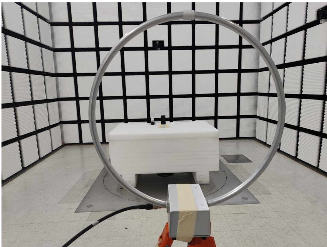
Radiated Emission Below 30MHz View Parallel-2CIH-6
