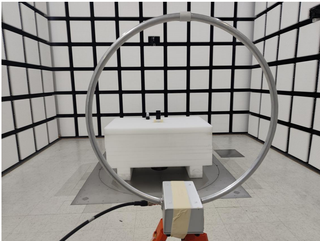
Radiated Emission Below 30MHz View Parallel-2CIH-5
