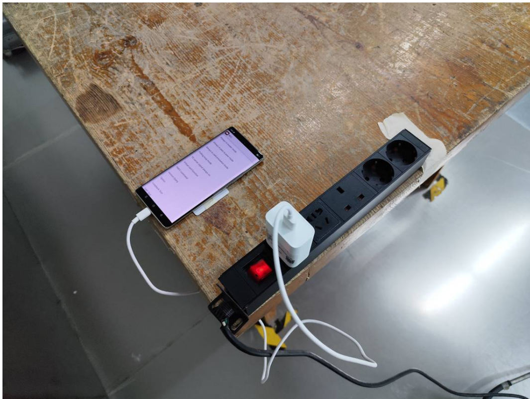
Conducted Emissions Side View- (Lighting Version &Adapter #1)
