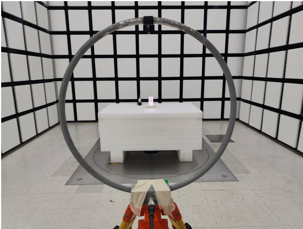
Radiated Emission Below 30MHz View Perpendicular- (Normal Version &Adapter #1)
