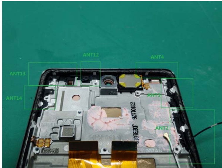
ANT4:WWAN Antenna,another Antenna: receiving only or no use
