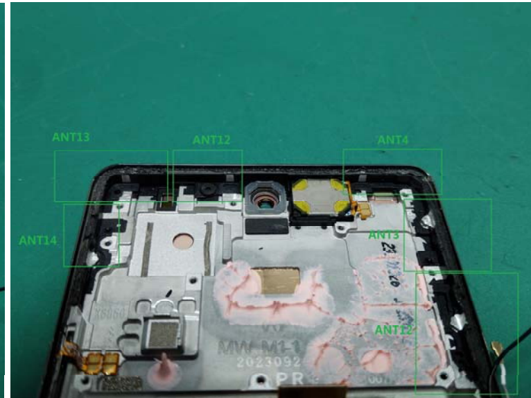
NT4:WWAN Antenna,another Antenna: receiving only or no use
