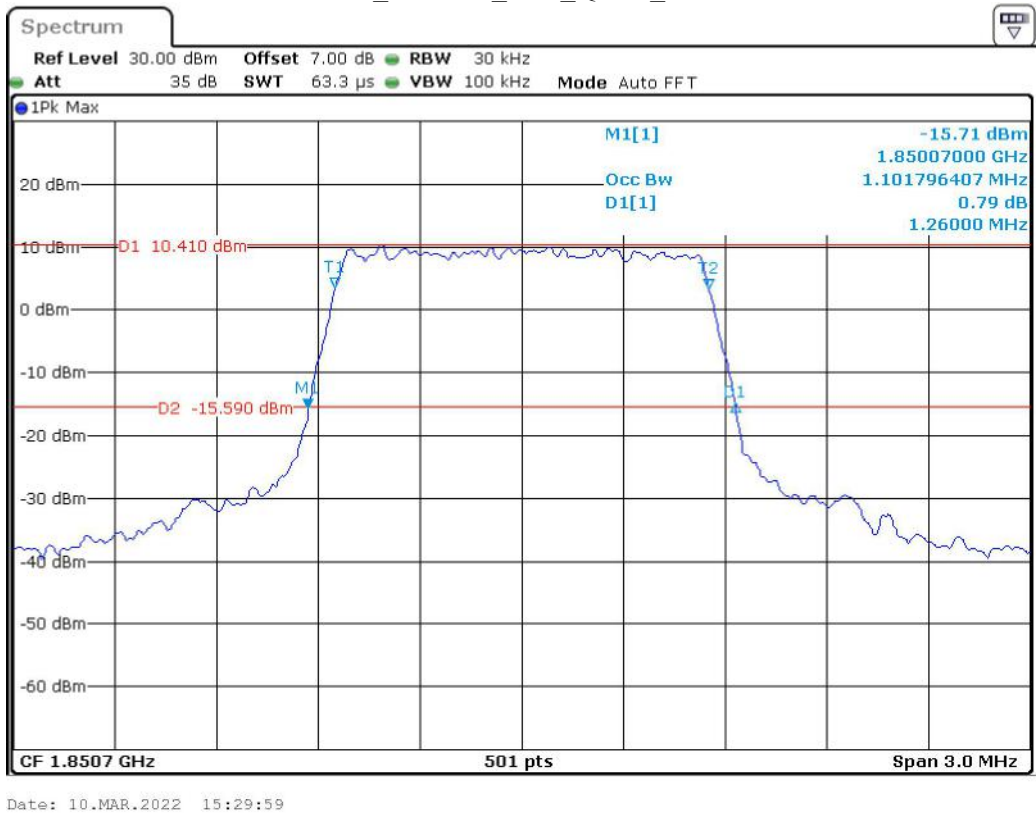
Band 2_1.4 MHz_Low_QPSK_RB6#0
