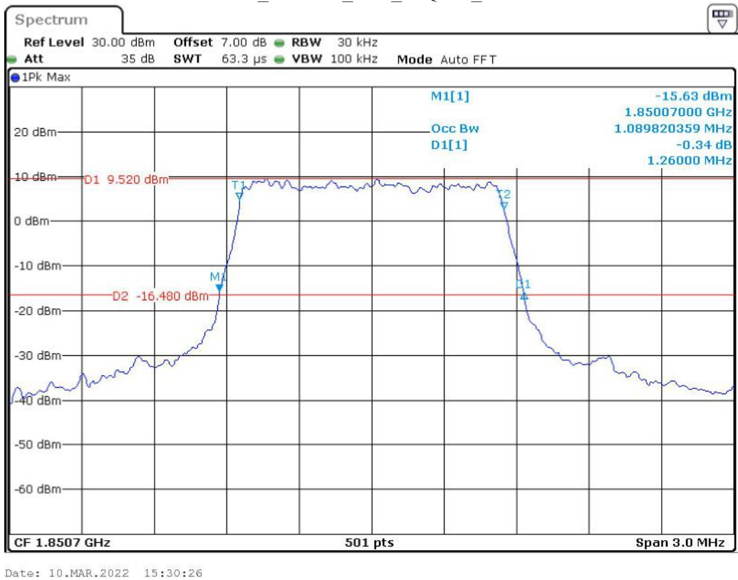
Band 2_1.4 MHz_Low_16QAM_RB6#0
