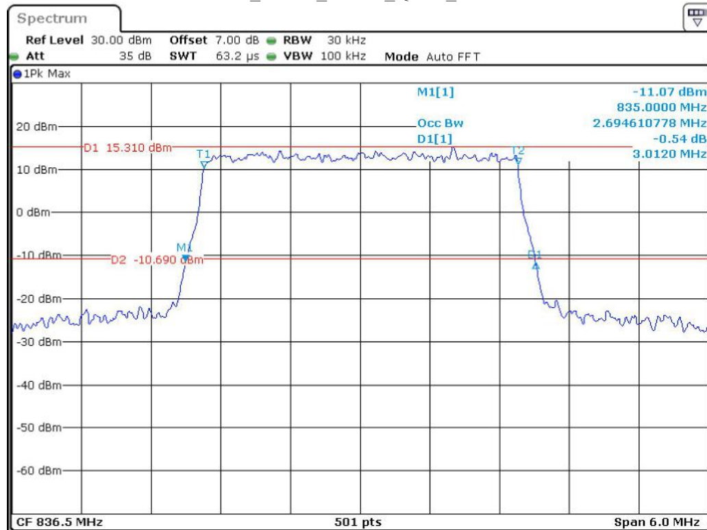
Band 5_3 MHz_Middle_QPSK_RB15#0
