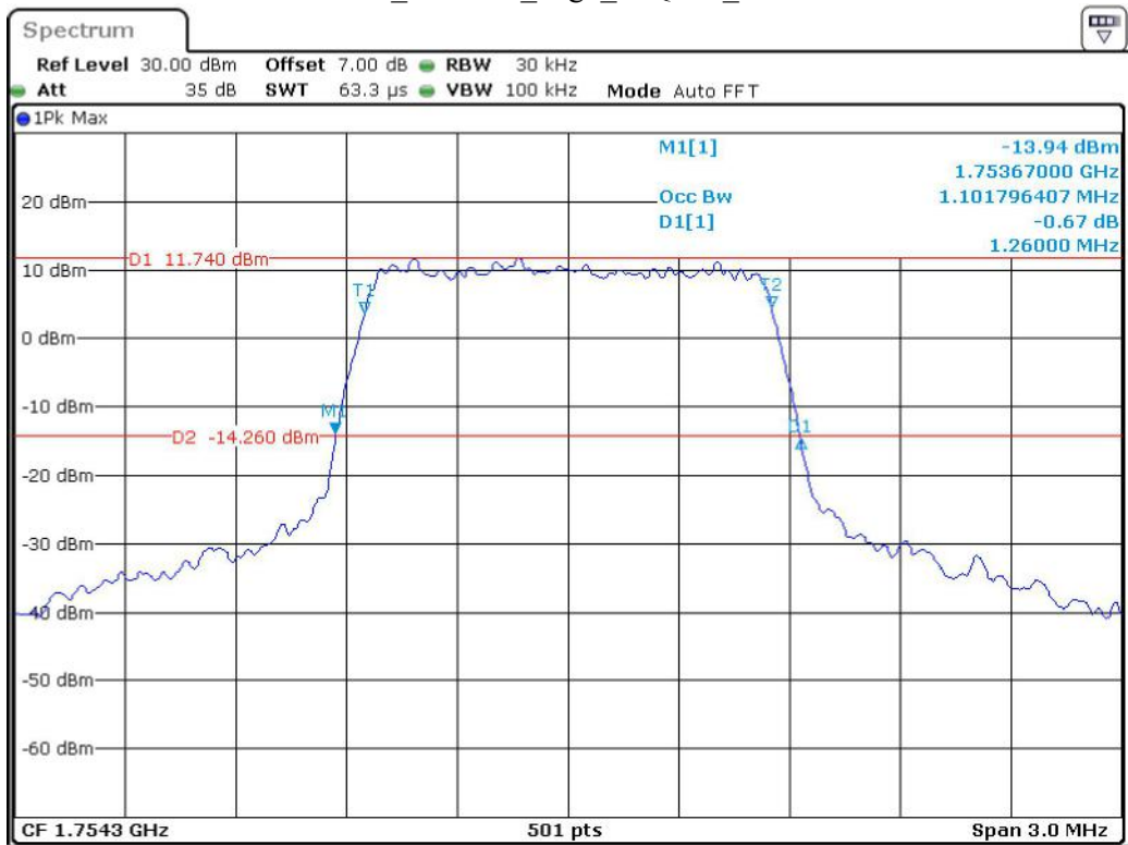
Band 4_1.4 MHz_High_16QAM_RB6#0
