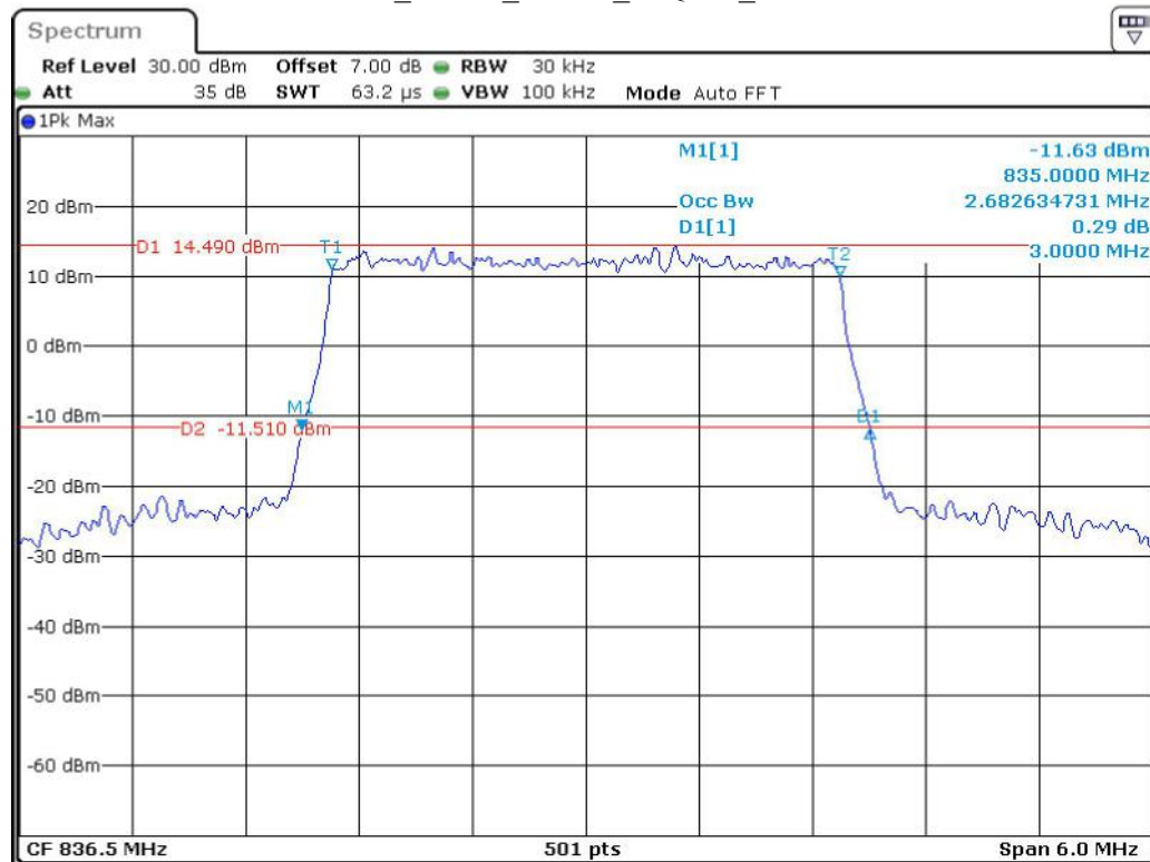
Band 5_3 MHz_Middle_16QAM_RB15#0
