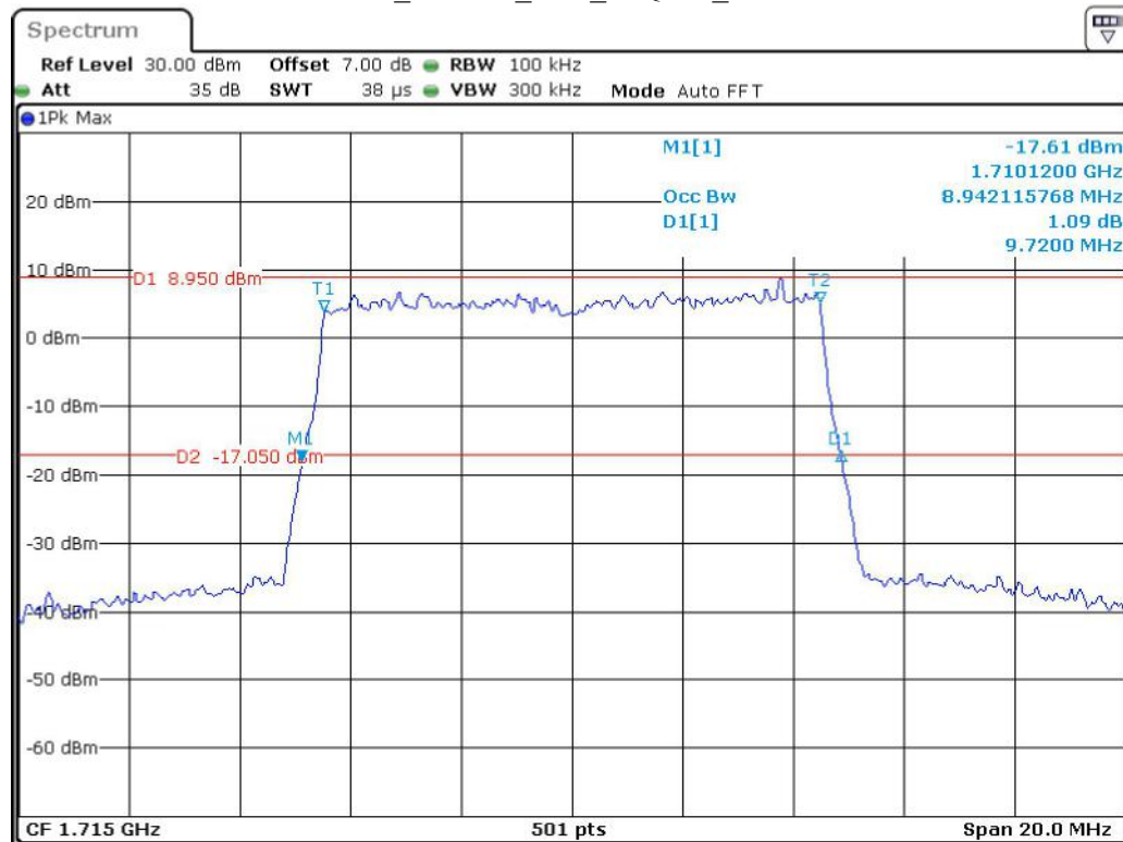
Band 4_10 MHz_Low_16QAM_RB50#0
