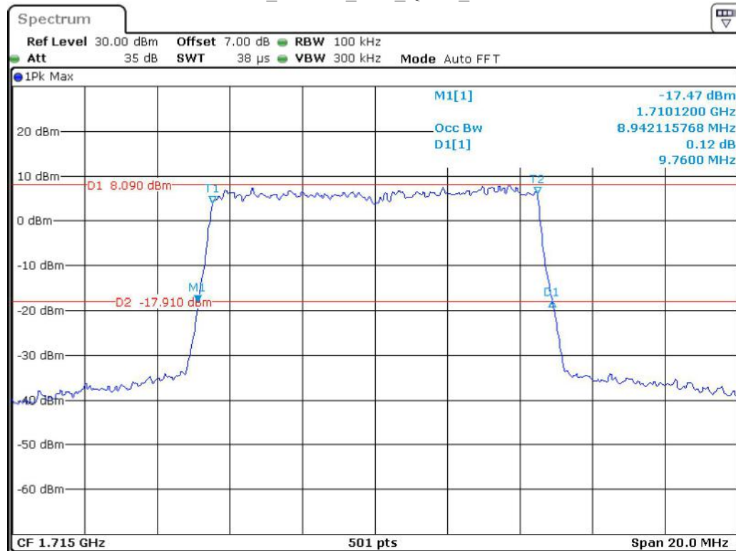
Band 4_10 MHz_Low_QPSK_RB50#0
