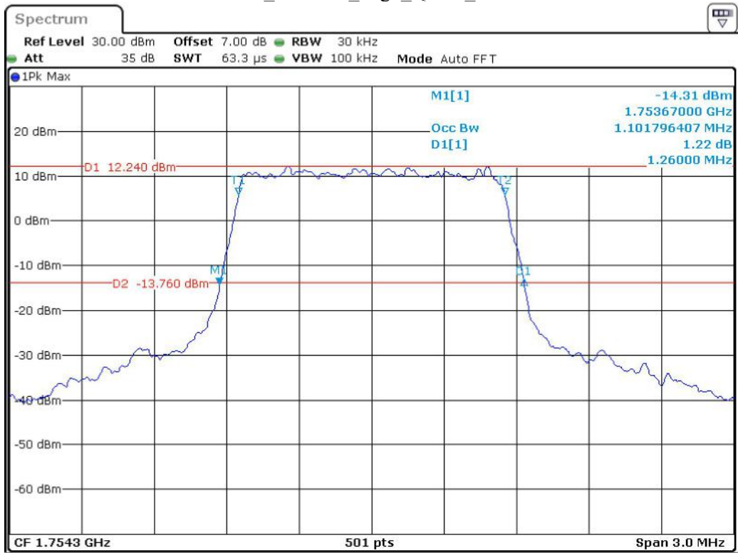
Band 4_1.4 MHz_High_QPSK_RB6#0
