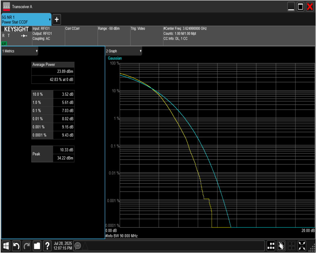
n78(3550-3700) SCS=30kHz DFT_QAM64 BW=90MHz Channel=643666 RB=240@0
