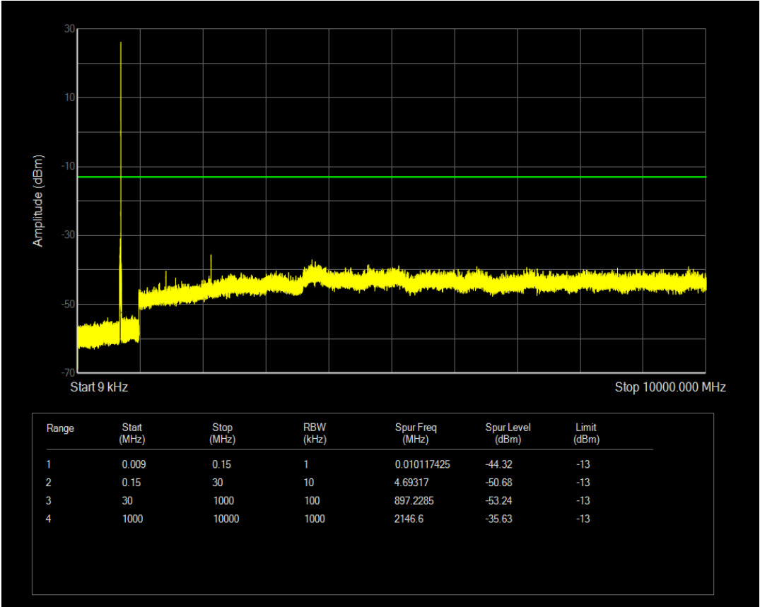
n12 SCS=15kHz CP_QPSK BW=15MHz Channel=141300 RB=1@78
