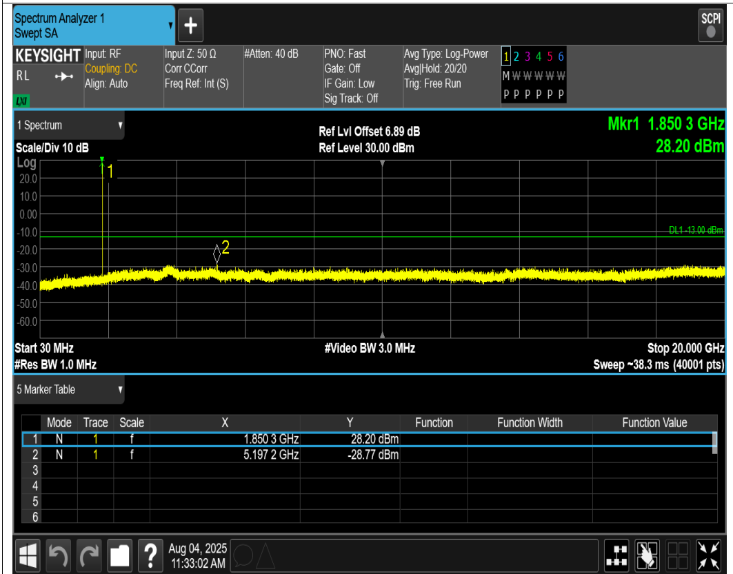
GSM1900 Channel=512
