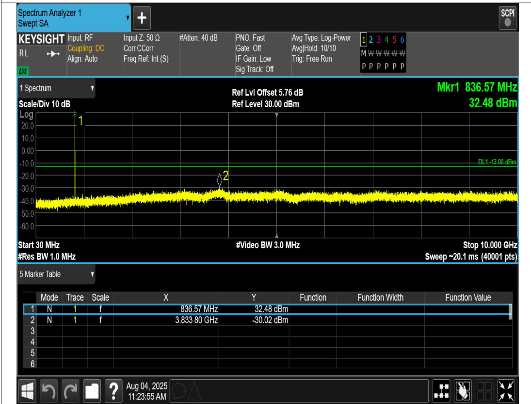
GSM850 Channel=190
