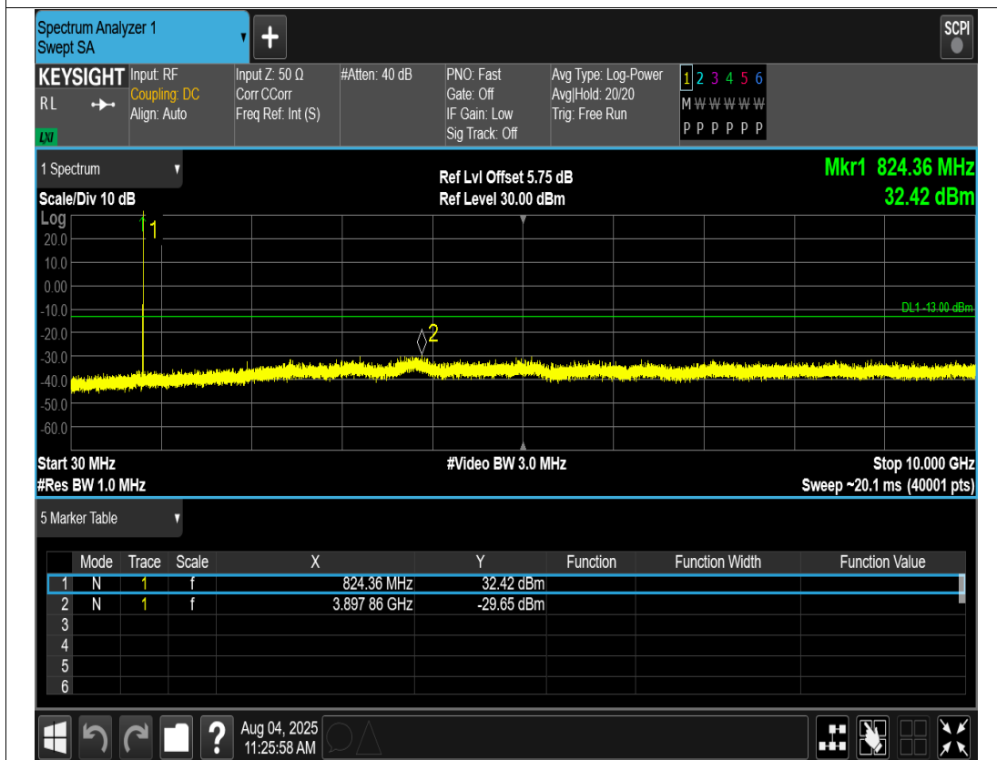
GPRS850 Channel=128
