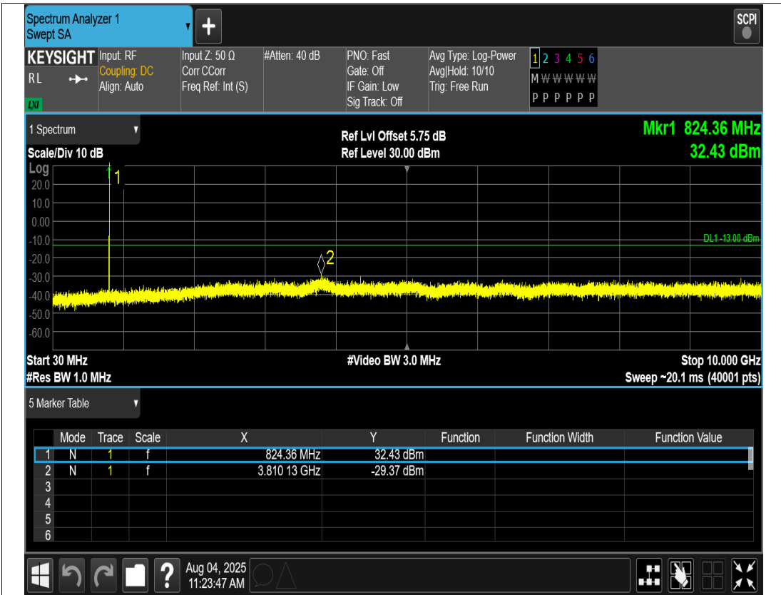
GSM850 Channel=128
