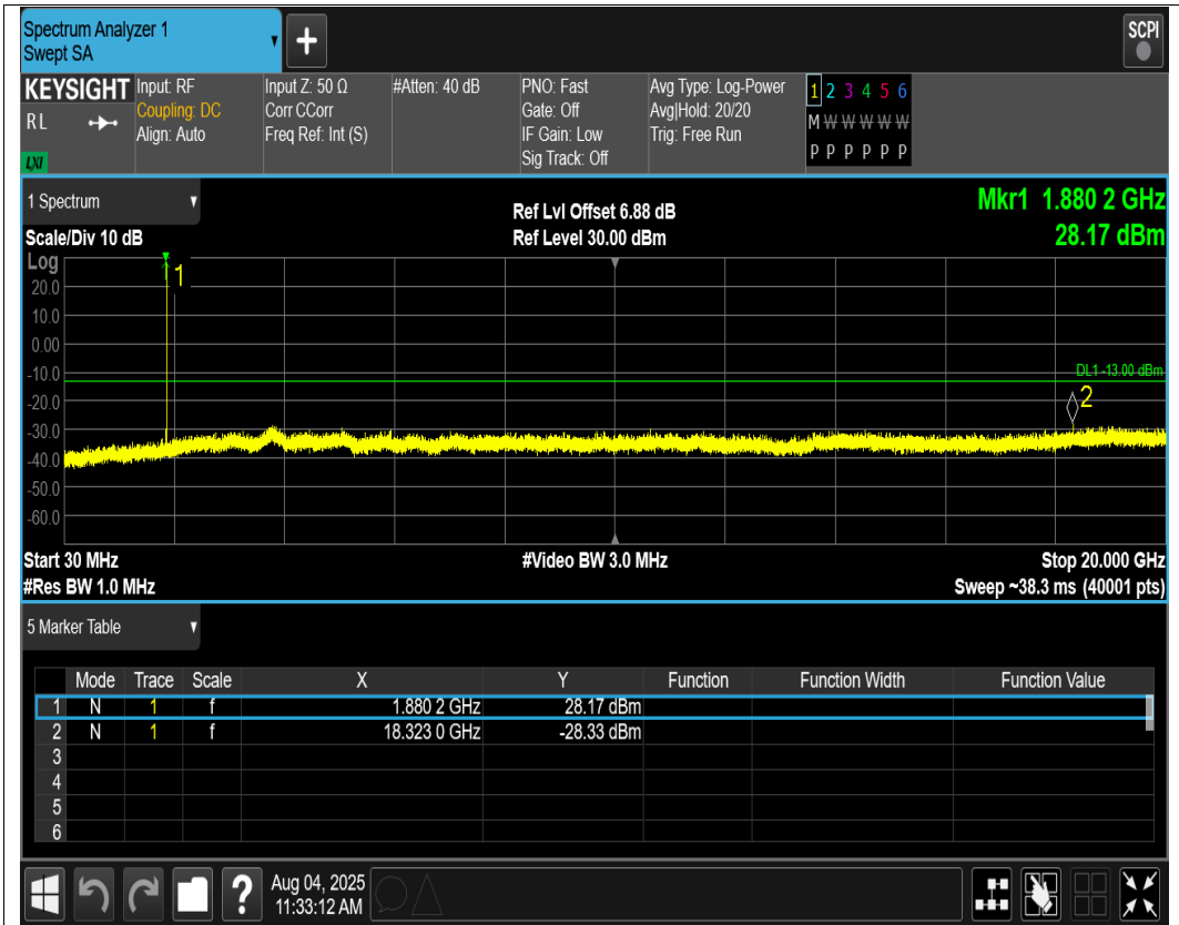
GSM1900 Channel=661
