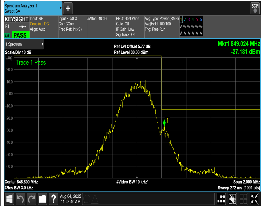
GSM850 Channel=251
