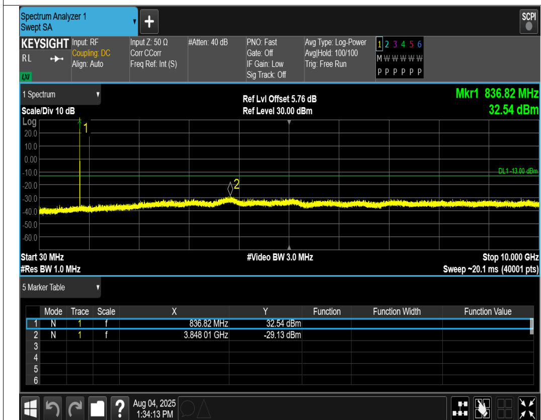
EGPRS850 Channel=190
