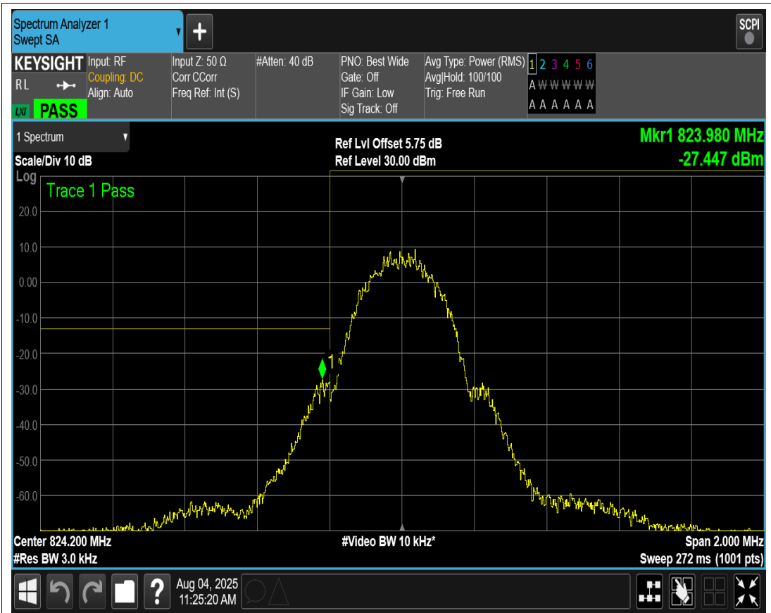
GPRS850 Channel=128
