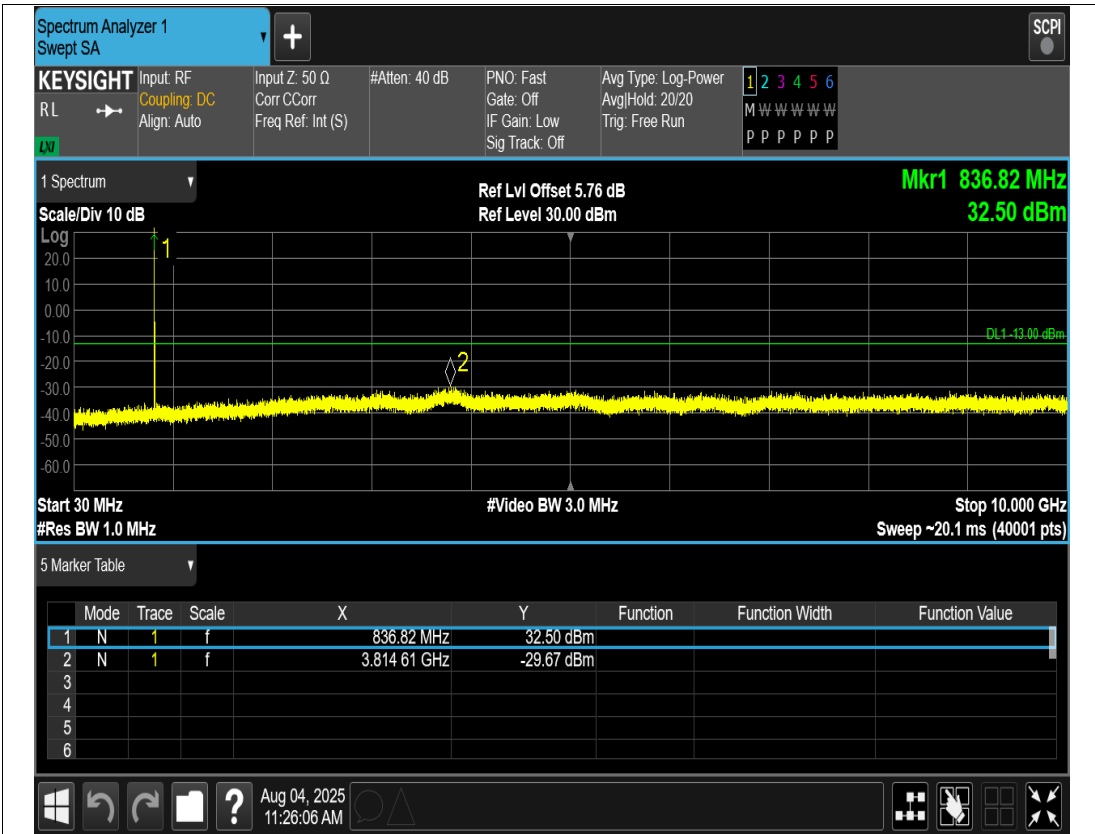
GPRS850 Channel=190
