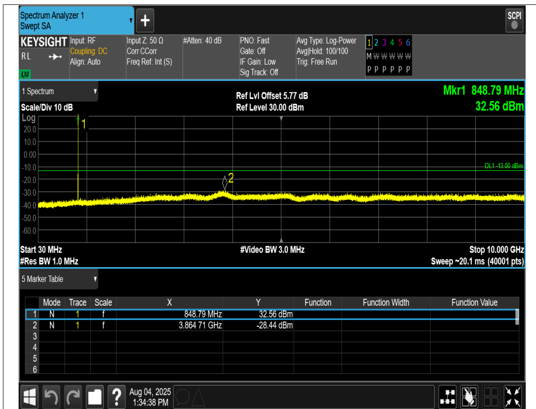
EGPRS850 Channel=251
