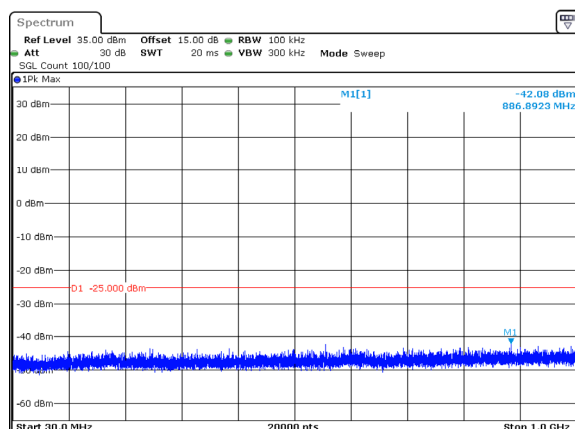
B7_2525.1MHz_Middle_20M_1@99_QPSK B7_2544.9MHz_Middle_20M_1@0_QPSK (30MHz~1GHz)
