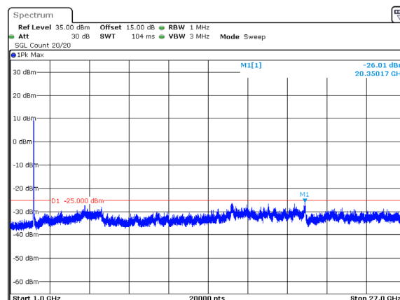
B7_2510MHz_Low_20M_100@0_16QAM B7_2529.8MHz_Low_20M_100@0_16QAM (1GHz~27GHz)
