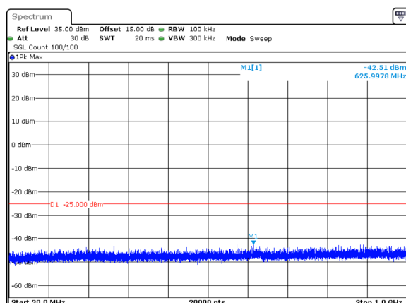
B7_2525.1MHz_Middle_20M_100@0_QPSK B7_2544.9MHz_Middle_20M_100@0_QPSK (30MHz~1GHz)
