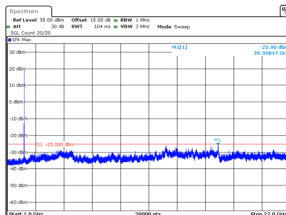
B7_2525.1MHz_Middle_20M_1@99_QPSK B7_2544.9MHz_Middle_20M_1@0_QPSK (1GHz~27GHz)
