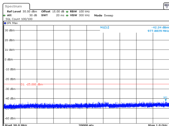
B7_2510MHz_Low_20M_100@0_16QAM B7_2529.8MHz_Low_20M_100@0_16QAM (30MHz~1GHz)
