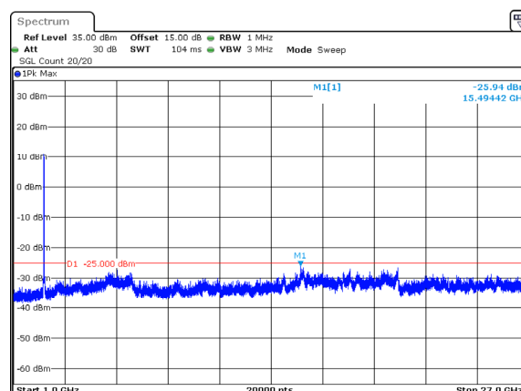
B7_2525.1MHz_Middle_20M_100@0_QPSK B7_2544.9MHz_Middle_20M_100@0_QPSK (1GHz~27GHz)
