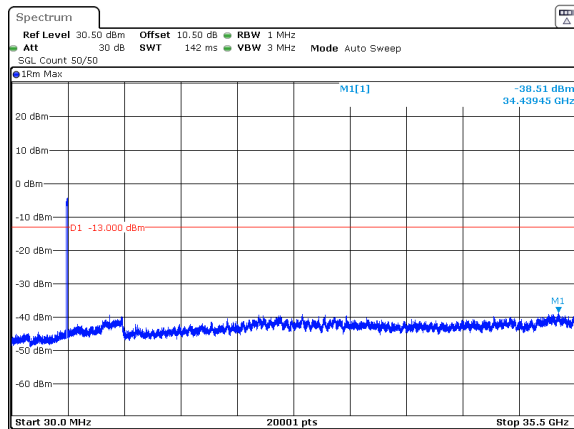
n78_1_80MHz_30kHz_3500MHz_DFT-s-OFDM QPSK_RB216@0 -38.51dBm
