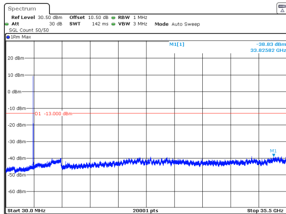
n78_1_80MHz_30kHz_3500MHz_DFT-s-OFDM QPSK_RB1@0 -38.83dBm
