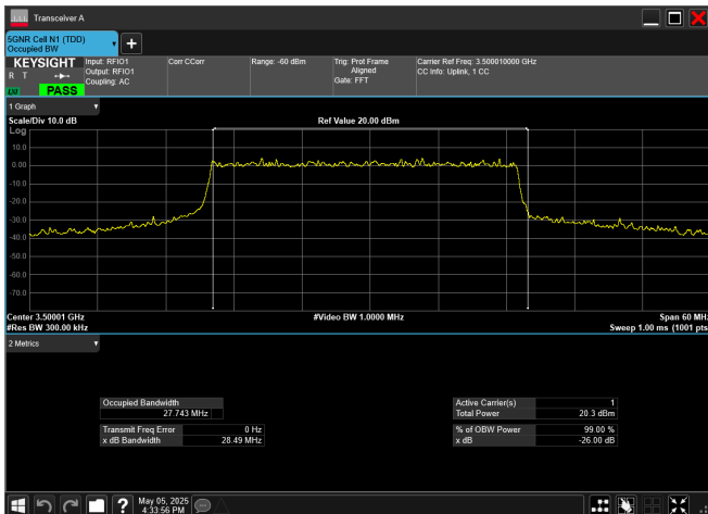
n78_1_30MHz_30kHz_3500MHz_DFT-s-OFDM 256 QAM_RB75@0
