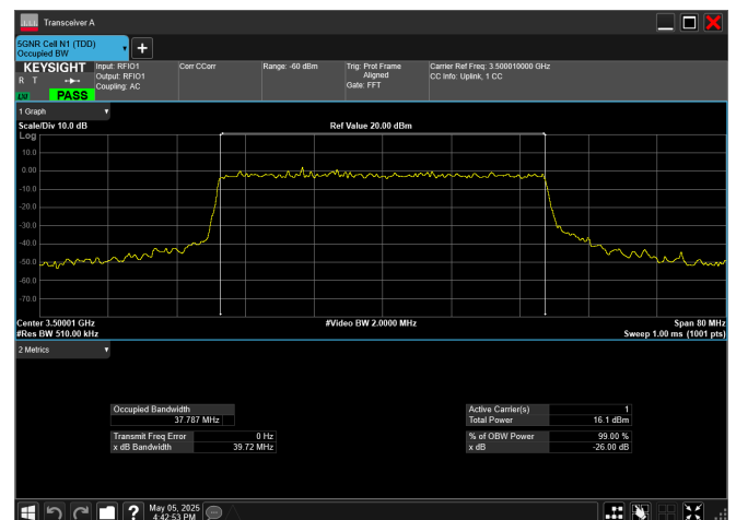
n78_1_40MHz_30kHz_3500MHz_CP-OFDM 256 QAM_RB106@0
