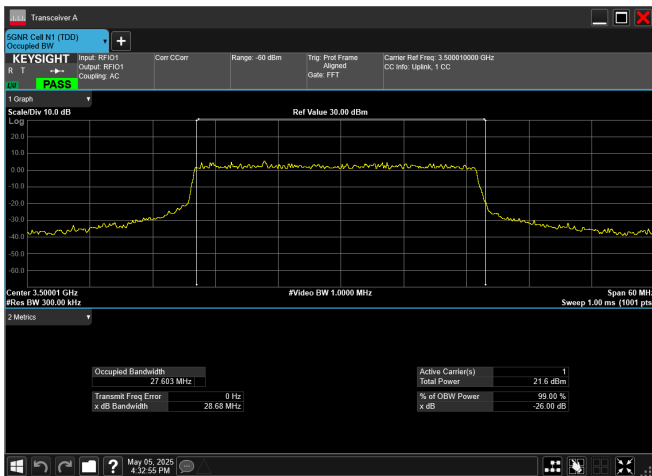
n78_1_30MHz_30kHz_3500MHz_DFT-s-OFDM 16 QAM_RB75@0
