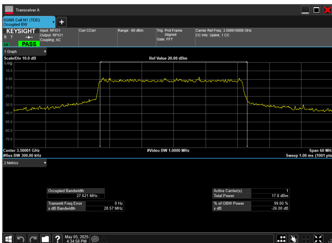
n78_1_30MHz_30kHz_3500MHz_DFT-s-OFDM 256 QAM_RB75@0
