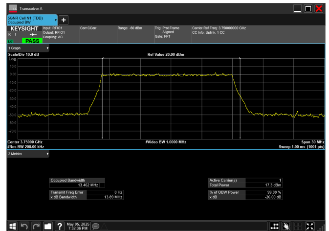
n78_3_15MHz_30kHz_3750MHz_CP-OFDM 16 QAM_RB38@0
