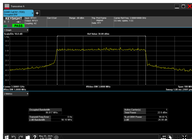
n78_1_90MHz_30kHz_3500MHz_DFT-s-OFDM 64 QAM_RB243@0
