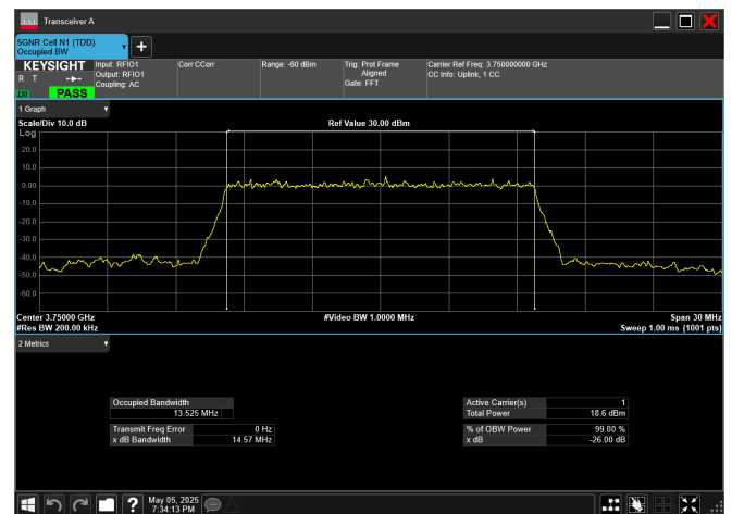
n78_3_15MHz_30kHz_3750MHz_CP-OFDM 256 QAM_RB38@0
