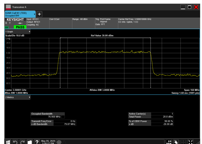
n78_1_80MHz_30kHz_3500MHz_DFT-s-OFDM 16 QAM_RB216@0
