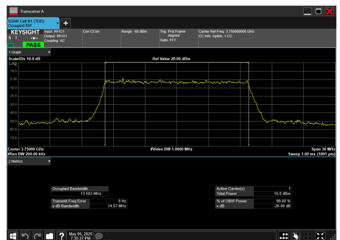
n78_3_15MHz_30kHz_3750MHz_CP-OFDM 256 QAM_RB38@0
