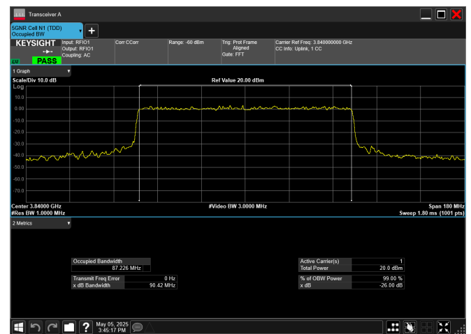
n77_3_90MHz_30kHz_3840MHz_CP-OFDM 256 QAM_RB245@0
