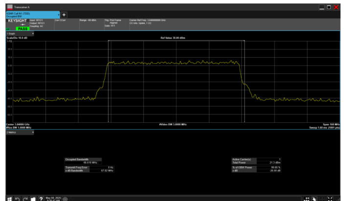
n77_3_70MHz_30kHz_3840MHz_DFT-s-OFDM 16 QAM_RB180@0
