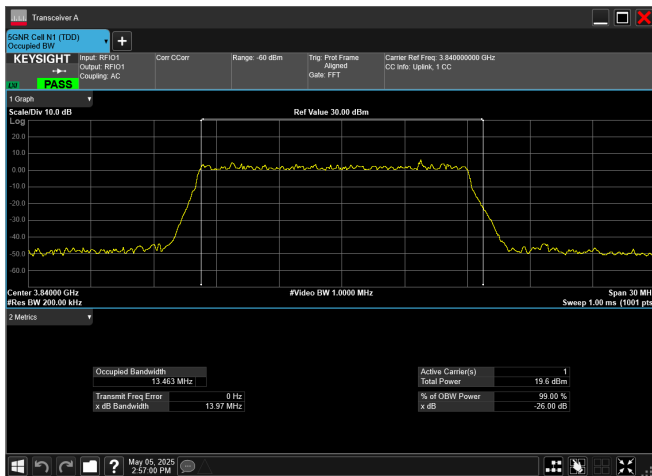
n77_3_15MHz_30kHz_3840MHz_CP-OFDM QPSK_RB38@0
