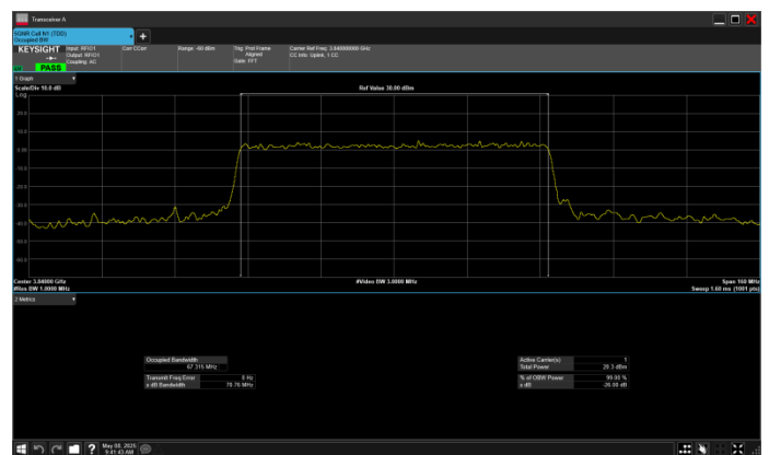
n77_3_70MHz_30kHz_3840MHz_CP-OFDM 256 QAM_RB189@0
