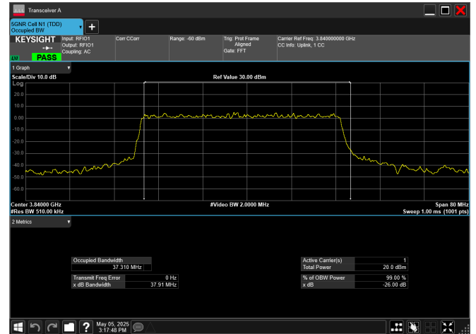
n77_3_40MHz_30kHz_3840MHz_DFT-s-OFDM 64 QAM_RB100@0
