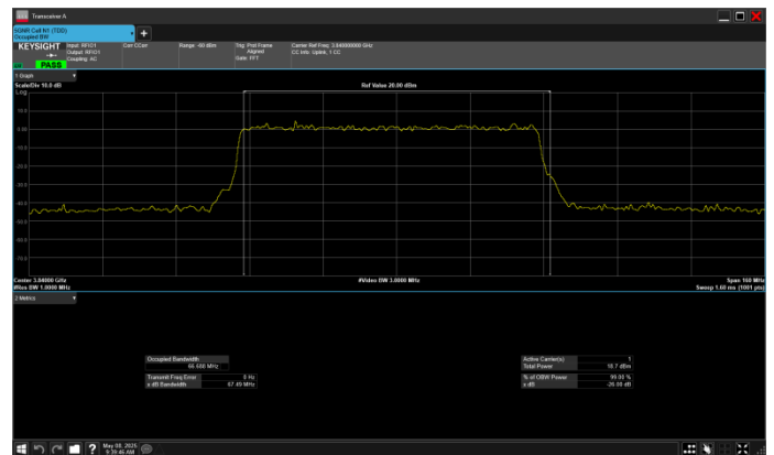
n77_3_70MHz_30kHz_3840MHz_CP-OFDM 16 QAM_RB189@0
