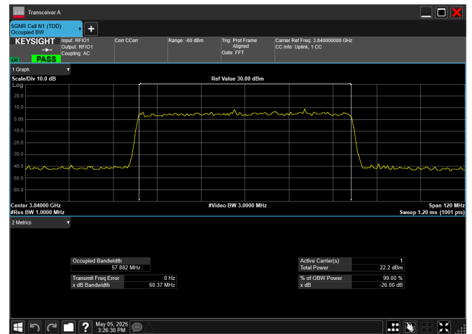
n77_3_60MHz_30kHz_3840MHz_DFT-s-OFDM 64 QAM_RB162@0
