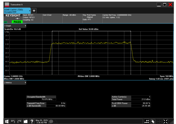
n77_3_80MHz_30kHz_3840MHz_DFT-s-OFDM 64 QAM_RB216@0
