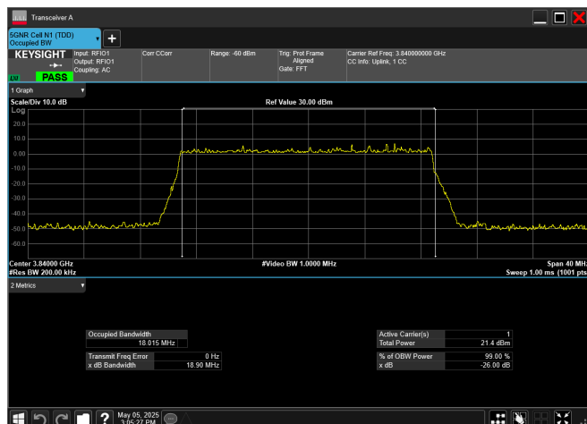
n77_3_20MHz_30kHz_3840MHz_DFT-s-OFDM 16 QAM_RB50@0
