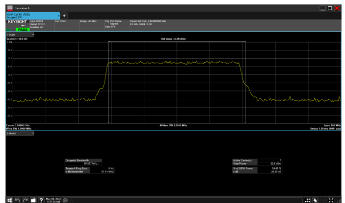
n77_3_70MHz_30kHz_3840MHz_DFT-s-OFDM 16 QAM_RB180@0
