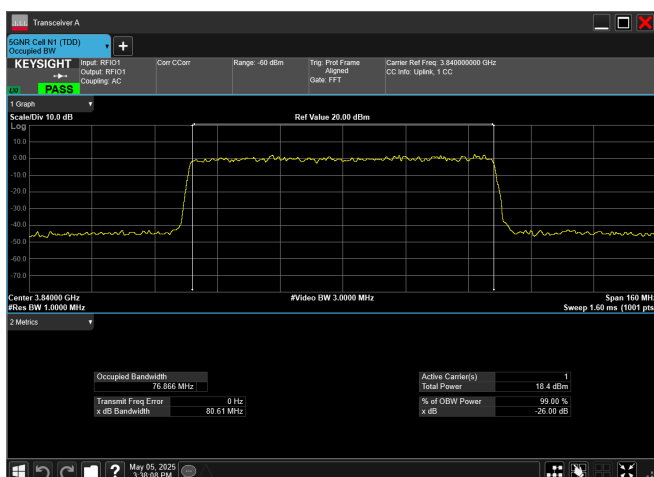
n77_3_80MHz_30kHz_3840MHz_DFT-s-OFDM 256 QAM_RB216@0
