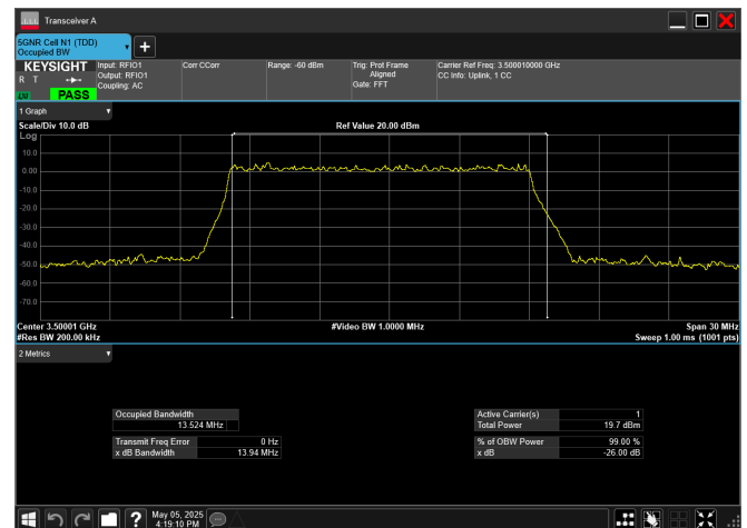
n78_1_15MHz_30kHz_3500MHz_DFT-s-OFDM 64 QAM_RB36@0
