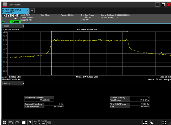
n77_3_30MHz_30kHz_3840MHz_CP-OFDM 64 QAM_RB78@0
