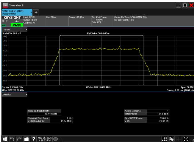
n78_1_15MHz_30kHz_3500MHz_DFT-s-OFDM 16 QAM_RB36@0
