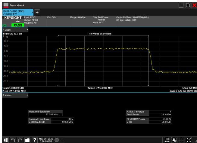
n77_3_60MHz_30kHz_3840MHz_DFT-s-OFDM 16 QAM_RB162@0
