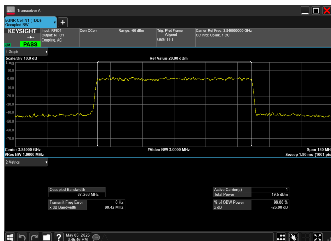
n77_3_90MHz_30kHz_3840MHz_CP-OFDM 64 QAM_RB245@0
