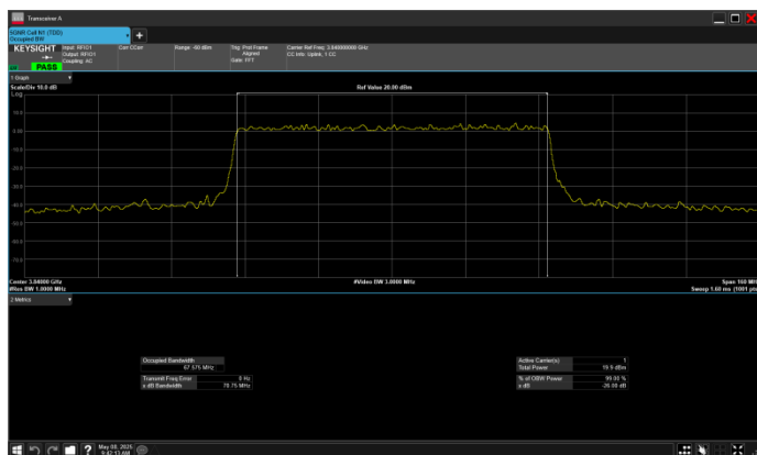
n77_3_70MHz_30kHz_3840MHz_CP-OFDM 64 QAM_RB189@0
