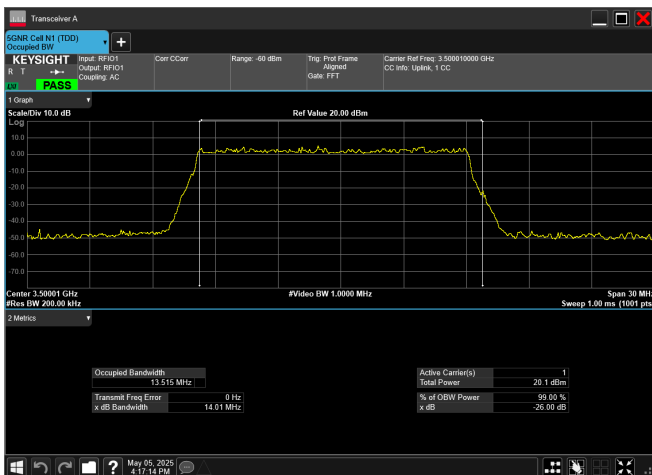
n78_1_15MHz_30kHz_3500MHz_DFT-s-OFDM 256 QAM_RB36@0
