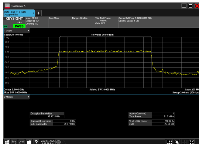
n77_3_100MHz_30kHz_3840MHz_DFT-s-OFDM 64 QAM_RB270@0
