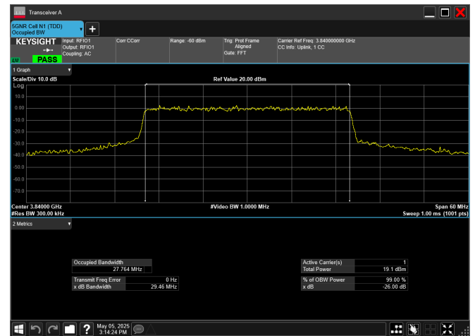
n77_3_30MHz_30kHz_3840MHz_CP-OFDM 256 QAM_RB78@0
