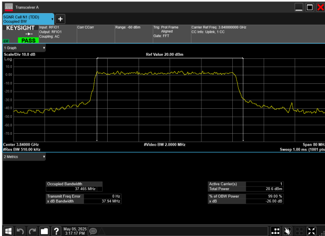
n77_3_40MHz_30kHz_3840MHz_DFT-s-OFDM 256 QAM_RB100@0
