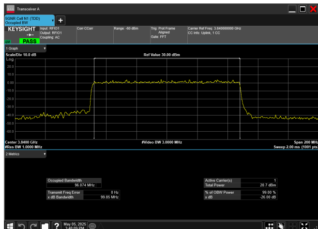
n77_3_100MHz_30kHz_3840MHz_DFT-s-OFDM 256 QAM_RB270@0
