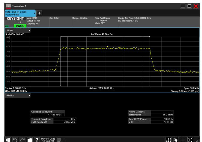
n77_3_50MHz_30kHz_3840MHz_CP-OFDM 256 QAM_RB133@0
