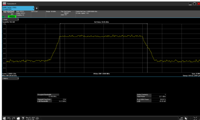
n77_1_15MHz_30kHz_3500MHz_DFT-s-OFDM 16 QAM_RB36@0
