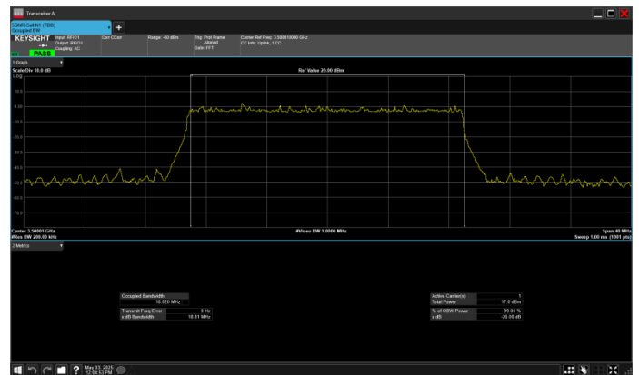
n77_1_20MHz_30kHz_3500MHz_CP-OFDM 16 QAM_RB51@0
