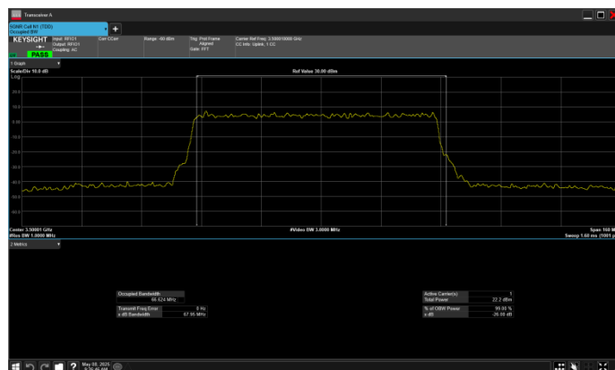
n77_1_70MHz_30kHz_3500MHz_DFT-s-OFDM 64 QAM_RB180@0
