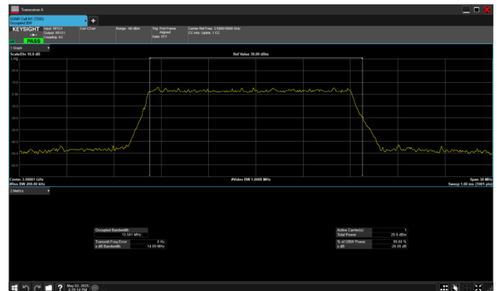
n77_1_15MHz_30kHz_3500MHz_DFT-s-OFDM 64 QAM_RB36@0
