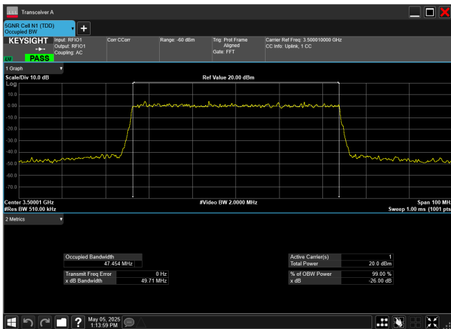
n77_1_50MHz_30kHz_3500MHz_CP-OFDM 256 QAM_RB133@0
