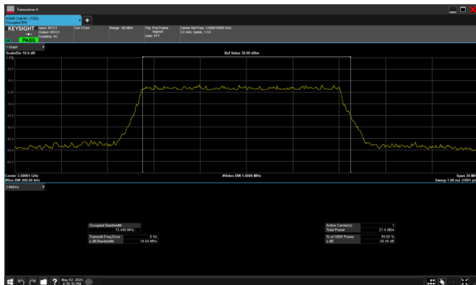
n77_1_15MHz_30kHz_3500MHz_DFT-s-OFDM 256 QAM_RB36@0
