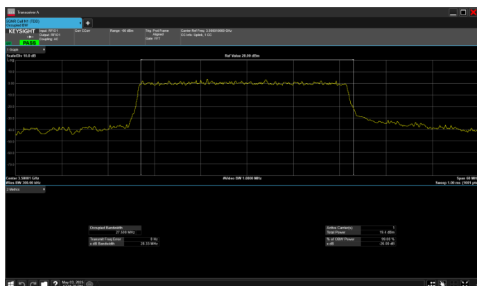
n77_1_30MHz_30kHz_3500MHz_DFT-s-OFDM 256 QAM_RB75@0
