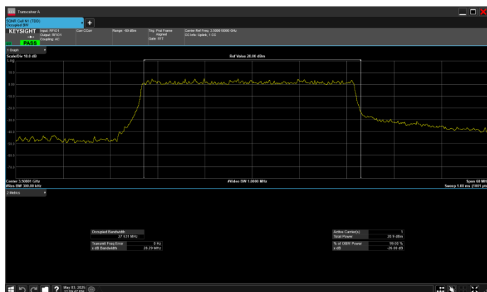
n77_1_30MHz_30kHz_3500MHz_DFT-s-OFDM 16 QAM_RB75@0
