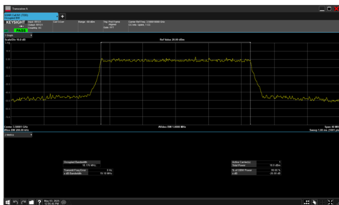
n77_1_20MHz_30kHz_3500MHz_CP-OFDM 64 QAM_RB51@0
