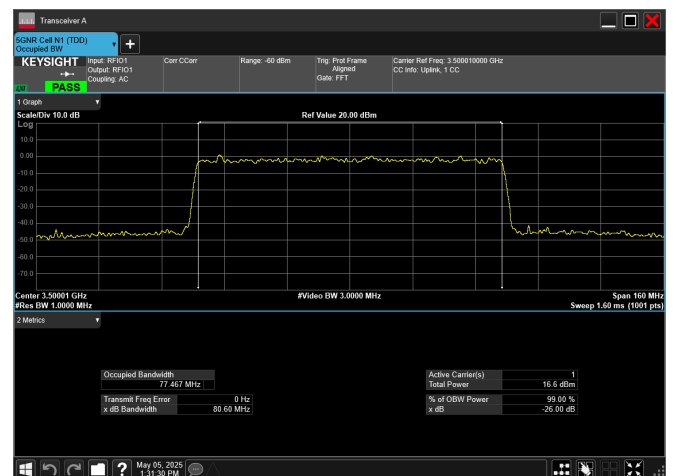
n77_1_80MHz_30kHz_3500MHz_CP-OFDM 256 QAM_RB217@0
