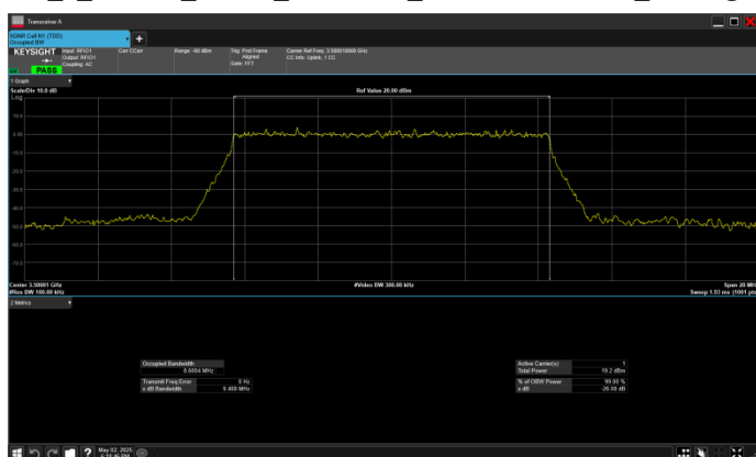
n77_1_10MHz_30kHz_3500MHz_CP-OFDM 64 QAM_RB24@0
