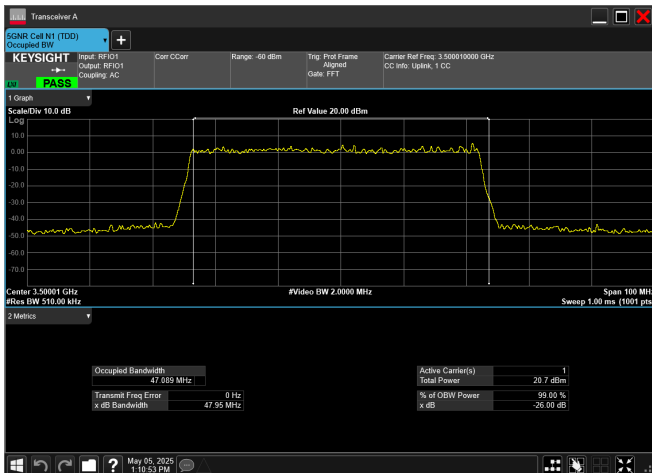
n77_1_50MHz_30kHz_3500MHz_DFT-s-OFDM 256 QAM_RB128@0
