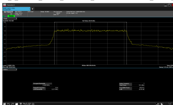
n77_1_10MHz_30kHz_3500MHz_CP-OFDM 256 QAM_RB24@0
