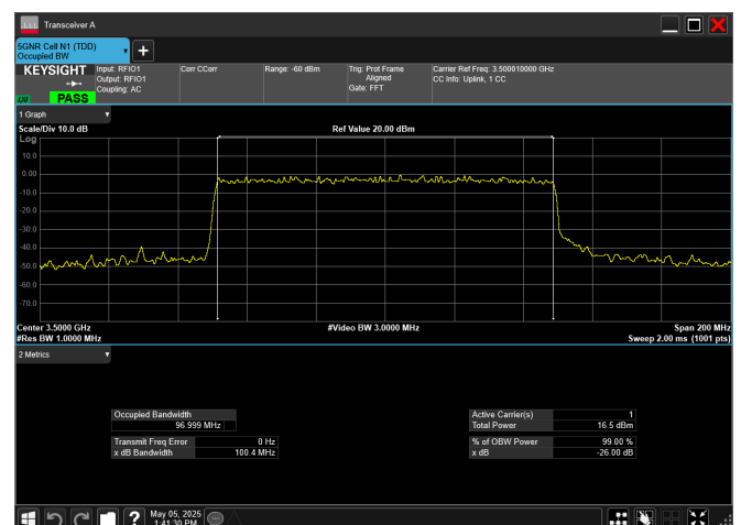
n77_1_100MHz_30kHz_3500MHz_CP-OFDM 256 QAM_RB273@0
