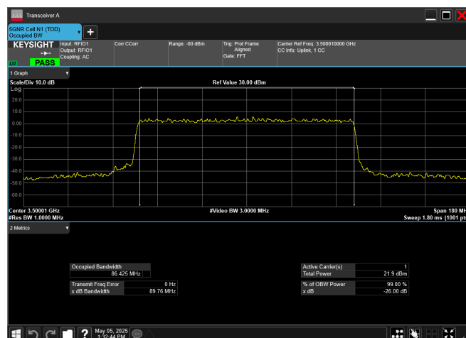
n77_1_90MHz_30kHz_3500MHz_DFT-s-OFDM 64 QAM_RB243@0
