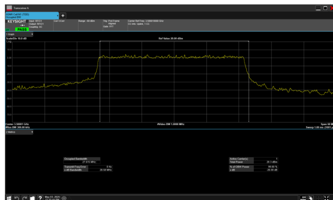
n77_1_30MHz_30kHz_3500MHz_DFT-s-OFDM 64 QAM_RB75@0
