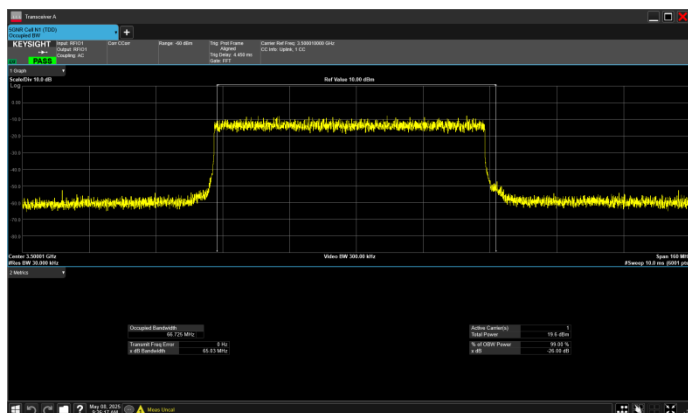
n77_1_70MHz_30kHz_3500MHz_DFT-s-OFDM 16 QAM_RB180@0
