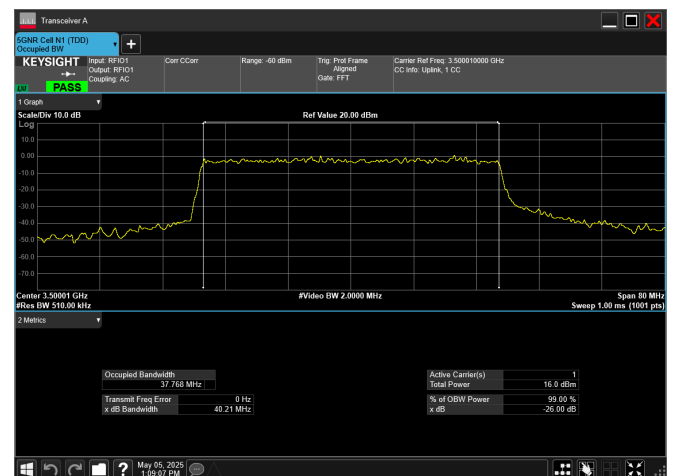
n77_1_40MHz_30kHz_3500MHz_CP-OFDM 256 QAM_RB106@0
