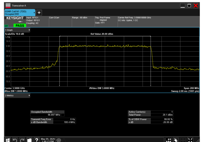
n77_1_100MHz_30kHz_3500MHz_CP-OFDM 256 QAM_RB273@0
