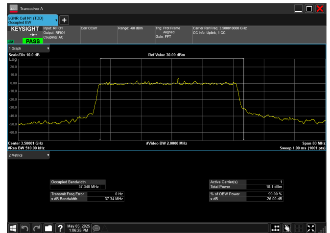
n77_1_40MHz_30kHz_3500MHz_CP-OFDM 16 QAM_RB106@0
