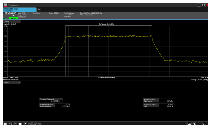
n77_1_10MHz_30kHz_3500MHz_CP-OFDM 16 QAM_RB24@0
