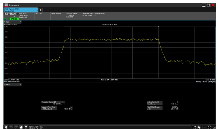
n77_1_20MHz_30kHz_3500MHz_CP-OFDM 256 QAM_RB51@0
