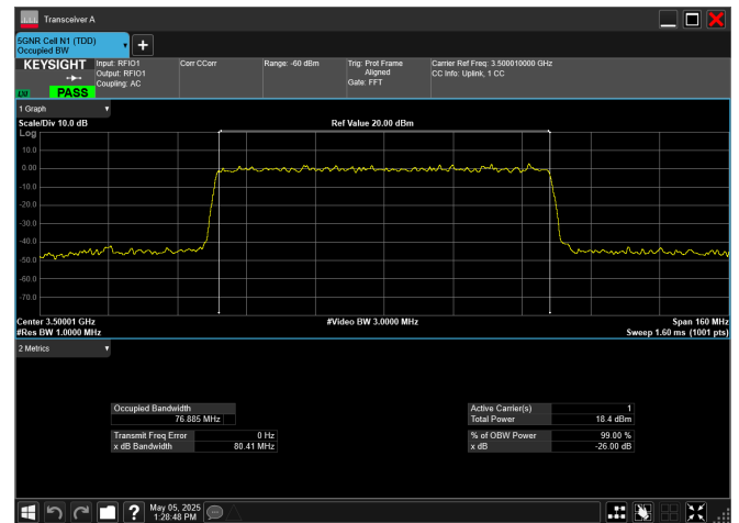
n77_1_80MHz_30kHz_3500MHz_CP-OFDM 16 QAM_RB217@0
