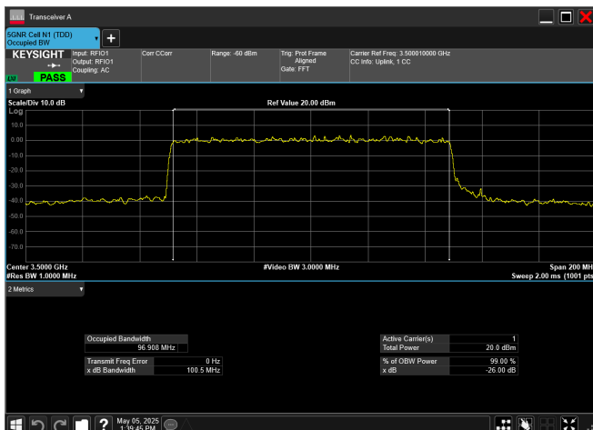
n77_1_100MHz_30kHz_3500MHz_CP-OFDM 64 QAM_RB273@0
