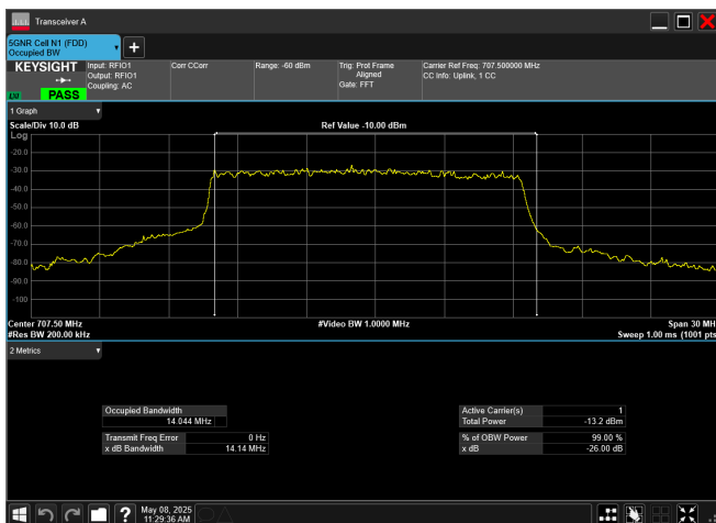
n12_15MHz_15kHz_707.5MHz_DFT-s-OFDM 256 QAM_RB75@0
