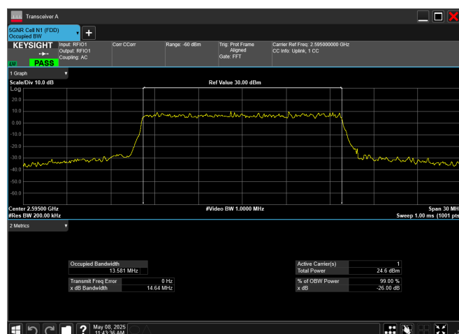
n38_15MHz_30kHz_2595MHz_CP-OFDM 256 QAM_RB38@0
