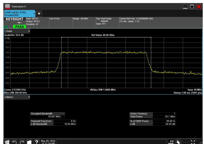
n7_20MHz_15kHz_2535MHz_DFT-s-OFDM 16 QAM_RB100@0
