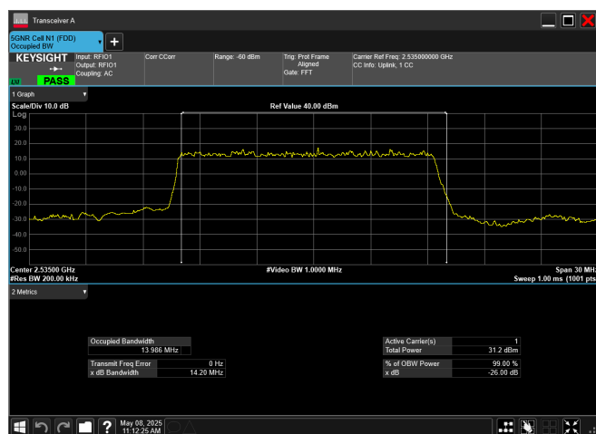
n7_15MHz_15kHz_2535MHz_DFT-s-OFDM 16 QAM_RB75@0
