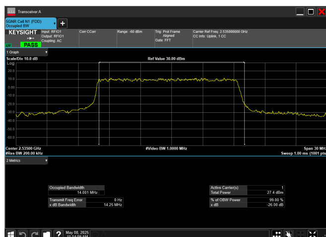
n7_15MHz_15kHz_2535MHz_DFT-s-OFDM 256 QAM_RB75@0
