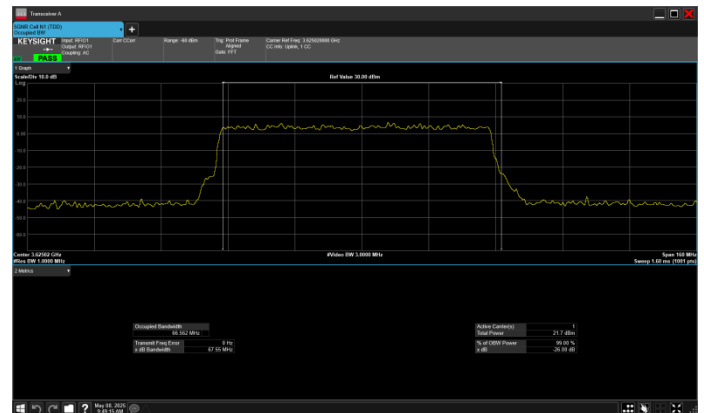
n78_2_70MHz_30kHz_3625MHz_DFT-s-OFDM 64 QAM_RB180@0
