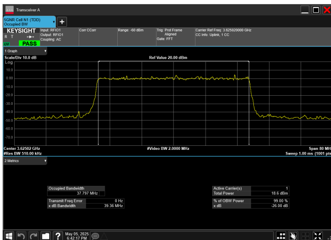
n78_2_40MHz_30kHz_3625MHz_CP-OFDM 64 QAM_RB106@0
