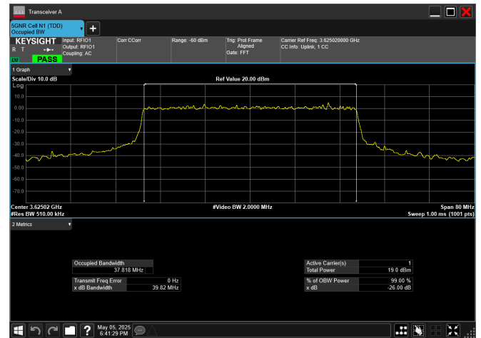
n78_2_40MHz_30kHz_3625MHz_CP-OFDM 256 QAM_RB106@0
