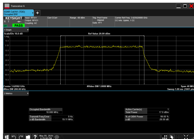
n78_2_20MHz_30kHz_3625MHz_CP-OFDM 16 QAM_RB51@0
