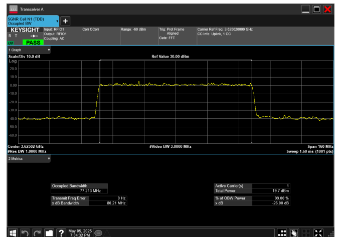
n78_2_80MHz_30kHz_3625MHz_CP-OFDM 256 QAM_RB217@0
