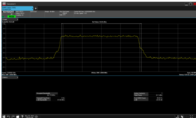
n78_2_70MHz_30kHz_3625MHz_DFT-s-OFDM 16 QAM_RB180@0
