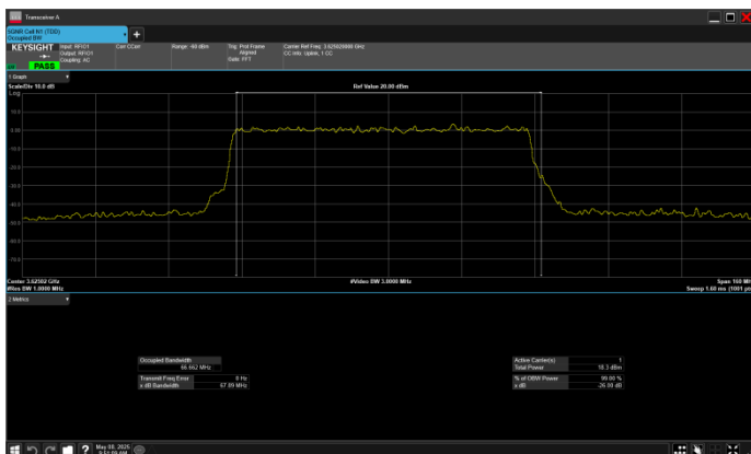
n78_2_70MHz_30kHz_3625MHz_DFT-s-OFDM 256 QAM_RB180@0
