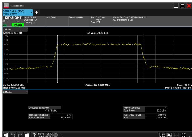
n78_2_50MHz_30kHz_3625MHz_DFT-s-OFDM 256 QAM_RB128@0
