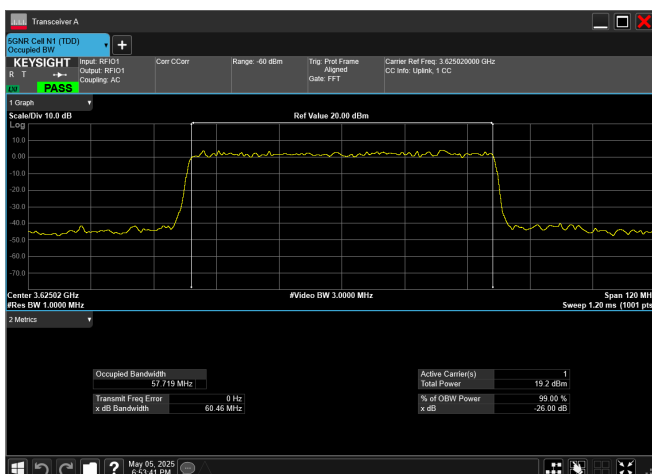
n78_2_60MHz_30kHz_3625MHz_CP-OFDM 64 QAM_RB162@0
