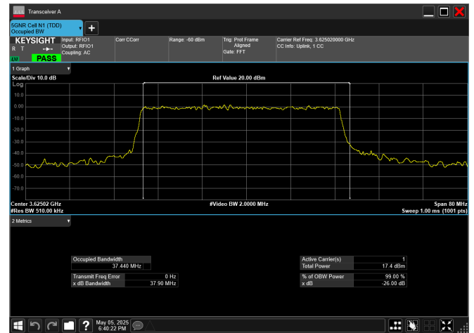
n78_2_40MHz_30kHz_3625MHz_CP-OFDM 16 QAM_RB106@0
