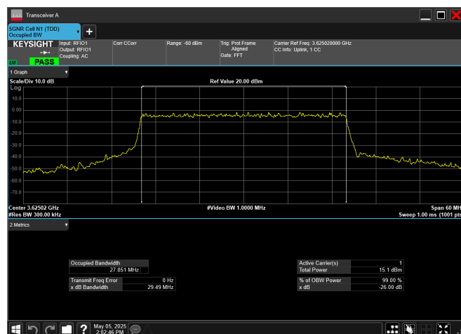
n77_2_30MHz_30kHz_3625MHz_CP-OFDM 256 QAM_RB78@0
