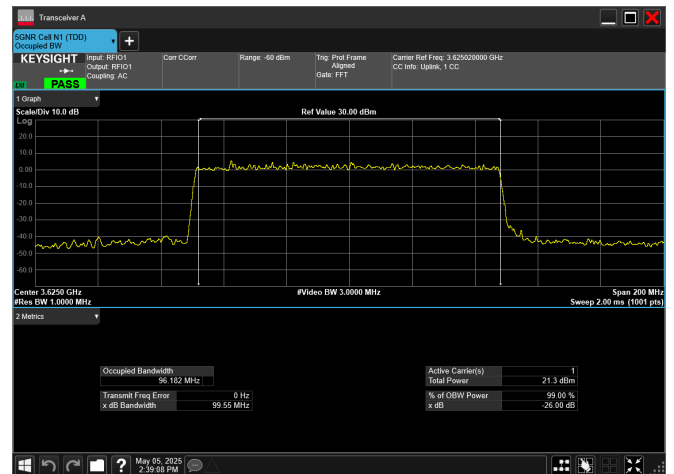
n77_2_100MHz_30kHz_3625MHz_DFT-s-OFDM 64 QAM_RB270@0
