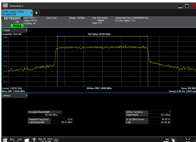
n77_2_100MHz_30kHz_3625MHz_DFT-s-OFDM 256 QAM_RB270@0
