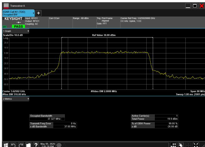
n77_2_40MHz_30kHz_3625MHz_DFT-s-OFDM 256 QAM_RB100@0
