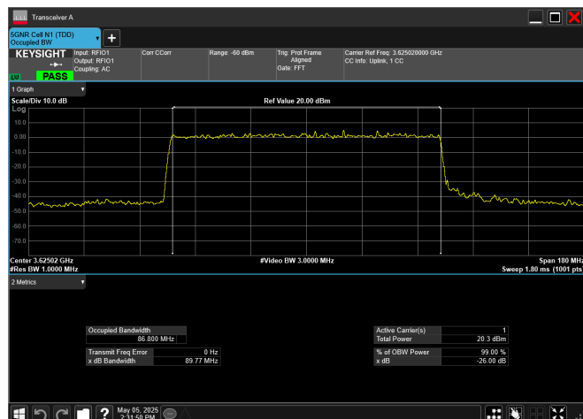
n77_2_90MHz_30kHz_3625MHz_DFT-s-OFDM 16 QAM_RB243@0
