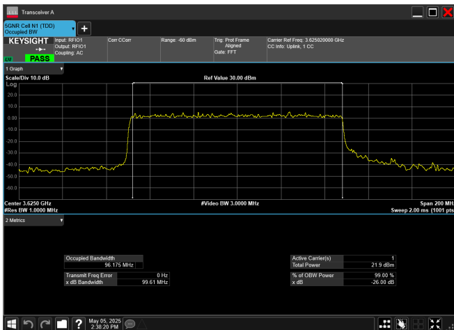
n77_2_100MHz_30kHz_3625MHz_DFT-s-OFDM 16 QAM_RB270@0
