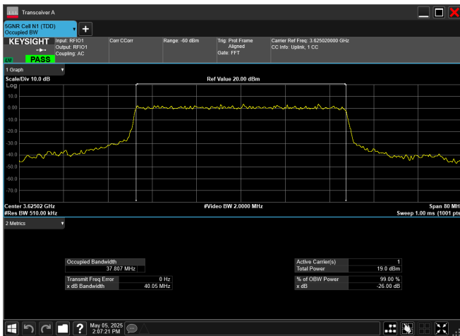
n77_2_40MHz_30kHz_3625MHz_CP-OFDM 256 QAM_RB106@0
