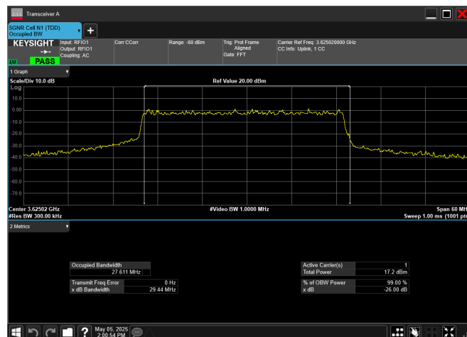
n77_2_30MHz_30kHz_3625MHz_CP-OFDM 16 QAM_RB78@0
