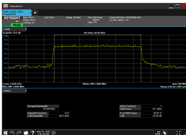
n77_2_100MHz_30kHz_3625MHz_CP-OFDM 256 QAM_RB273@0
