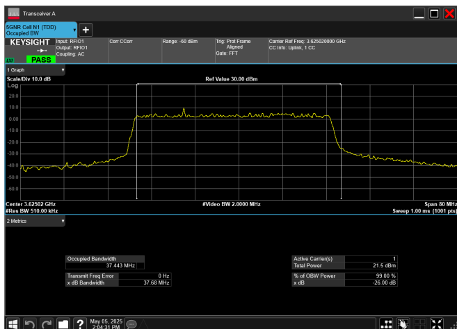
n77_2_40MHz_30kHz_3625MHz_DFT-s-OFDM 16 QAM_RB100@0
