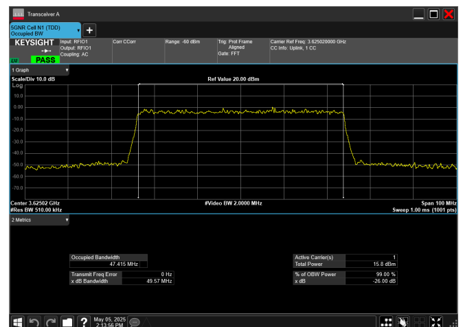
n77_2_50MHz_30kHz_3625MHz_CP-OFDM 256 QAM_RB133@0
