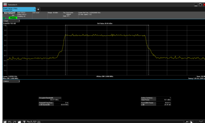
n77_2_70MHz_30kHz_3625MHz_CP-OFDM 16 QAM_RB189@0
