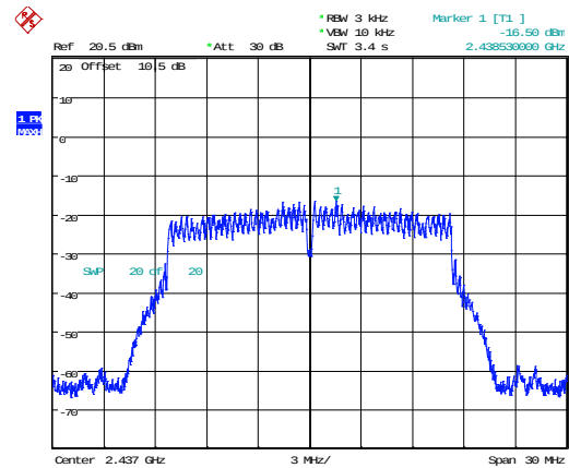
802.11g_2437MHz_Chain 0
