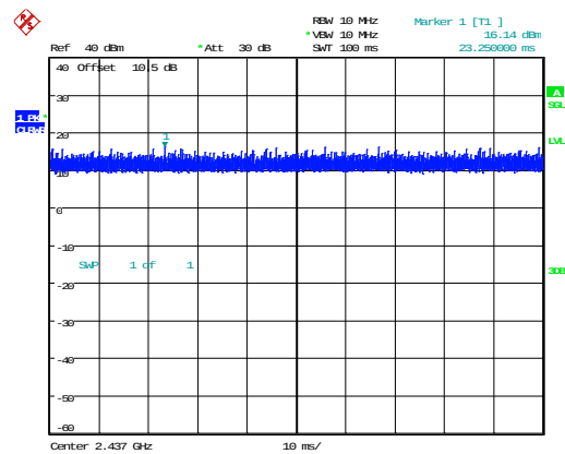
802.11g_2437MHz_Chain 0
