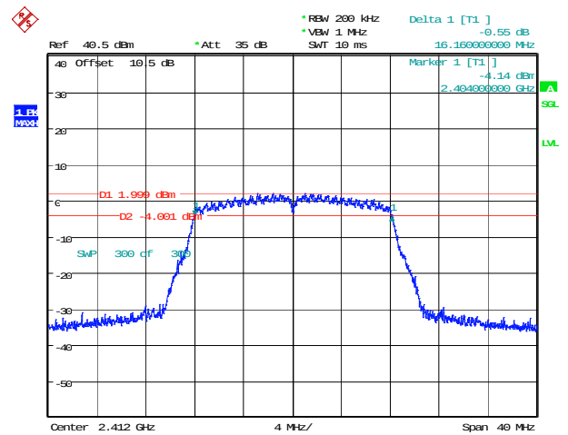
802.11g_2412MHz_Chain 1
