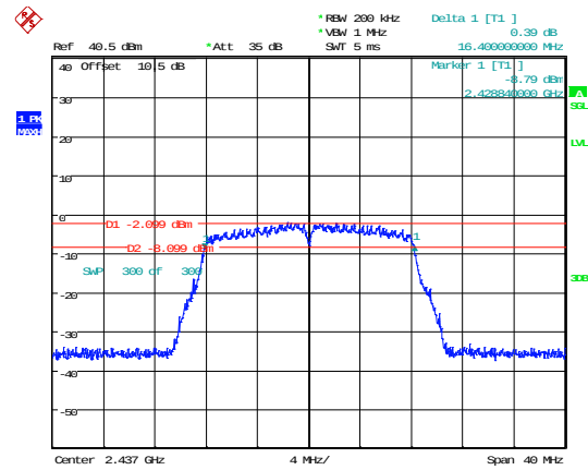
802.11g_2437MHz_Chain 0
