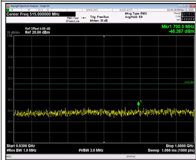
Band38-5MHz-64QAM-38000-1RB#0-Range1:30~1000MHz
