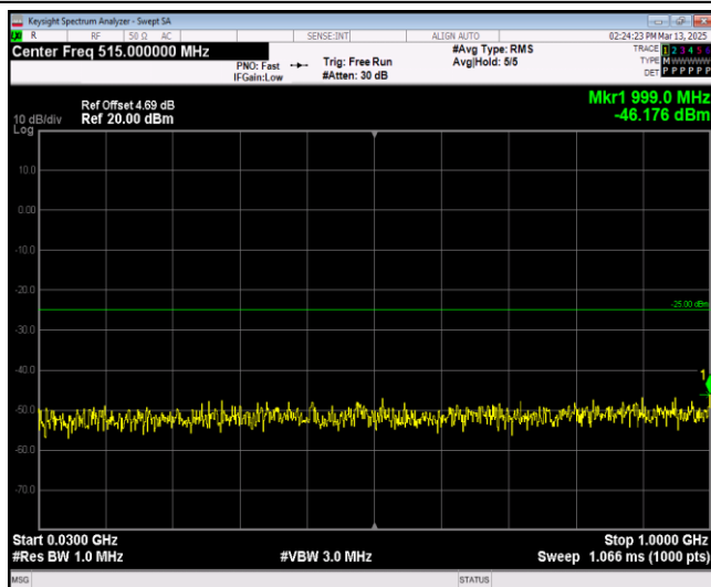
Band38-5MHz-QPSK-37775-1RB#0-Range1:30~1000MHz
