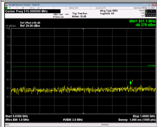
Band38-5MHz-64QAM-38000-1RB#0-Range1:30~1000MHz
