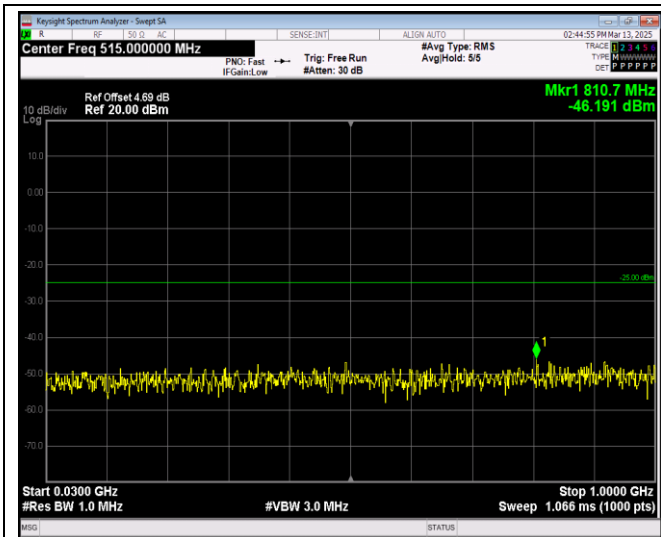
Band38-5MHz-64QAM-37775-1RB#0-Range1:30~1000MHz
