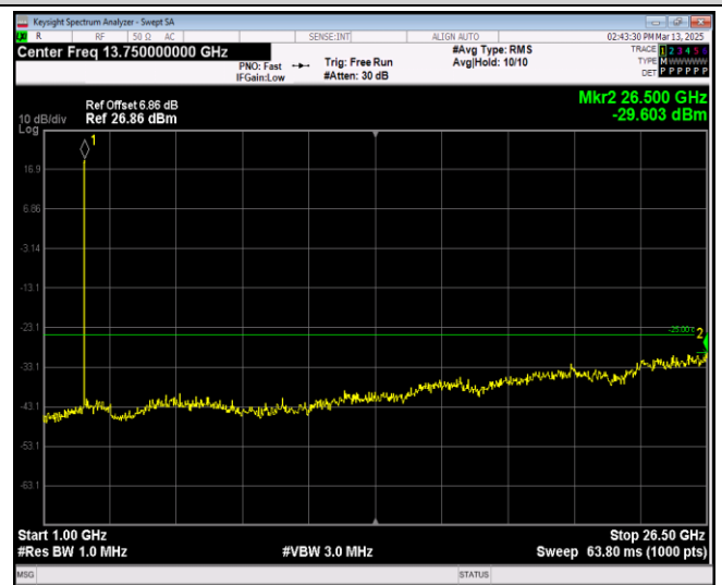
Band38-5MHz-64QAM-38000-1RB#0-Range2:1000~26500MHz
